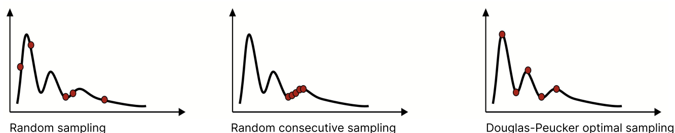
Figure 2. Sketch of the different sampling strategies, fully random, random consecutive, optimal sampling using the Douglas-Peucker algorithm.
