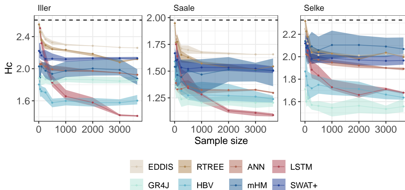
Figure 3. Learning curve using the continuous random sampling strategy for the different models and catchments, conditional entropy, H_c . The lower the values of H_c , the more the model could learn from the data (i.e., the better discharge simulations are). The band of the learning curves are the 25th and 75th percentile of the ensemble of 30 repetitions, the line is the median. The dashed line shows the maximum possible entropy. Note that for visibility reasons we applied a different y-axis scaling for each catchment.
