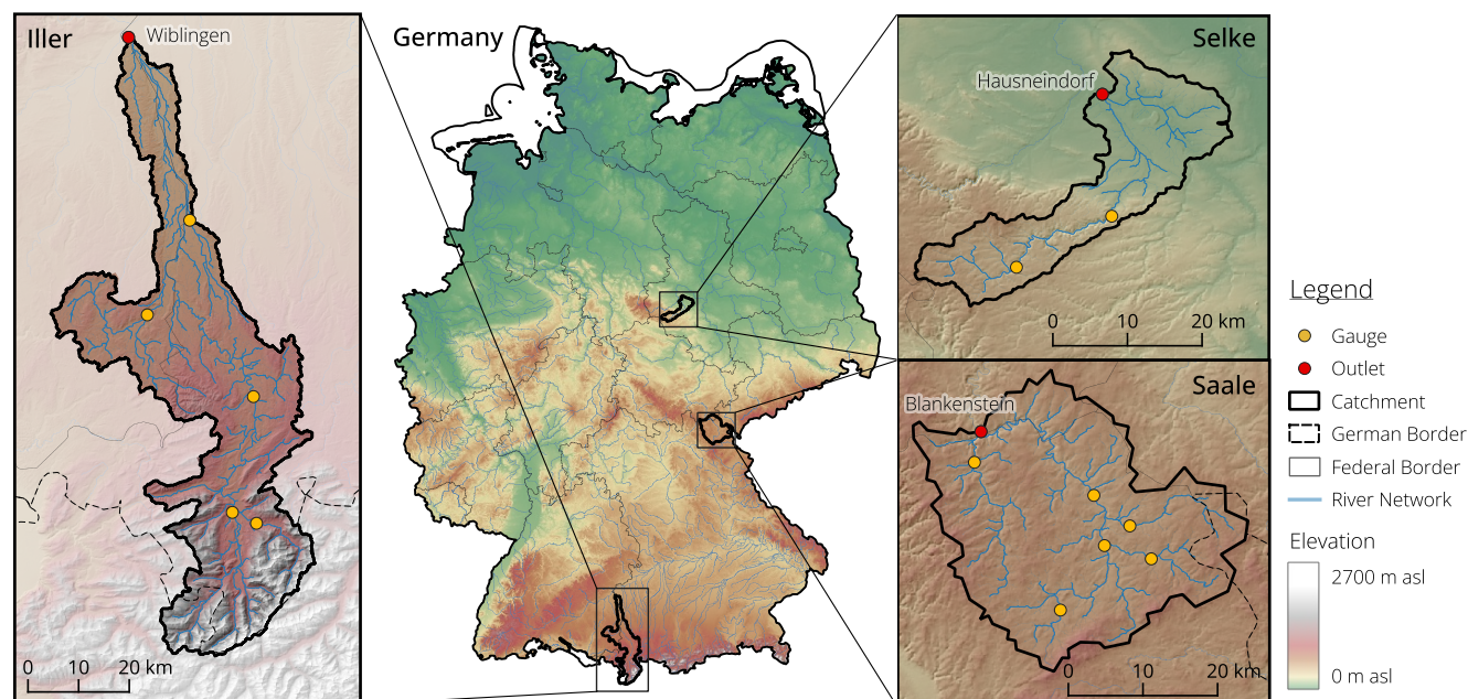
Figure 1. Geographic location, topography and gauging location of the sub-basins of the study catchments.
