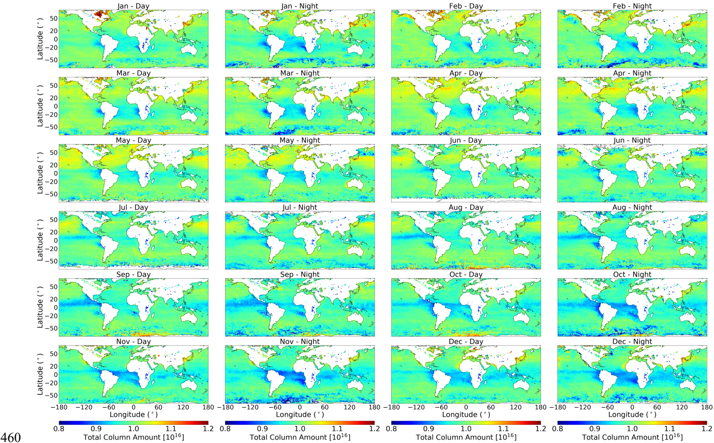
Figure 8 Monthly OCS SOCE total column in units of molecules \text{cm}^{-2} . Day and night are presented for each month of 2018, in 1^\circ \times 1^\circ bins. 2 months are presented on each row, with day and night split into separate columns.
