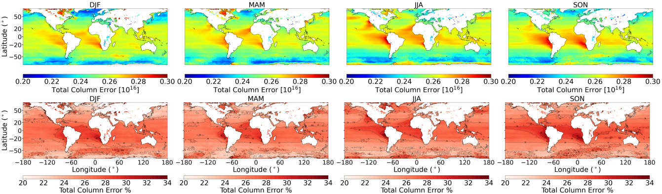
Figure 7. Seasonal mean OCS SOCE posterior error in units of molecules cm -2 (top), for 2018, in 1°×1° bins. Percentage error relative to the total column amount is shown in the bottom row and the columns indicate DJF, MAM, JJA and SON respectively.
