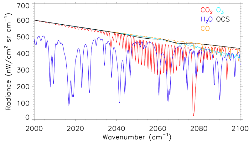
240 Figure 1. Modelled top-of-atmosphere radiances ( \text{nW cm}^{-2} \text{ sr cm}^{-1} ) showing absorption contribution from all five species in the full range considered for OCS microwindow selection: 2000\text{--}2100 \text{ cm}^{-1} , for a pixel in the Indian Ocean ( 0.05^\circ\text{S} , 67.6^\circ\text{E} ) on the 18 th July 2018. A spectral sampling of 0.25 \text{ cm}^{-1} was used.
