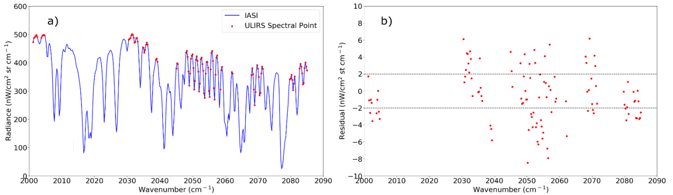
245 Figure 2. a) IASI-B measurement spectra (blue), overlaid with ULIRS spectral points (red) and b) ULIRS OCS retrieval residual spectra (red) for a test pixel over the Indian Ocean on the 18 th July 2018: ( 0.05^\circ\text{S} , 67.6^\circ\text{E} ). Mean residual = 2.59 \text{ nW cm}^{-2} \text{ sr cm}^{-1} . The grey lines indicate the \pm 2 \text{ nW} noise estimate for this spectral region.
