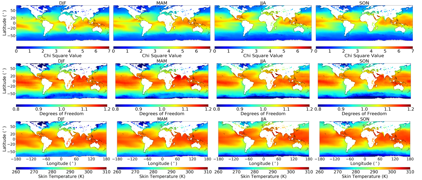
Figure 5. Top row shows \chi^2 , middle row shows mean DOFS, bottom row shows sea surface skin temperature (K). All rows are seasonal (identified in the title) and combine both day and night OCS SoE retrievals from 2018, in 1^\circ \times 1^\circ bins.
