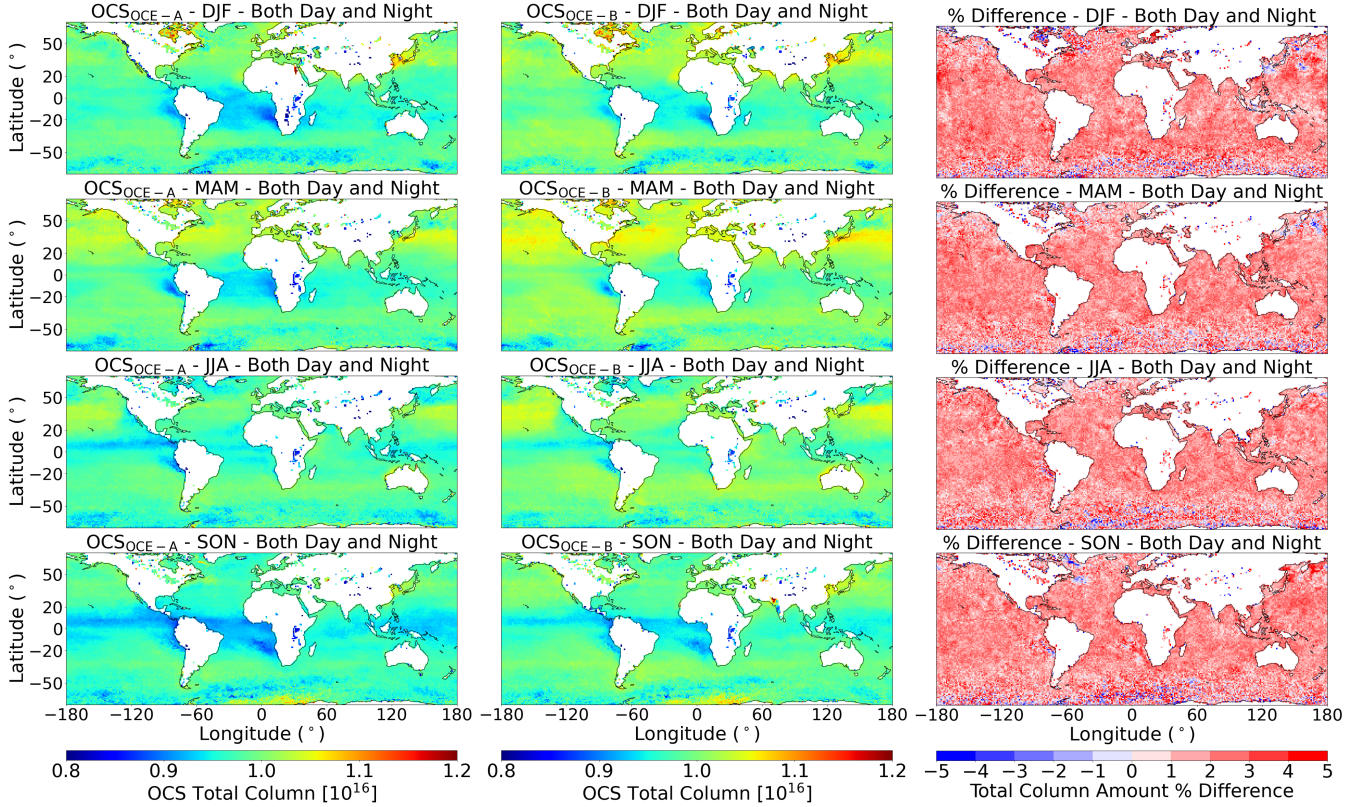
Figure 10. Seasonal estimates of total column OCS mean values in units of molecules \text{cm}^{-2} , for 2018, in 1^\circ \times 1^\circ bins. Left: \text{OCS}_{\text{OCE-A}} estimates, middle: \text{OCS}_{\text{OCE-B}} estimates, right: the % difference between \text{OCS}_{\text{OCE-A}} and \text{OCS}_{\text{OCE-B}} . Daytime and nighttime retrievals are combined.
