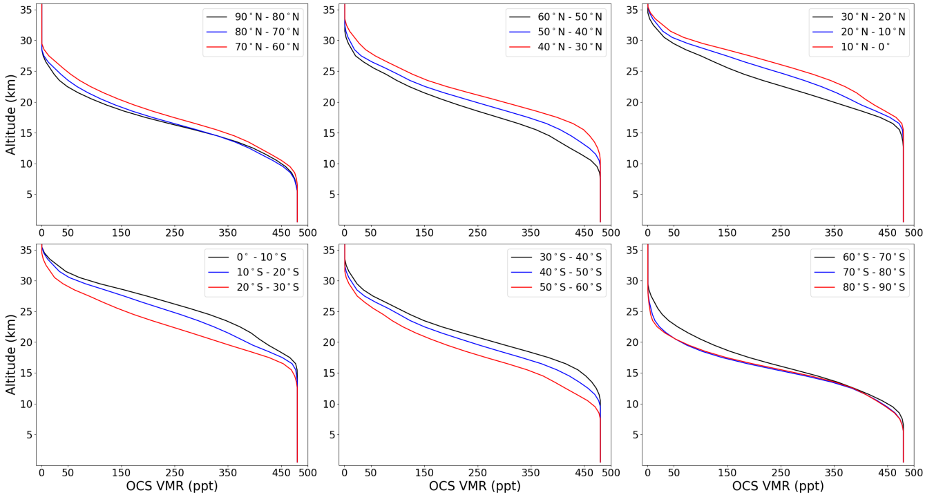
Figure 3. ULIRS a priori profiles of OCS (ppt) derived from ACE-FTS OCS averaged between 2004 and 2020 in 10° latitude bins, stitched to a tropospheric concentration of 480 ppt and an upper stratospheric value of 1 ppt.
