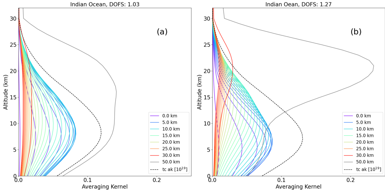
Figure 4. Averaging kernels (AKs) for each level of the ULIRS OCS retrieval grid for pixels over the Indian Ocean, illustrating (a) the minimum DOFS case (4.0°S, 66.8°E; DOFS = 1.03) and (b) the maximum DOFS case (0.15°S, 64.1°E; DOFS = 1.27). Coloured lines represent AKs at different retrieval grid levels; only every 5th level is labelled in the legend (e.g., “0.0 km” = surface, “5.0 km” = 5 km altitude level). The grey line indicated the top level (50 km), and the black dashed line shows the total column averaging kernel (tc_ak, units: molecules cm -2 /ppm). Pixels were selected from daytime pixels for the period between 9th and 26th July 2018, from OCS OCE-B measurements.
