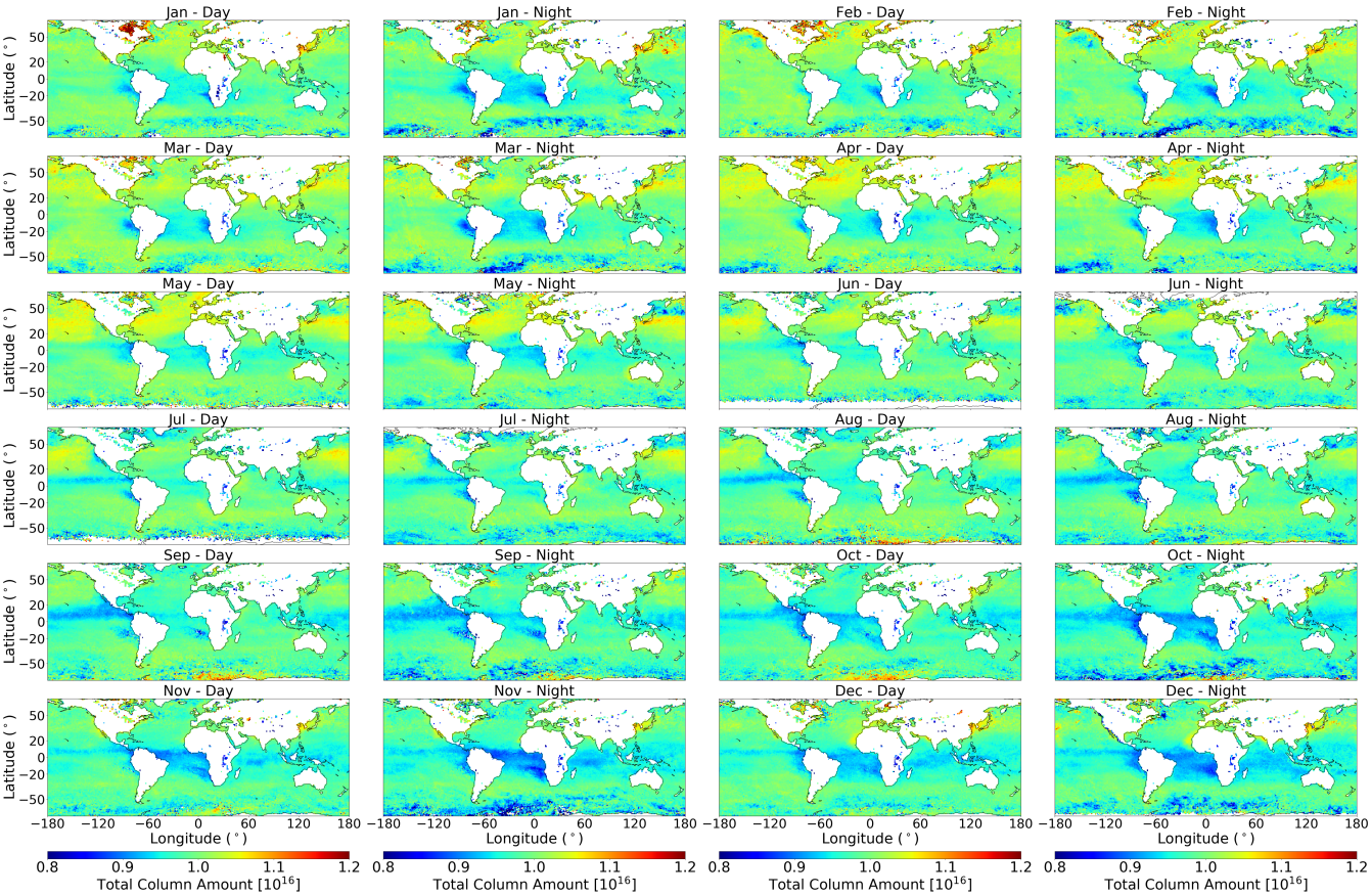
460 Figure 8 Monthly OCS SOCE total column in units of molecules \text{cm}^{-2} . Day and night are presented for each month of 2018, in 1^\circ \times 1^\circ bins. 2 months are presented on each row, with day and night split into separate columns.
