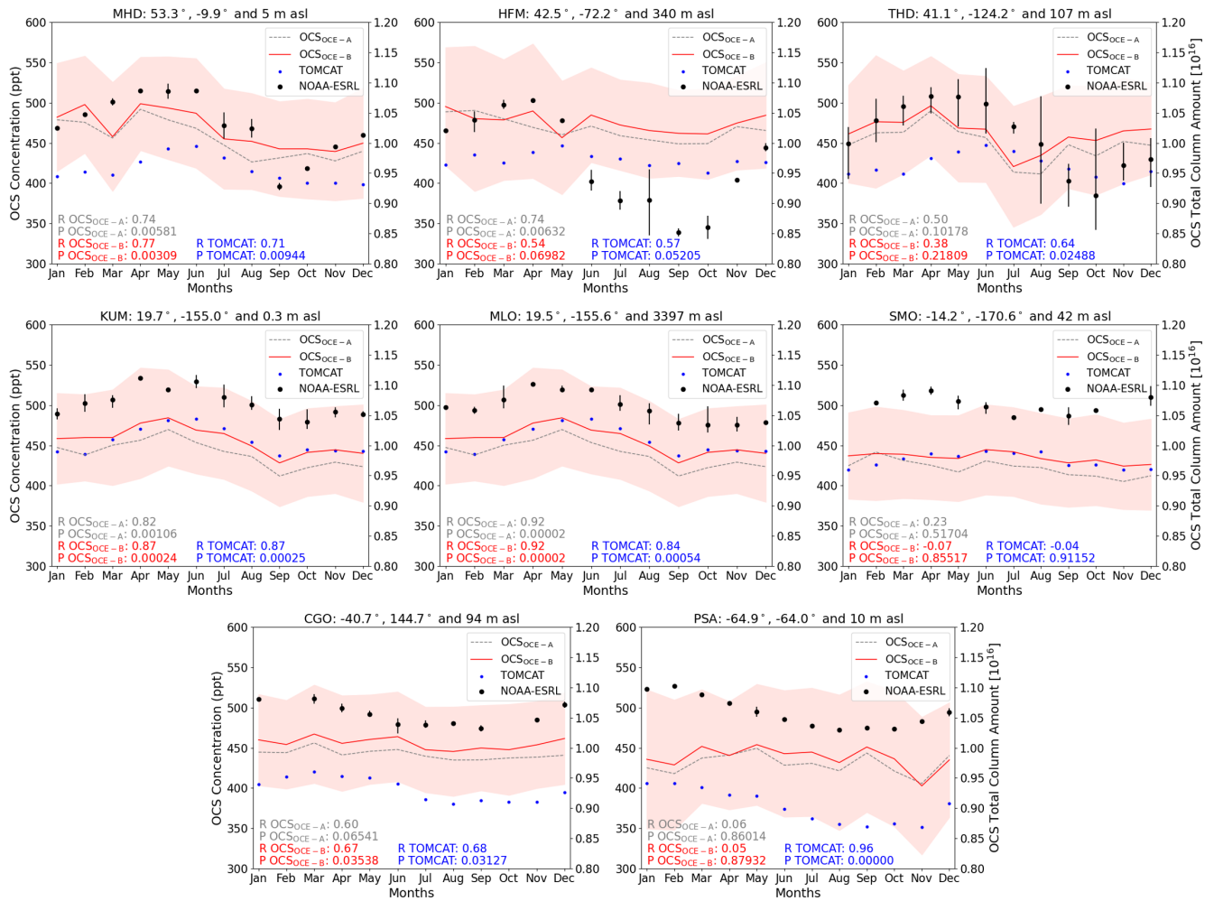
560 Figure 12. NOAA-ESRL surface flask monthly mean observations for 2018 (ppt, black circles) – left axis, are compared with OCS OCE-A (grey dashed), OCS OCE-B (red) and TOMCAT (blue) total column amounts (molecules \text{cm}^{-2} ) – right axis, for the same year. The shaded region represents standard deviation in OCS OCE-B . Note the TOMCAT OCS total columns do not have IASI AKs applied and the statistical comparison is with NOAA-ESRL. All columns in the nearest TOMCAT 2.8^\circ \times 2.8^\circ grid box to the respective surface observations is used in the calculation of the monthly mean OCS OCE-A , OCS OCE-B and TOMCAT columns. Missing NOAA-ESRL points are due to missing data. 565 Linear regression calculations of R represent the Pearson correlation coefficient and of P, the test for statistical significance in the relationship.
