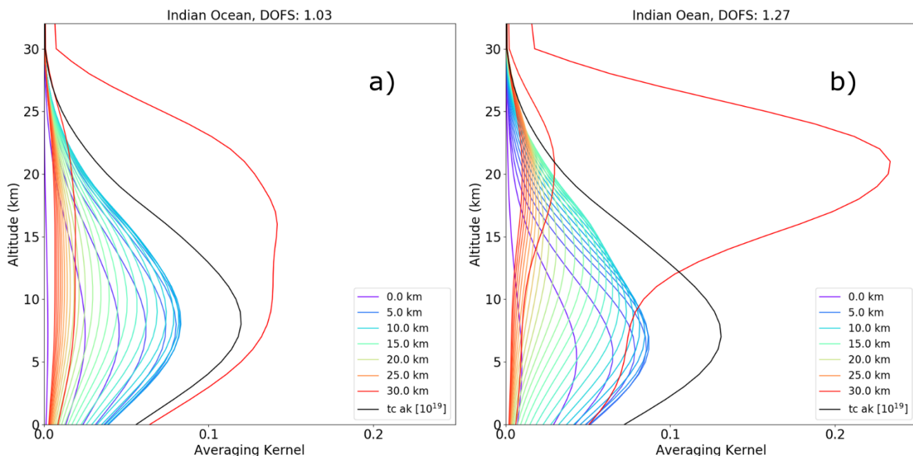
325 Figure 4. Averaging kernels for each level of the ULIRS OCS retrieval grid (solid-coloured lines), the total column AK (units: (molecules cm 2 )/ppm) for minimum DOFS (left) and maximum DOFS (right) scenarios for pixels over the Indian Ocean. DOFS values for each pixel are shown in the titles. (a) Indian Ocean minimum DOFS: 4.0°S, 66.8°E and (b) Indian Ocean maximum DOFS: 0.15°S, 64.1°E. These pixels were selected from the period between 9th and 26th July 2018, from OCS OCE-B measurements.
