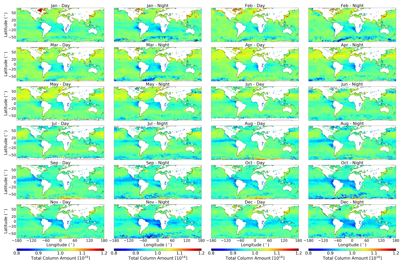
Figure 8 Monthly OCS OCE total column in units of molecules cm -2 . Day and night are presented for each month of 2018, in 1°×1° bins. 2 months are presented on each row, with day and night split into separate columns.
