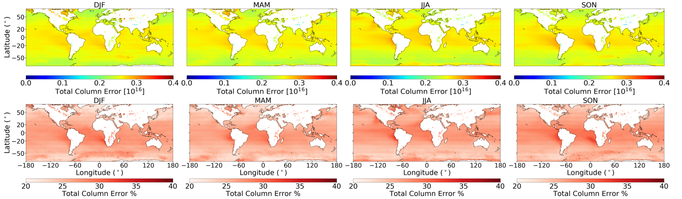
Figure 7. Seasonal mean \text{OCS}_{\text{OCE}} posterior error in units of molecules \text{cm}^{-2} (top), for 2018, in 1^\circ \times 1^\circ bins. Percentage error relative to the total column amount is shown in the bottom row and the columns indicate DJF, MAM, JJA and SON respectively.
