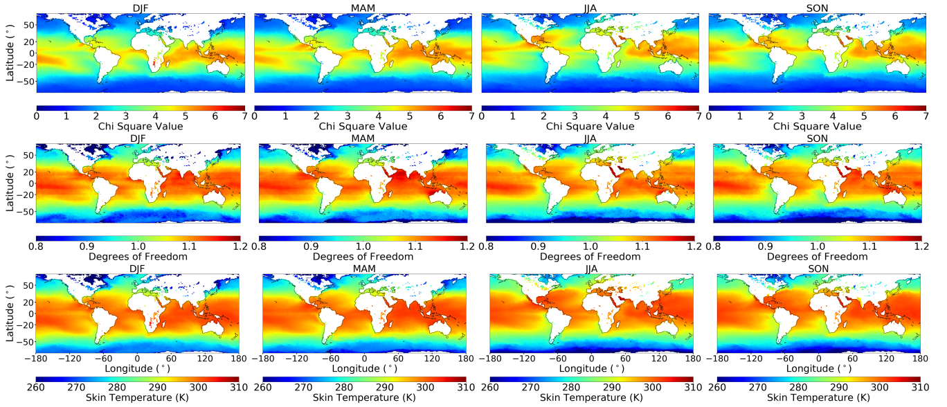
Figure 5. Top row shows \chi^2 , middle row shows mean DOFS, bottom row shows sea surface skin temperature (K). All rows are seasonal (identified in the title) and combine both day and night OCS OCF retrievals from 2018, in 1^\circ \times 1^\circ bins.
