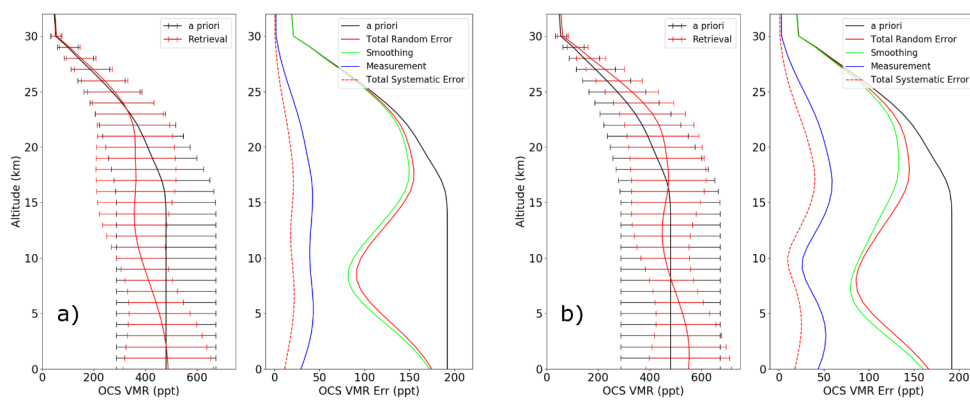
Figure 6. Profiles of retrieved and a priori OCS (left) and profiles of error components (right) for (a) minimum DOFS case and (b) maximum DOFS (b). The 2 pixels selected correspond to Figure 4, where (a) Indian Ocean minimum DOFS: 4.0°S, 66.8°E and (b) Indian Ocean maximum DOFS: 0.15°S, 64.1°W.
