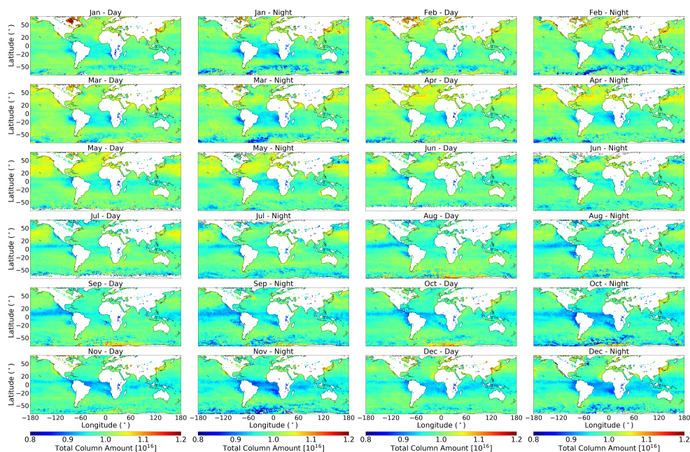
Figure 8 Monthly OCS OCE total column in units of molecules cm -2 . Day and night are presented for each month of 2018, in 1°×1° bins. 2 months are presented on each row, with day and night split into separate columns.
