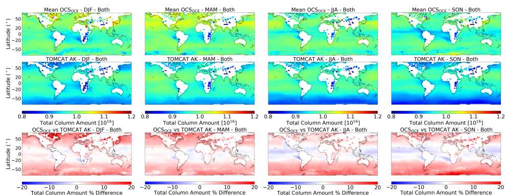
Figure 11. 1 st row: seasonal estimates of total column OCS OCE mean values in units of molecules cm -2 , for 2018, in 1°×1° bins. 2 nd row: TOMCAT OCS with OCS OCE AK applied and 3 rd row: the % difference with OCS OCE .
