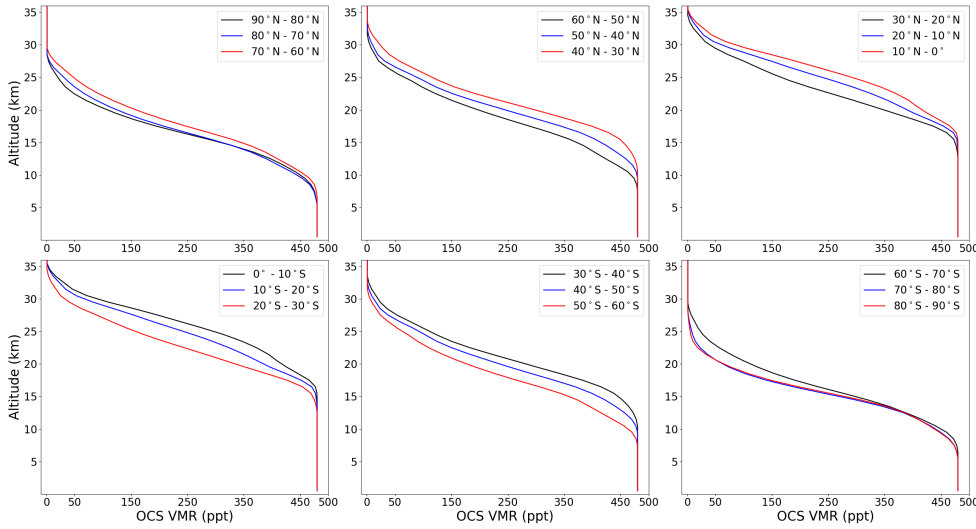
Figure 3. ULIRS a priori profiles of OCS (ppt) derived from ACE-FTS OCS averaged between 2004 and 2020 in 10^\circ latitude bins, stitched to a tropospheric concentration of 480 ppt and an upper stratospheric value of 1 ppt.
