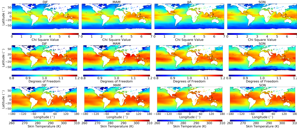
Figure 5. Top row shows \chi^2 , middle row shows mean DOFS, bottom row shows sea surface skin temperature (K). All rows are seasonal (identified in the title) and combine both day and night OCS oce retrievals from 2018, in 1^\circ \times 1^\circ bins.
