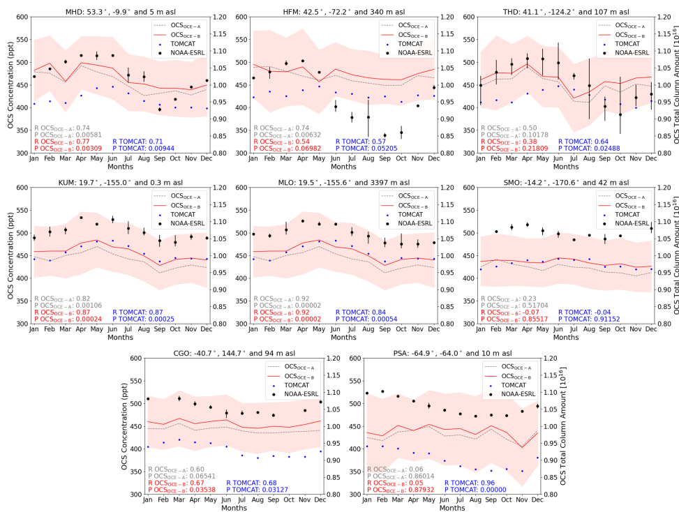
590 Figure 12. NOAA-ESRL surface flask monthly mean observations for 2018 (ppt, black circles) – left axis, are compared with OCS OCE-A (grey dashed), OCS OCE-B (red) and TOMCAT (blue) total column amounts (molecules cm -2 ) – right axis, for the same year. The shaded region represents standard deviation in OCS OCE-B . Note the TOMCAT OCS total columns do not have IASI AKs applied and the statistical comparison is with NOAA-ESRL. All columns in the nearest TOMCAT 2.8°×2.8° grid box to the respective surface observations is used in the calculation of the monthly mean OCS OCE-A , OCS OCE-B and TOMCAT columns. Missing NOAA-ESRL points are due to missing data. 595 Linear regression calculations of R represent the Pearson correlation coefficient and of P, the test for statistical significance in the relationship.
