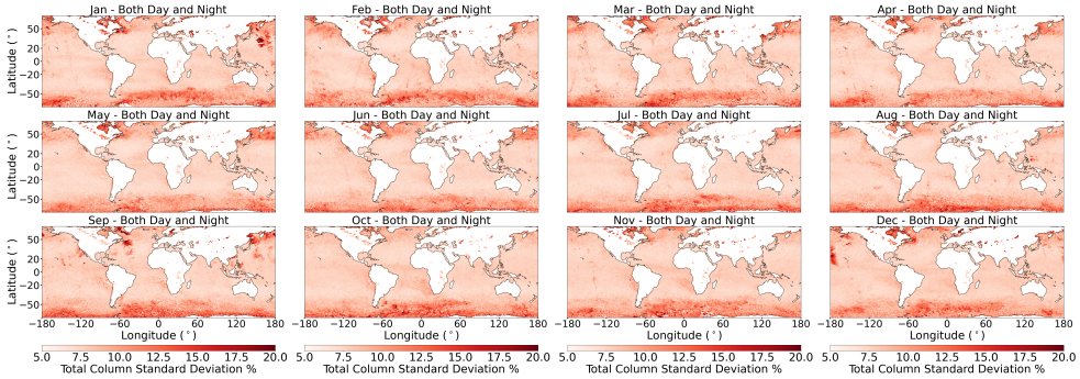
495 Figure 9. Monthly standard deviation (%) of total column OCS mean values for 2018. Day and night are combined for each month, in 1^{\circ} \times 1^{\circ} bins.
