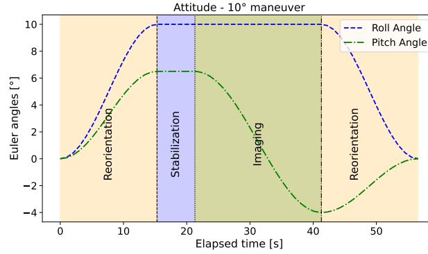
Figure 3. Schematic Illustration of TANGO’s dynamic maneuverability using roll and pitch adjustments during an observational cycle. The plot represents a 10° roll maneuver, showing key stages of satellite operation: reorientation, stabilization, and imaging.
