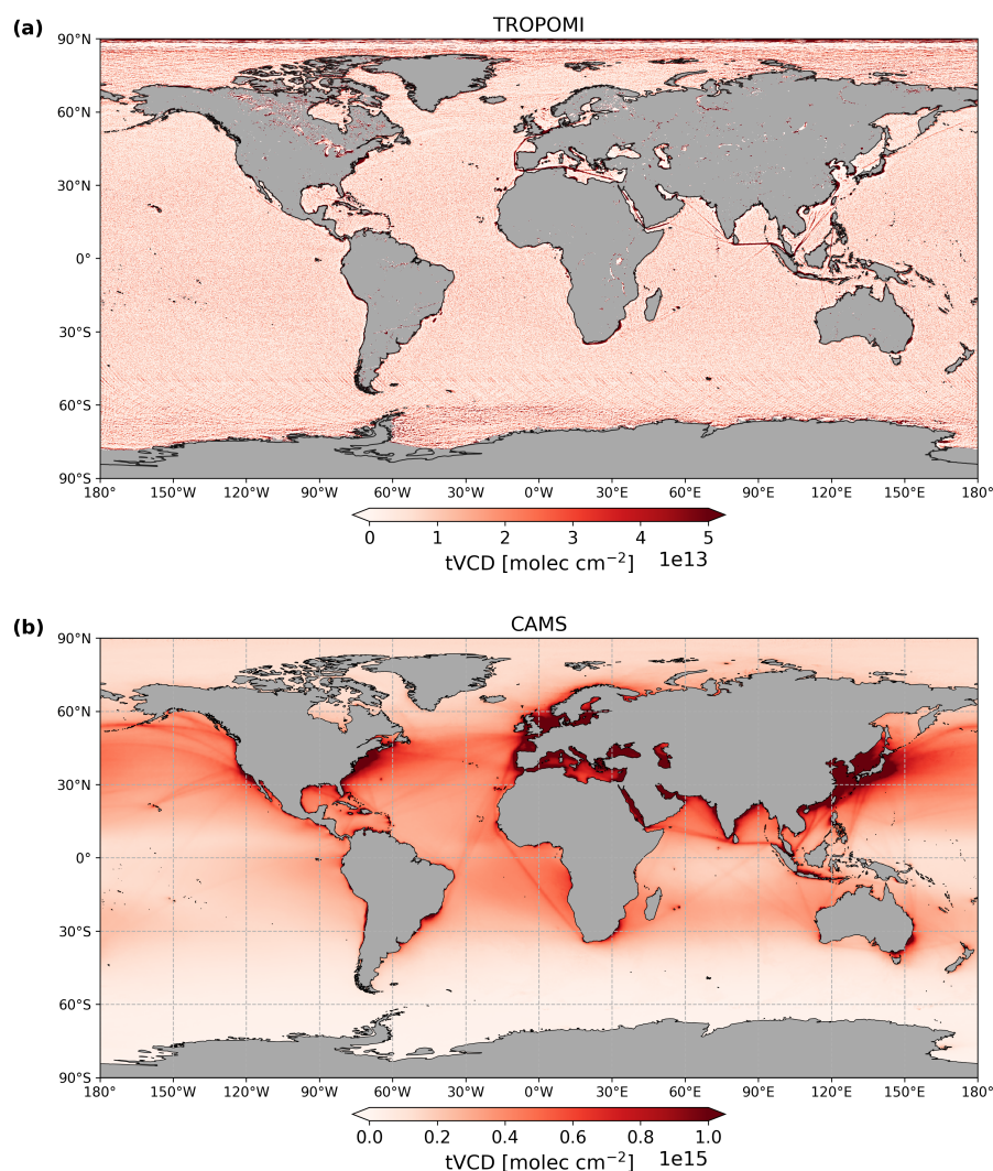
Figure C1. On a global scale, the magnitude of (a) the filtered TROPOMI NO 2 tVCDs is, on average, at least a factor of 10 smaller than the magnitude of (b) the CAMS NO 2 tVCDs. Additionally, differences are found in the spatial extent of the shipping lanes, resulting from the coarser resolution of the CAMS model data, which are retrieved on a 0.4^\circ \times 0.4^\circ grid from 2019 to 2023 with cloud flagging. However, the positions of a great number of shipping routes, visible in the CAMS data, are identified in the filtered TROPOMI NO 2 data. In addition, the CAMS model data show a higher NO 2 signal in the Ross Sea near the Antarctic continent at a similar position to the filtered TROPOMI data (see also Fig. B1a), which confirms the assumption that this is an actual NO 2 emission signal.
