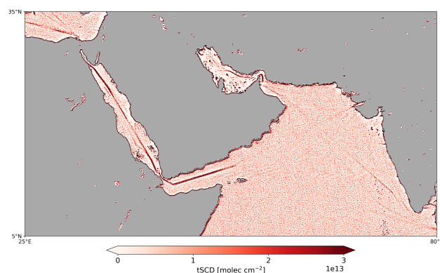
Figure B2. Filtered TROPOMI NO 2 signals from shipping activity in the Red and Arabian Seas with the non-iterative high-pass filtering at a box size of approximately 0.25° in both longitude and latitude. Two separated shipping lanes are visible in the Gulf of Aden. In the Persian Gulf, a distinct shipping route is visible near the coast of Iran, and the dot-shaped elevated NO 2 values indicate NO x emissions from offshore platforms. However, the shipping NO 2 signals in the Arabian Sea are not as pronounced as in the filtered TROPOMI data using the iterative approach with a box size of 1° (see Fig. 4a).
