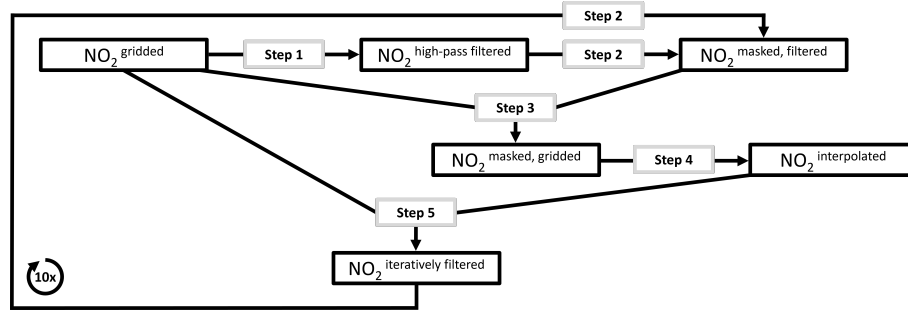
Figure 1. Schematic overview of the iterative high-pass filtering procedure applied on the gridded TROPOMI NO 2 tSCD. After a thorough examination, an iteration number of ten times proves to be the most efficient.
