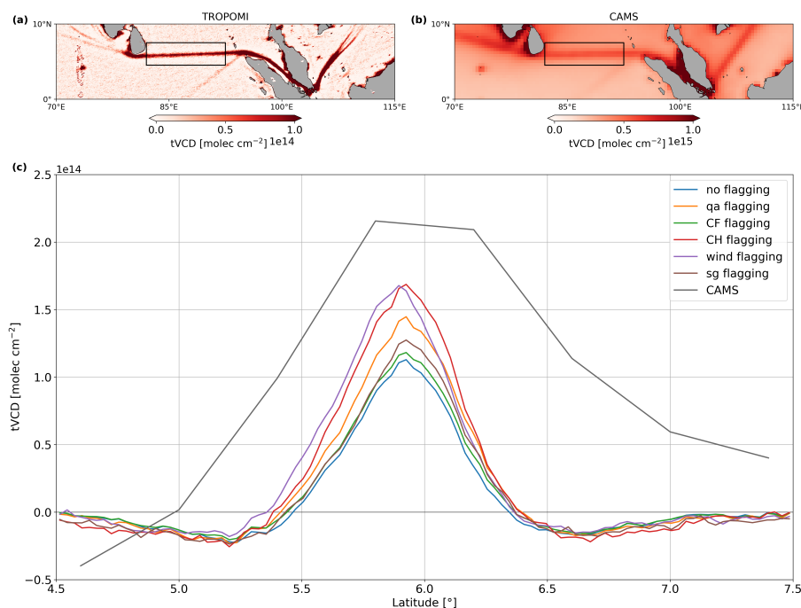
Figure 11. As Fig. 6, but with (a) the filtered TROPOMI NO 2 tVCDs, (b) the CAMS NO 2 tVCDs, and (c) the cross-sections of the shipping lane for the different TROPOMI flagging criteria and the CAMS data, which are offset by a value of 3.5e14 molec cm -2 . The brought-together curves of the data sets show a similar distribution peak, but the area under the CAMS tVCD curve is more extensive than under those of the filtered TROPOMI tVCDs. This broader FWHM in latitude of the CAMS curve results due to the coarser resolution of the CAMS model data, which are retrieved on a 0.4° x 0.4° grid for the years from 2019 to 2023 with cloud flagging.
