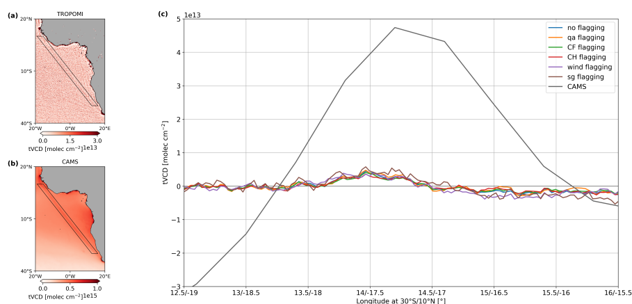
Figure C3. As Fig. C2, but (c) presents the cross-sections of the black polygons of the shipping lane in the South Atlantic Ocean west of the African continent. The CAMS NO 2 tVCDs are offset by a value of 4.5e14 molec cm -2 , and thus, capture the shipping lane with approximately 100 times larger values than the filtered TROPOMI NO 2 tVCDs, which do not exceed 0.5e13 molec cm -2 at the maximum peak. The filtered TROPOMI NO 2 curves vary greatly in this region due to the S5p orbit-oriented structures enhanced by the high-pass filtering, while the CAMS peak is straight-lined due to the coarser resolution. The higher values on the right side of the CAMS curve result from larger signals near the continent, possibly due to emission outflow. In comparison, the smaller values on the left curve side correspond to weaker signals in the open ocean.
