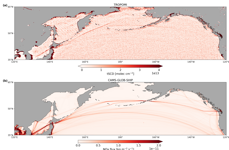
Figure 5. (a) Filtered TROPOMI and (b) CAMS-GLOB-SHIP \text{NO}_2 signals from shipping activity in the North Pacific correlate well for the two shipping routes between Asia and North America. The \text{NO}_2 signal in the Bering Sea is only identified in the filtered TROPOMI data and not tracked through the AIS-based CAMS-GLOB-SHIP data, possibly due to disabled trackers onboard military or unauthorized fishing vessels. The CAMS-GLOB-SHIP data cover the years from 2018 to 2021.
