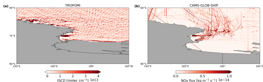
Figure B1. The higher NO 2 signal in the (a) filtered TROPOMI data in the Southern Ocean near the Antarctic continent can be assigned to (b) CAMS-GLOB-SHIP NO 2 shipping activities in the Ross Sea. The CAMS-GLOB-SHIP data cover the years from 2018 to 2021. The enhanced NO 2 signal is detected only in the summer season with minimal sea ice extent, while during winter, the NO 2 signal in the Antarctic region is dominated by sea ice cover, indicating that these NO 2 emissions may originate from ship emissions.
