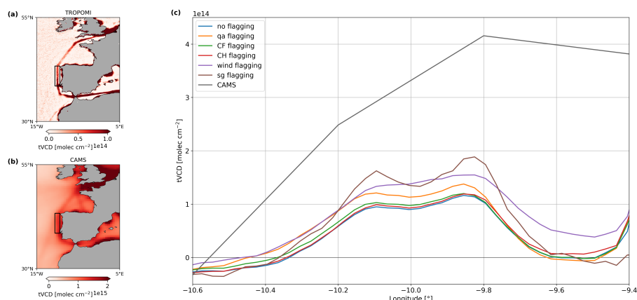
Figure C2. (a) Filtered TROPOMI NO 2 tVCDs, (b) CAMS NO 2 tVCDs, and (c) the cross sections of the shipping lane in the North Atlantic Ocean near the coast of Portugal (black rectangles) for the different TROPOMI flagging criteria and the CAMS data, which are offset by a value of 1e15 molec cm -2 . Besides the at least 20 times larger CAMS NO 2 values compared to the TROPOMI data, the two peak patterns of this small-scale shipping lane are not as clearly identified in the CAMS curve as in the TROPOMI tVCDs due to the coarser resolution of the CAMS model data. In addition, this poor resolution leads to a mixing of shipping signals and emissions from land, here visible in the considerable NO 2 value at -9.4° longitude, which is not clearly set aside from the signal peak at -9.8° longitude.
