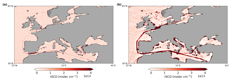
Figure 3. Filtered TROPOMI NO 2 signals from shipping activity in the European seas, analyzed with high-pass filters at different box sizes: approximately (a) 0.25° and (b) 1° in both longitude and latitude. The 0.25° box size reveals details of more minor shipping routes, such as the two shipping lanes in the North Atlantic Ocean, while weaker signals, such as in the Baltic Sea, and NO x emissions from oil and gas platforms in the North Sea (see also Fig. 9), are more visible with the 1° box size. The NO 2 saturation near land, especially visible in the North Sea, around Italy, and at the coast of France, Spain and North Africa in (b), is a result of the iterative high-pass filtering which partially enhances the higher NO 2 signals at coastlines.
