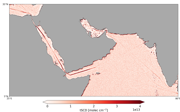
Figure B4. Filtered TROPOMI \text{NO}_2 signals from shipping activity in the Red and Arabian Seas with the non-iterative high-pass filtering at a box size of approximately 0.25^\circ in both longitude and latitude. Two separated shipping lanes are visible in the Gulf of Aden. In the Persian Gulf, a distinct shipping route is visible near the coast of Iran, and the dot-shaped elevated \text{NO}_2 values indicate \text{NO}_x emissions from offshore platforms. However, the shipping \text{NO}_2 signals in the Arabian Sea are not as pronounced as in the filtered TROPOMI data using the iterative approach with a box size of 1^\circ (see Fig. 4a).
