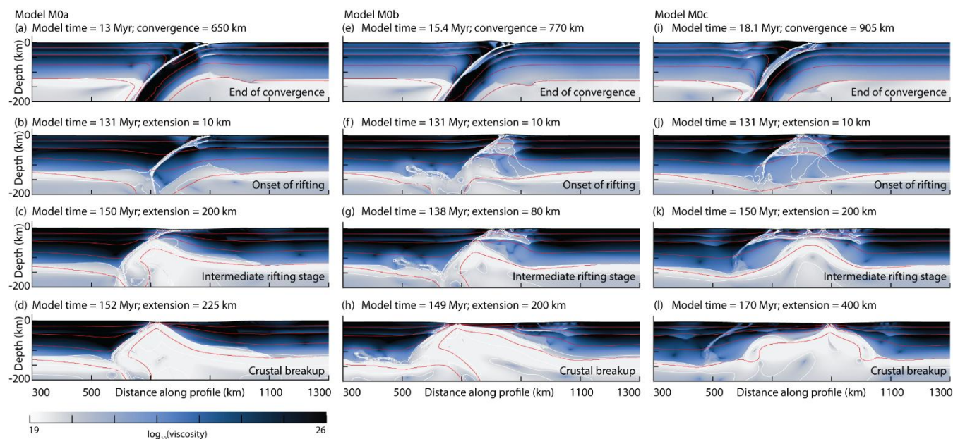
Figure C 2. Viscosity snapshots of the evolution of model experiments M0a (a-d), M0b (e-h), and M0c (i-l). Selected isotherms displayed by red contours (300°C, 600°C, 900°C, and 1300°C) and areas experiencing high strain rates displayed with white contours ( 10^{-13} to 10^{-15} s ^{-1} ).
