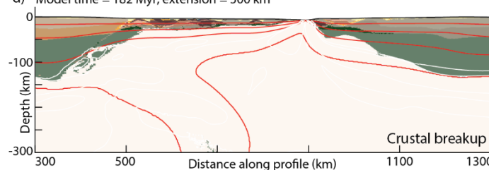
Figure C 1. Model evolution of supplementary model S1. (a-d) SM1 is characterized by an extra-large orogen and slab breakoff below the LAB. During rifting, new normal shear-zones form within the orogen creating wide, asymmetric rifted margins. The style is similar to what is observed in experiments M0c, M1b and M2b.
