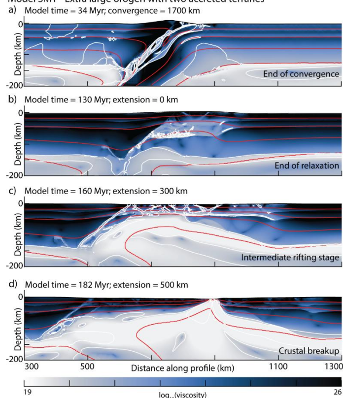
660 Figure C 5. Viscosity snapshots of the evolution of supplementary model experiment SM1 (a-d). Selected isotherms displayed by red contours (300°C, 600°C, 900°C, and 1300°C) and areas experiencing high strain rates displayed with white contours ( 10^{-13} to 10^{-15} s ^{-1} ).
