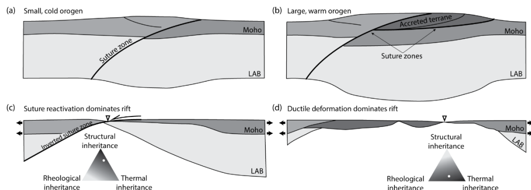
425 Figure 8. Conceptual figure showing the difference in evolution between rifting a small, cold (a, c) and a large, warm (b, d) orogen. Ternary diagrams on (c) and (d) display the estimated relative importance in the rift evolution of the three inheritance types considered in this study.
