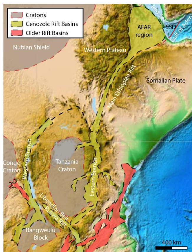
Figure 2. Map of the rheological, structural and thermal inheritance example sights from the East African Rift System. The shapes of cratons and rift basins were drawn after Ali and Watts (2013); Kidane et al. (2003); Kolawole et al. (2021); Rime et al. (2023); Samsu et al. (2023)
