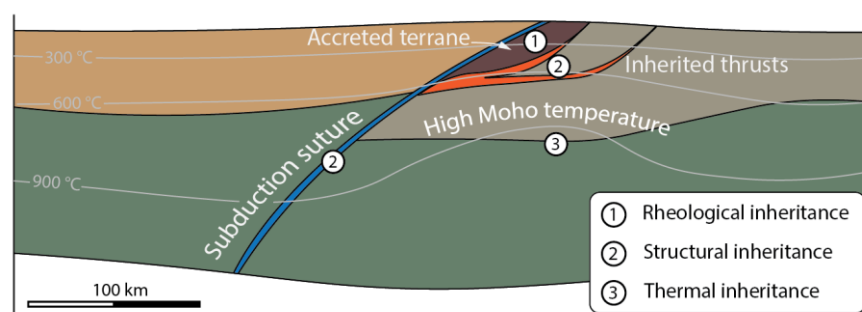
45 Figure 1. A simplified lithospheric-scale cross-section illustrating the different types of orogenic inheritance that can exert a controlling influence on a subsequent phase of continental rifting.
