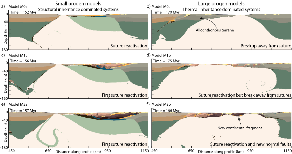
Figure 7. Comparison of the final rifted margins of 6 experiments forming a small size orogen (left column, panels a, c and e) or large size orogen (right column, panels b, d and f) accreting 0 (top row, a and b), 1 (middle row, c and d) or 2 (bottom row, e and f) microcontinents. The comparison demonstrates the strong effect of the pre-rift thermal state of the lithosphere on the degree of suture reactivation and the final geometry of the resulting rifted margins. From a to f the snapshots are from models M0a, M0c, M1a, M1b, M2a and M2b.
