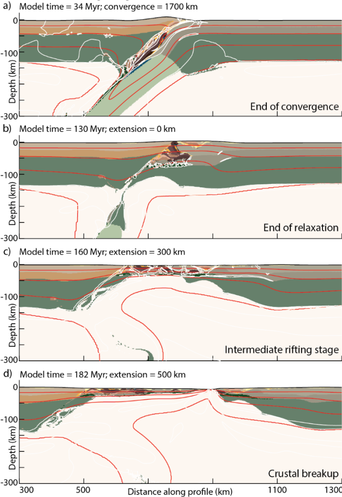
Figure C 1. Model evolution of supplementary model S1. (a-d) SM1 is characterized by an extra-large orogen and slab breakoff below the LAB. During rifting, new normal shear-zones form within the orogen creating wide, asymmetric rifted margins. The style is similar to what is observed in experiments M0c, M1b and M2b.
