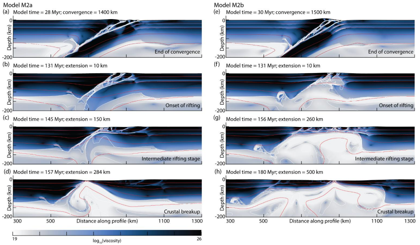
Figure C 4. Viscosity snapshots of the evolution of model experiments M2a (a-d) and M2b (e-h). Selected isotherms displayed by red contours (300°C, 600°C, 900°C, and 1300°C) and areas experiencing high strain rates displayed with white contours ( 10^{-13} to 10^{-15} \text{ s}^{-1} ).
