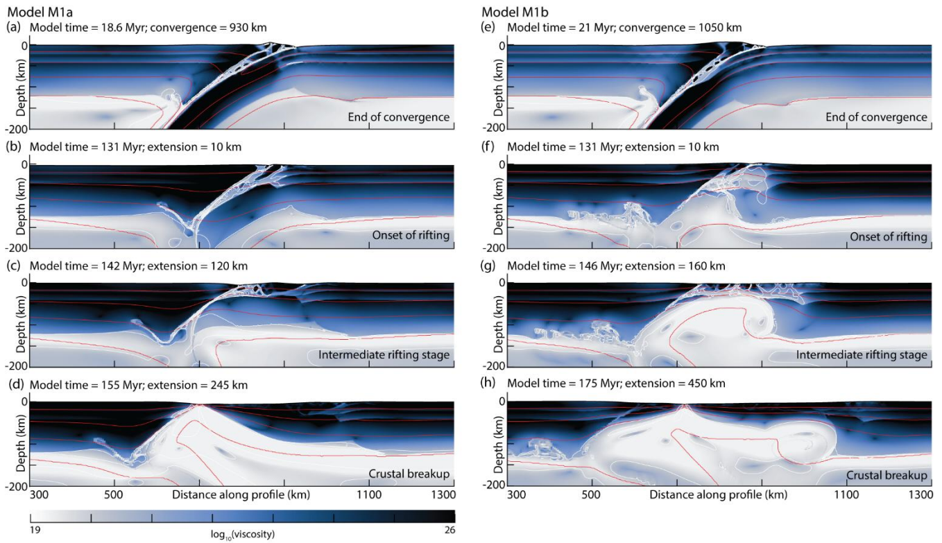
Figure C 3. Viscosity snapshots of the evolution of model experiments M1a (a-d) and M1b (e-h). Selected isotherms displayed by red contours (300°C, 600°C, 900°C, and 1300°C) and areas experiencing high strain rates displayed with white contours ( 10^{-13} to 10^{-15} \text{ s}^{-1} ).
