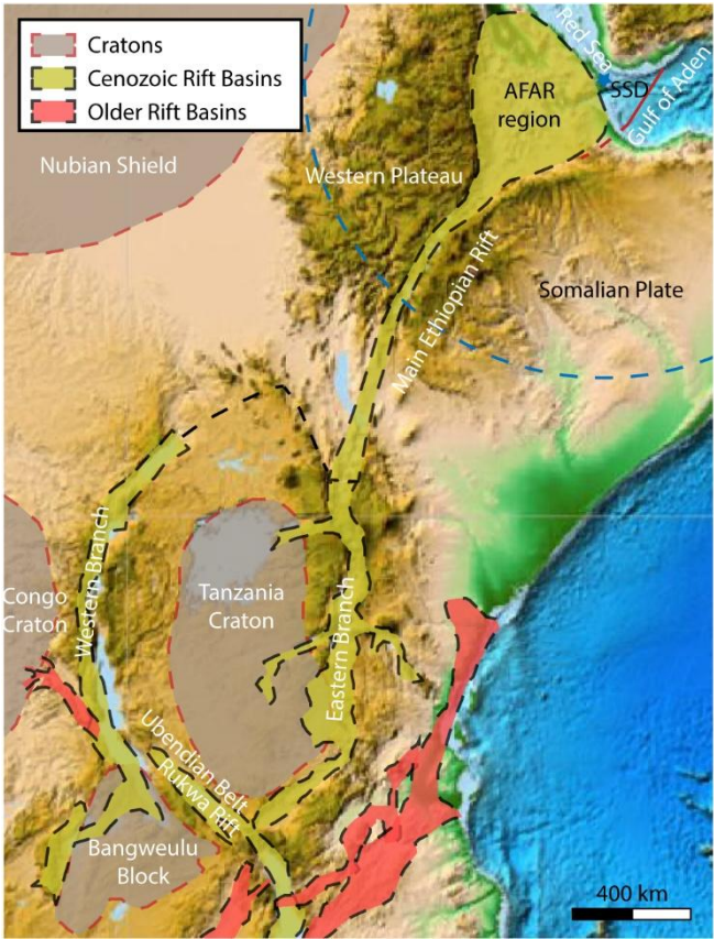
70 Figure 2. Examples of rheological inheritance in the form of Cratons and structural inheritance in the form of Cenozoic and older rift basins from the East African Rift System. The shapes of cratons and rift basins were drawn after Ali and Watts (2013); Kidane et al. (2003); Kolawole et al. (2021); Rime et al. (2023); Samsu et al. (2023). The red line, marked SSD, shows the location of the
