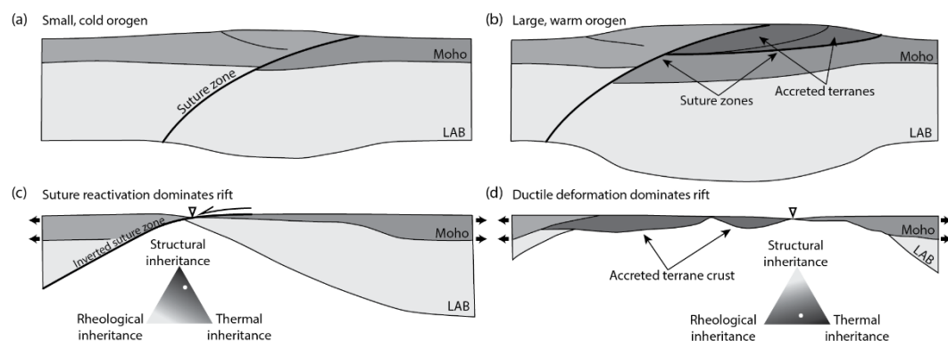
Figure 8. Conceptual figure showing the difference in evolution between rifting a small, cold (a, c) and a large, warm (b, d) orogen. The large, warm orogen displayed here also incorporates accreted terranes (darkest grey material). Ternary diagrams on (c) and 450 (d) display the estimated relative importance in the rift evolution of the three inheritance types considered in this study.
