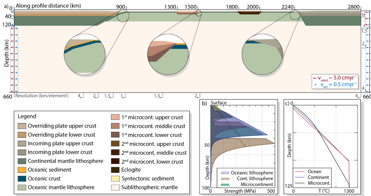
Figure 3. Initial experimental setup before the initiation of convergence, shortening, terrane accretion and orogeny. a) The initial geometry of a model containing two microcontinents with close-ups of the ocean-continent margins and an ocean-microcontinent margin. The black numbers along the vertical domain edges represent distance in kms measured from the top left corner. The light-grey numbers along the edges represent the numerical resolution, measured as element size in kms. The red and blue arrows along the sides represent the velocity boundary conditions in the collision and rifting phases respectively. b) Analytically-calculated strength-profiles of the initial continental lithosphere, the oceanic lithosphere and a microcontinent, with dashed lines showing the strain-weakened profiles. c) Analytical temperature profiles of the oceanic and continental lithospheres as well as the microcontinents used in the strength calculations depicted in b).
