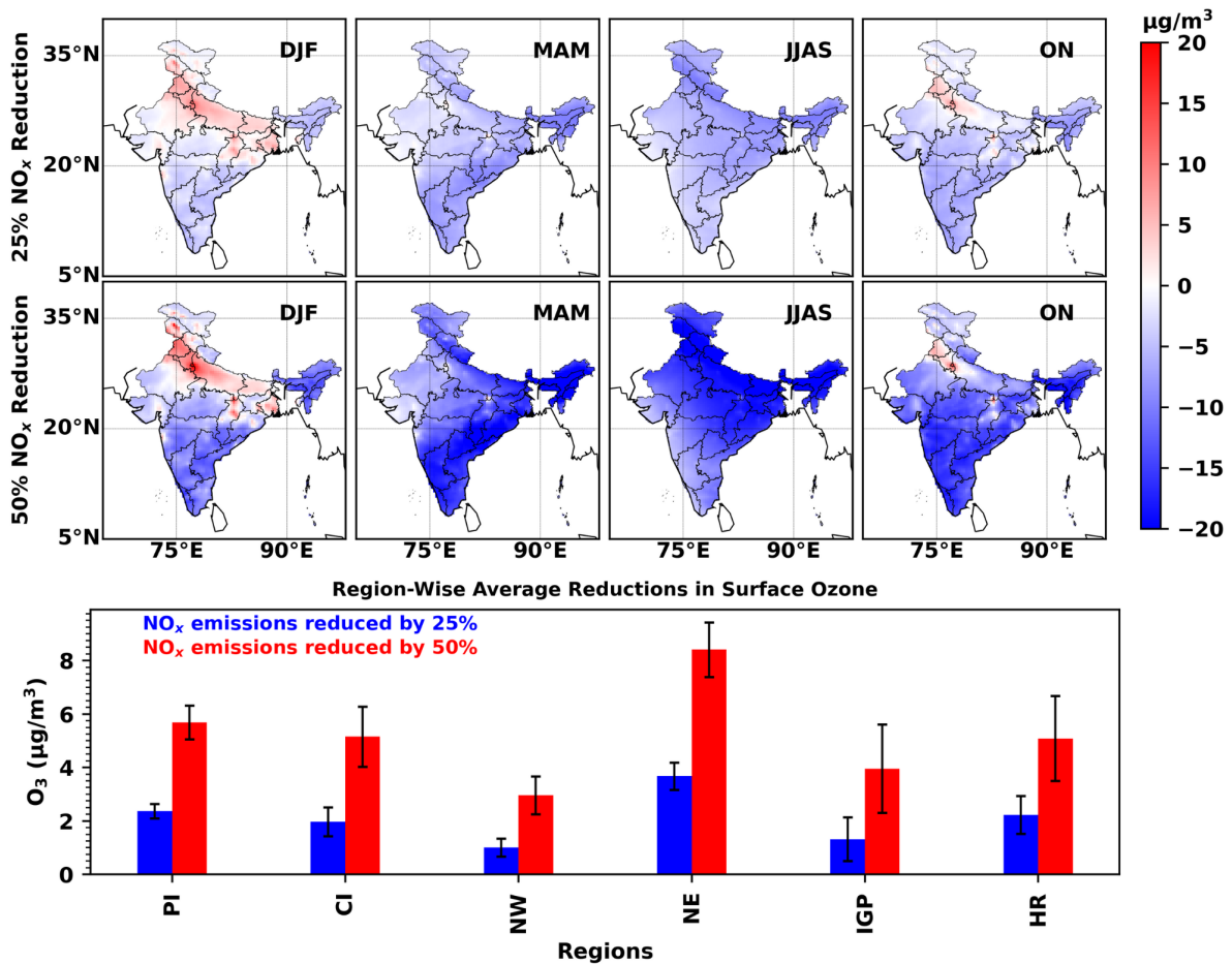
Figure 7: The change in ozone levels when NO x emissions are scaled down by (top) 25% and (middle) 50% when compared to that of base simulation in 2022 with no reduction of emissions. (bottom) Region-wise averaged surface ozone reduction when NO x emissions are scaled down by 25 and 50% for the year 2022. The whiskers represent the standard deviations. Here, DJF is December-January-February, MAM is March-April-May, JJAS is June-July-August-September, ON is October-November, NW is NorthWest, NE is North East India, IGP is Indo-Gangetic Plains and HR is Hilly Regions.
