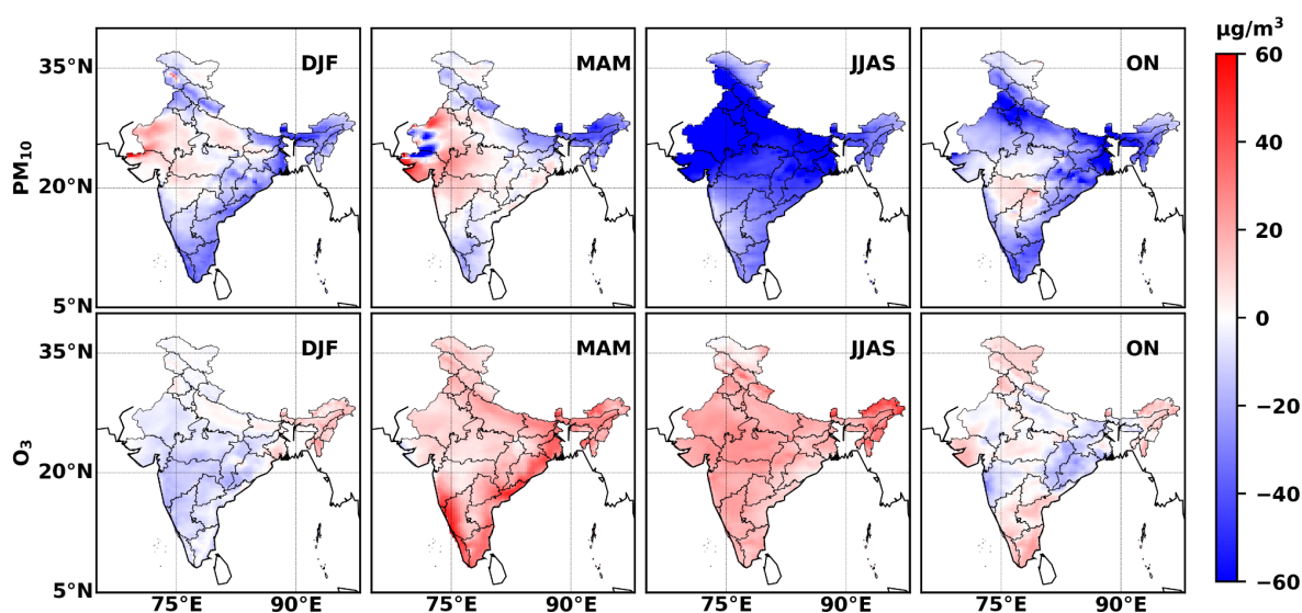
Figure 3: The difference in (Top) PM 10 and (Bottom) Ozone in 2022 when compared to that of 2018. Here, DJF is December-January-February, MAM is March-April-May, JJAS is June-July-August-September and ON is October-November.
