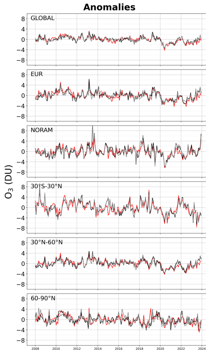
335 Figure 15: Monthly time series of tropospheric ozone anomalies in Dobson units (DU) derived from IASI CDR (red), 340 smoothed (black) and raw (gray) sonde data on the global and regional scales. The tropospheric column is integrated from the surface to the thermal tropopause, as defined by the World Meteorological Organization (WMO, 1957).
