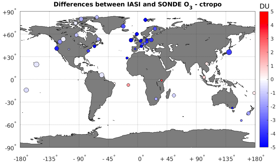
Figure 8: Location of the 43 ozonesonde stations used in this study. The colors represent the mean difference between IASI and sonde tropospheric ozone column in Dobson units (DU) over the period from January 2008 and December 2023. The standard deviation is represented by the size of the circle.
