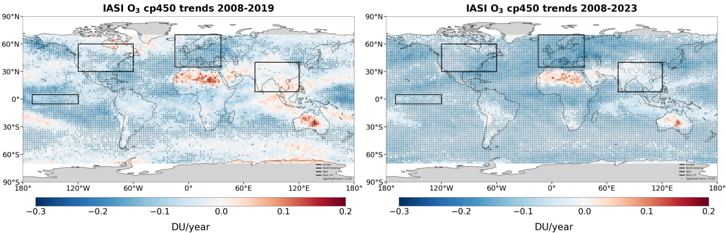
840 Figure D1: Spatial distribution of lower tropospheric ozone (surface-450 hPa) trends (in DU year -1 ) derived from IASI-CDR before the COVID-19 pandemic (2008–2019) and including the pandemic (2008–2023). Dots indicate trends with high to very high certainty (p-value<=0.05). The black rectangles indicate the boundaries of the regions analyzed in Fig. 13.
