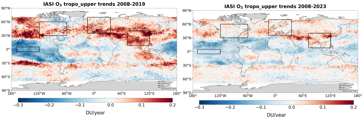
845 Figure D2: Spatial distribution of upper tropospheric ozone (450 hPa-tropopause) trends (in DU per year) derived from IASI-CDR before the COVID-19 pandemic (2008–2019) and including the pandemic (2008–2023). The tropopause altitude is estimated using the WMO thermal definition. Dots indicate trends with high to very high certainty (p-value<=0.05). The black rectangles indicate the boundaries of the regions analyzed in Fig. 13.
