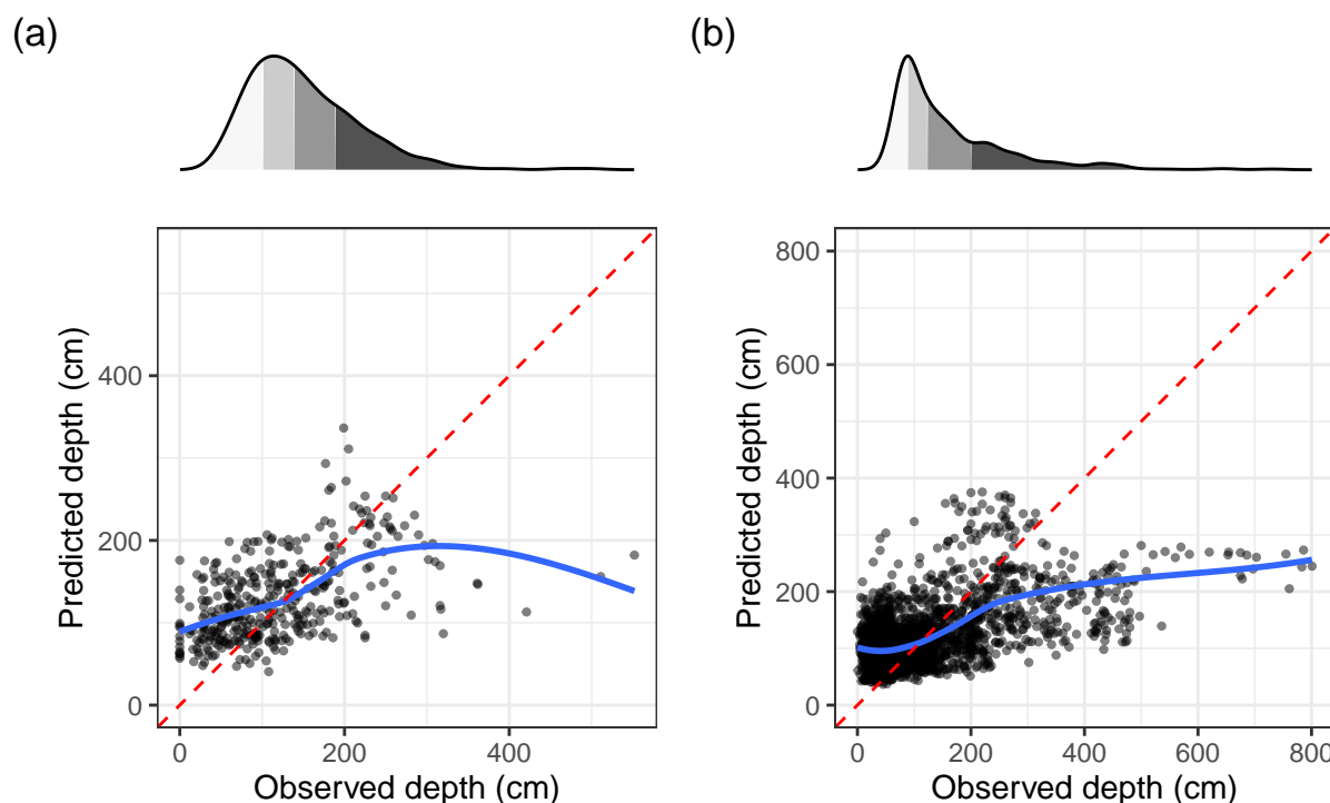
Figure 3. Calibration plots for the best-performing models at Skrimfjella (a) and Ørskogfjellet (b), with predictions from spatial cross-validation. Points are transparent to show overlap. Blue lines are local polynomial regressions and the red dashed line in each panel shows the 1:1 line. Marginal distributions (top) are shaded by quartile.
