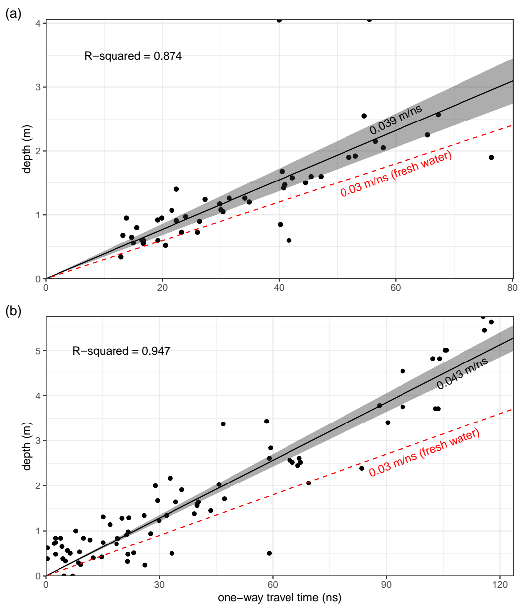
Figure A1. Calibration of GPR wave velocity at Skrimfjella (a) and Ørskogfjellet (b) by regression of probed depth against wave travel time.
