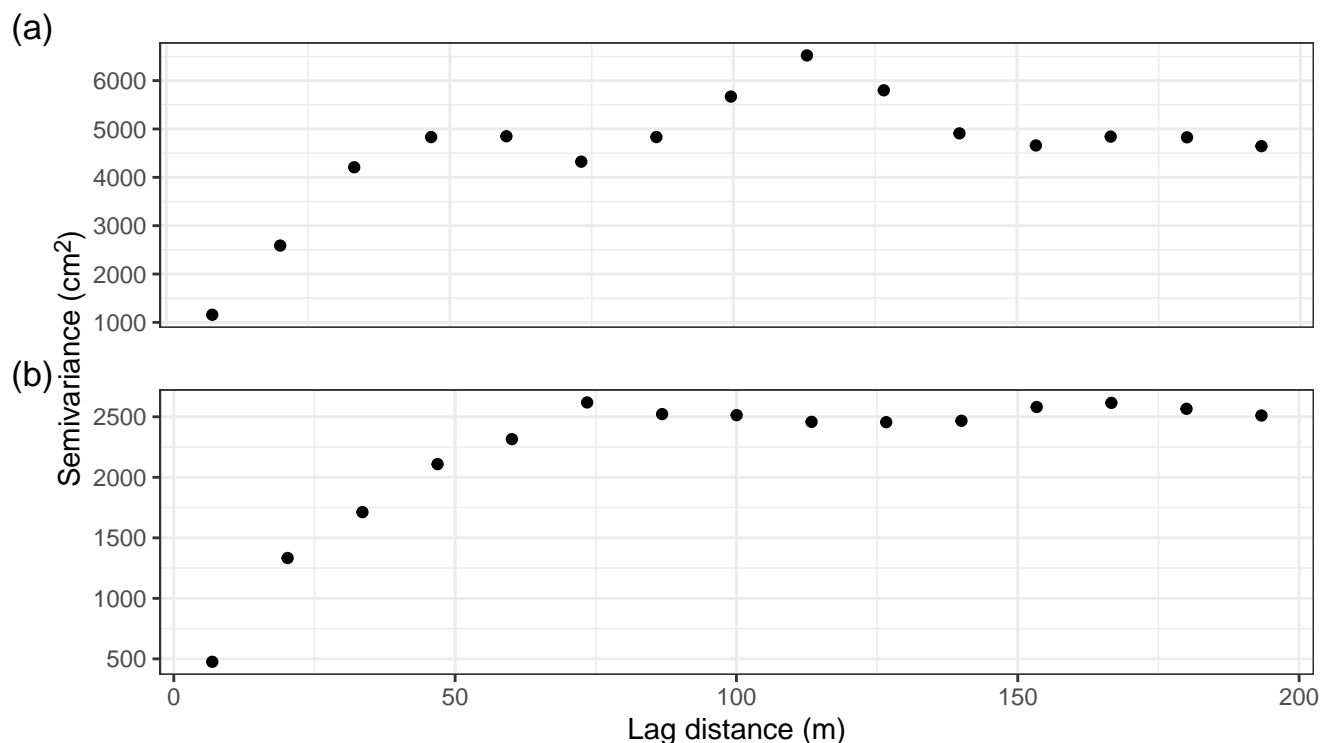
Figure B1. Empirical semivariograms of peat depth point measurements at Skrimfjella (a) and Ørskogfjellet (b).
