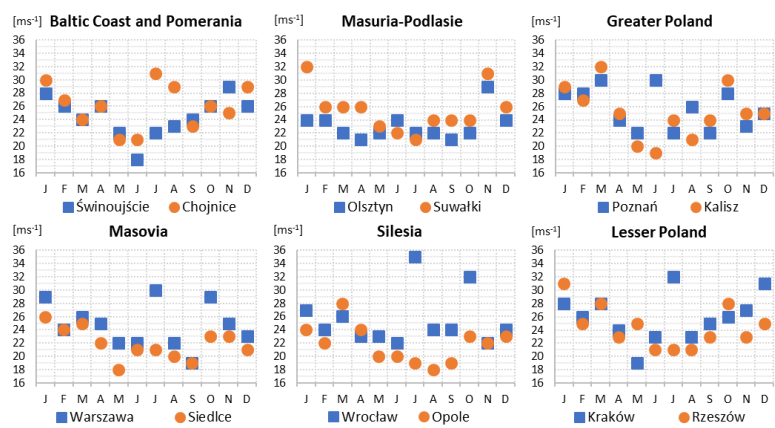
Figure 13. Maximum monthly wind gust speeds ( \text{ms}^{-1} ) at selected stations in Poland representing the six studied regions, 1993–2022
