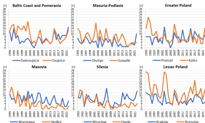
Fig. 11. Year-to-year course of the annual number [n] of gust winds of >17 \text{ ms}^{-1} at selected stations representing six studied regions in Poland, 1993–2022
