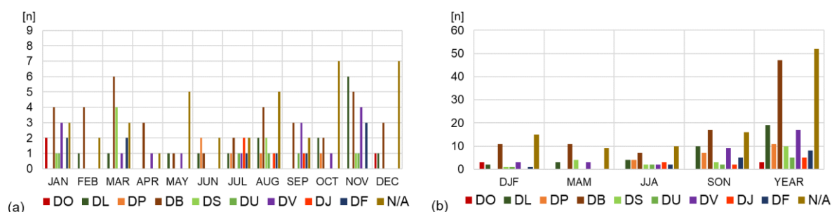
Fig. 9. Monthly (a) and seasonal and annual (b) number [n] of strong winds in Poland for which information about the character of damage exists (DO, DL, DP, DB, DS, DU, DV, DJ and DF) or does not exist (N/A), 1281–1600. For explanations of abbreviations, see the Methods section.
