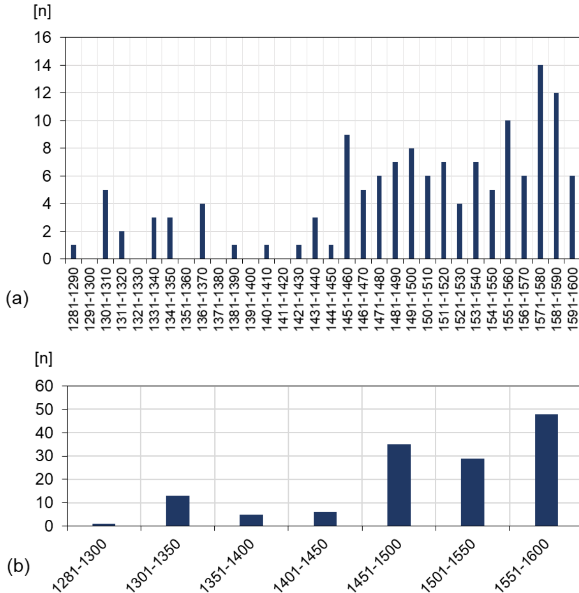
Fig. 3. Decadal (a) and 50-year (b) number of occurrences [n] of strong winds of all categories in Poland, 1281–1600
