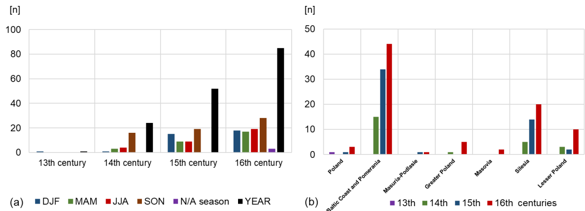
Fig. 2. Number [n] of weather notes for Poland for seasons (a) and regions (b), 1281–1600. Explanation: “N/A season” – specific season is not available (unknown); the category “Poland” encompasses all notes for which the region is unknown.
