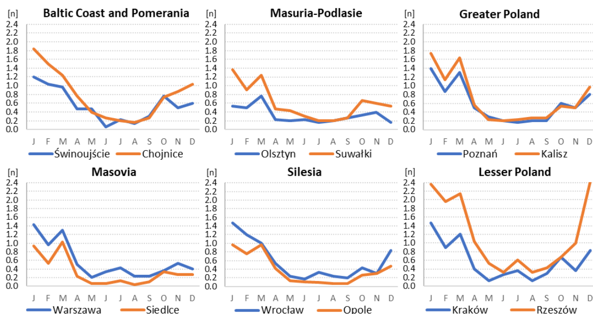
Fig. 12. Annual course based on the average monthly number [n] of gust winds of >17 \text{ ms}^{-1} at selected stations representing the six studied regions in Poland, 1993–2022
