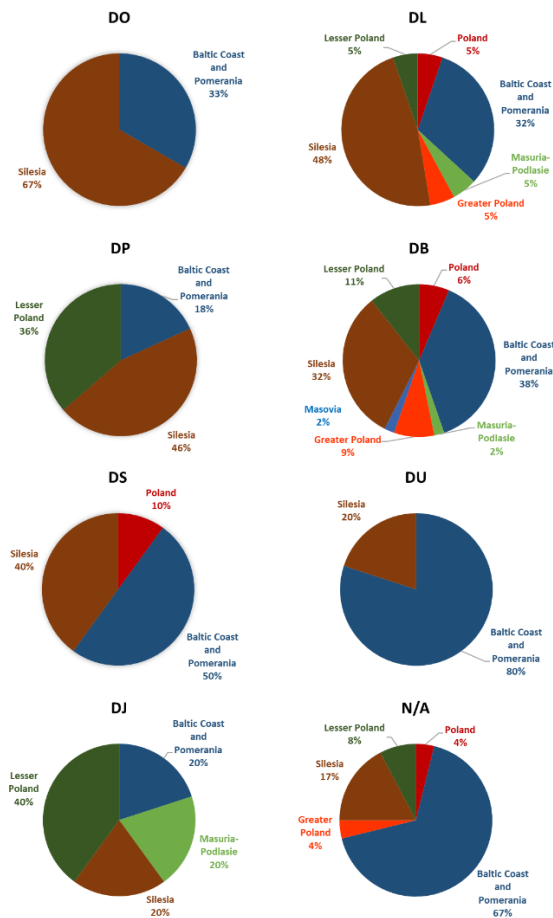
Fig. 10. Relative frequencies (%) of damage categories estimated for particular regions in Poland, 1281–1600
