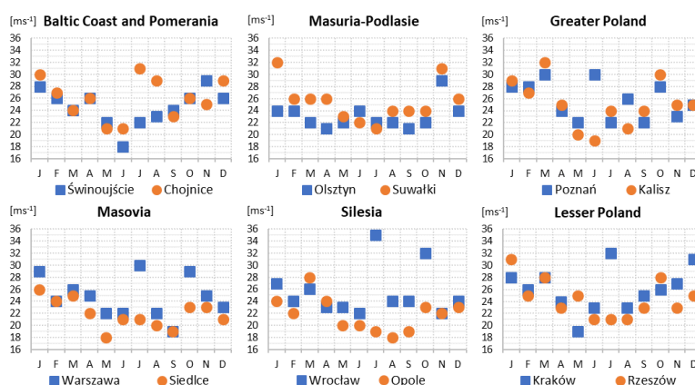
Fig. 13. Maximum monthly wind gust speeds ( \text{ms}^{-1} ) at selected stations in Poland representing the six studied regions, 1993–2022
