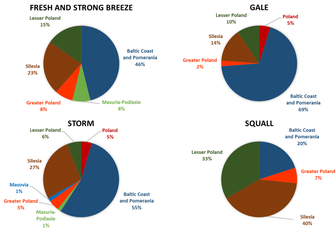
Fig. 6. Relative frequencies (%) of occurrence of strong winds of different types (tornadoes excluded) in the studied regions of Poland, 1281–1600
