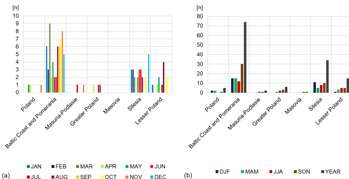
Fig. 4. Monthly (a) and seasonal (b) number [n] of strong winds of all categories by region, 1281–1600 Explanation: The total number of strong winds in seasons/years presented in Fig. 4b is greater than calculated based only on monthly statistics because some weather notes provide information about only the season or even only the year of occurrence (see also text in 2.2.1 and Table 1).
