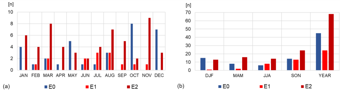
Fig. 7. Monthly (a) and seasonal (b) number of occurrences [n] of strong winds in Poland, according to extent of damage, 1281–1600
