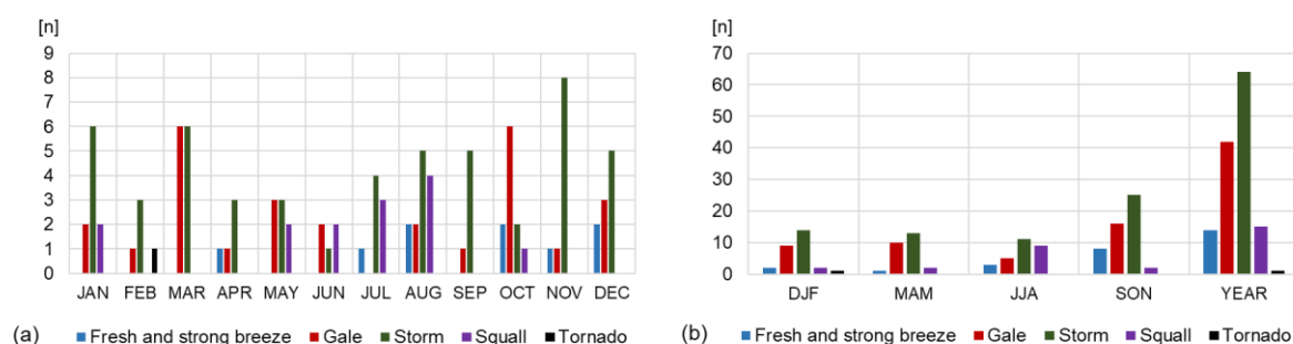
Fig. 5. Monthly (a) and seasonal (b) number of occurrences [n] of strong winds of different types in Poland, 1281–1600
