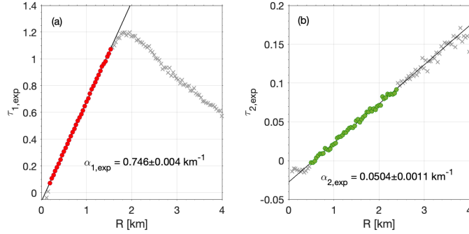
Figure 5: Differential optical depth for (a) \lambda_1 ( ^{12}\text{CO}_2 ) and (b) \lambda_2 ( ^{13}\text{CO}_2 ) and typical bisquare linear fit to estimate mean differential absorption coefficient. Colored dotted markers: points used for the fit; cross markers: outliers.
