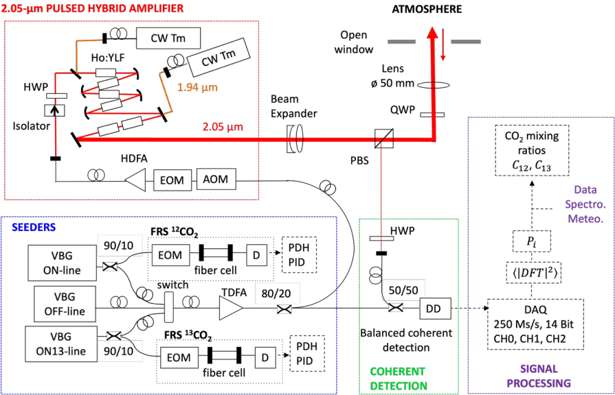
Figure 2: DIAL set-up for \delta^{13}\text{C} measurement. FRS : frequency reference system, EOM et AOM : electro and acoustic-optical modulators, HDFA and TDFA : Holmium and Thulium fiber amplifiers, VBG :volume Bragg grated laser diode, PDH : Pound-Drever-Hall, HWP and QWP :half and quarter wave plate, PBS : polarizer beam splitter. Signal processing: data acquisition system (DAQ) with 3 channels (CH0, CH1 and CH2) for the 3 wavelengths, real time range-gate Discrete Fourier Transform (DFT), backscatter power ( P_i ) at each wavelength and ^{12}\text{CO}_2 ( C_{12} ) and ^{13}\text{CO}_2 ( C_{13} ) mixing ratios computed with additional spectroscopic and in situ meteorological data.
