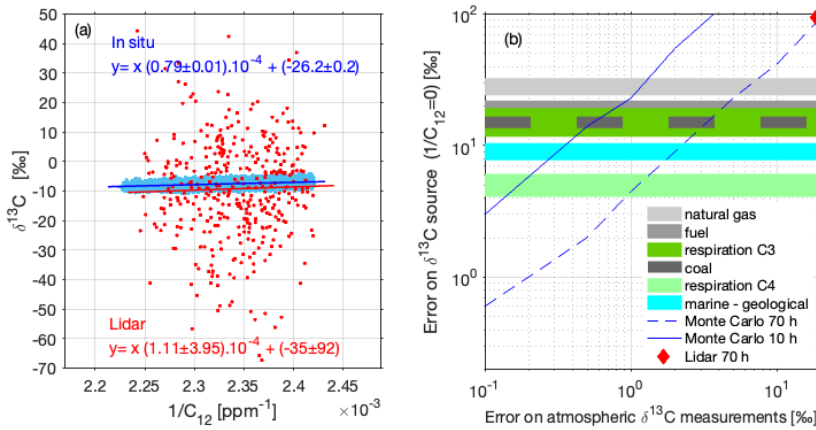
Figure 9: (a) Keeling plot for in situ gas analyzer and CDIAL measurements (b) Monte Carlo simulations of the \delta^{13}C_{source} error estimate (time resolution is 10 min) using in situ gas analyzer as the truth and random additional noise on \delta^{13}C measurements. Lidar error on \delta^{13}C_{source} estimate with 70h of measurements is indicated as well as \delta^{13}C_{source} geophysical typical anomalies for natural gas, fuel, coal anthropogenic emissions, C-3 and C-4 plant respiration and marine or geological source with respect to standard atmospheric mixed air \delta^{13}C (9‰).
