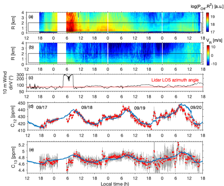
385 Figure 8: C_{12} and C_{13} lidar measurements. (a) Lidar reflectivity for wavelength 0 and associated (b) Lidar radial wind speed. (c) In situ horizontal wind direction ( dirV ) at 10 m and lidar line-of-sight (LOS) azimuth angle. (d) C_{12} and (e) C_{13} lidar mixing ratio measurements (markers). The solid line corresponds to in situ PICARRO G2101-i analyzer measurements. Space resolution for lidar C_{12} and C_{13} measurements is around 1.0-1.3 and 1.5-1.8 km respectively depending on the level of the signal power (panel (a)). Time resolution is 10 min. Error bars are calculated from \alpha_{exp} estimates (Fig. 5).
