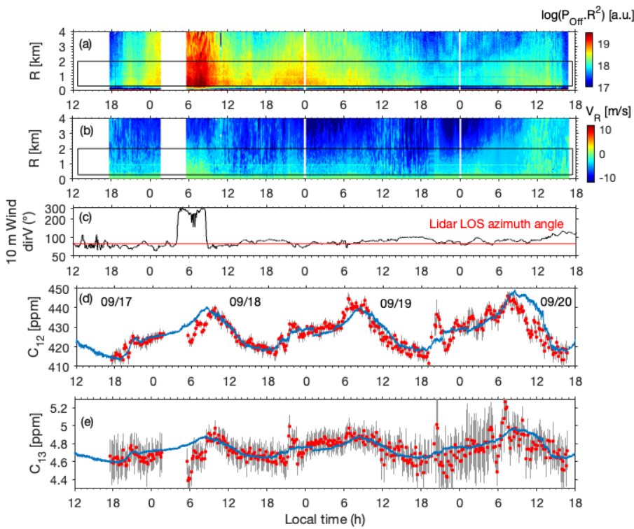
355 Figure 8: C_{12} and C_{13} lidar measurements. (a) Lidar reflectivity for wavelength 0 and associated (b) Lidar radial wind speed. (c) In situ horizontal wind direction ( dirV ) at 10 m and lidar line-of-sight (LOS) azimuth angle. (d) C_{12} and (e) C_{13} lidar mixing ratio measurements (markers). The solid line corresponds to in situ PICARRO G2101-i analyzer measurements. Space resolution for lidar C_{12} and C_{13} measurements is around 1.0-1.3 and 1.5-1.8 km respectively depending the level of the signal power (panel (a)). Time resolution is 10 min. Error bars are calculated from \alpha_{1,exp} estimates (Fig. 5).
