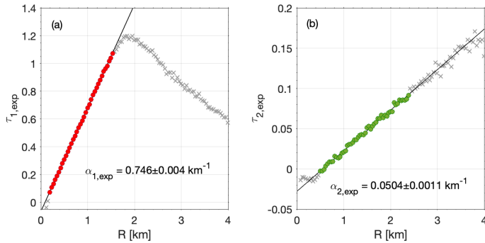
240 Figure 5: Differential optical depth for (a) \lambda_1 ( ^{12}\text{CO}_2 ) and (b) \lambda_2 ( ^{13}\text{CO}_2 ) and typical bisquare linear fit to estimate mean differential absorption coefficient. Colored dotted markers: points used for the fit; cross markers: outliers.
