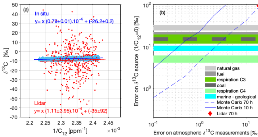
385 Figure 9: (a) Keeling plot for in situ gas analyzer and CDIAL measurements (b) Monte Carlo simulations of the \delta^{13}C_{source} error estimate (time resolution is 10 min) using in situ gas analyzer as the truth and random additional noise on \delta^{13}C measurements. Lidar error on \delta^{13}C_{source} estimate with 70h of measurements is indicated as well as \delta^{13}C_{source} geophysical typical anomalies for natural gas, fuel, coal anthropogenic emissions, C-3 and C-4 plant respiration and marine or geological source with respect to standard atmospheric mixed air \delta^{13}C (9‰).
