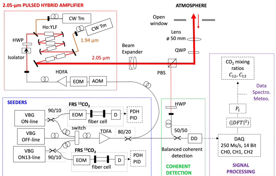
175 Figure 2: DIAL set-up for \delta^{13}\text{C} measurement. FRS : frequency reference system, EOM et AOM : electro and acoustic-optical modulators, HDFA and T DFA : Holmium and Thulium fiber amplifiers, VBG : volume Bragg grated laser diode, PDH : Pound-Drever-Hall, HWP and QWP : half and quarter wave plate, PBS : polarizer beam splitter. Signal processing: data acquisition system (DAQ) with 3 channels (CH0, CH1 and CH2) for the 3 wavelengths, real time range-gate Discrete Fourier Transform (DFT), backscatter power ( P_i ) at each wavelength and ^{12}\text{CO}_2 ( C_{12} ) and ^{13}\text{CO}_2 ( C_{13} ) mixing ratios computed with additional spectroscopic and in situ meteorological data.
