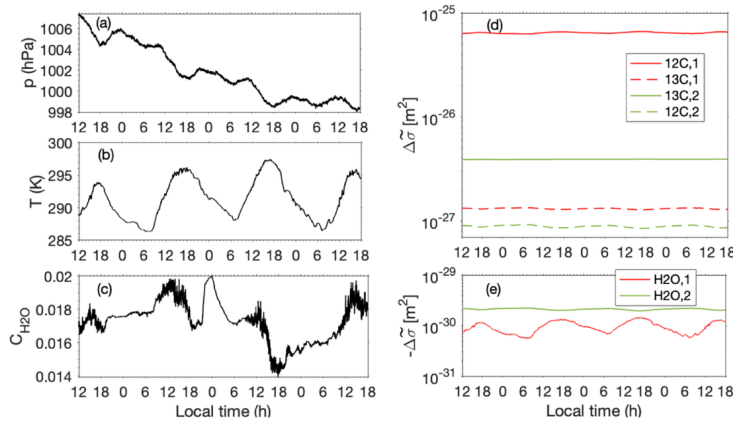
260 Figure 6: Meteorological data and differential ACS calculations. (a) Pressure (b) Temperature (c) \text{H}_2\text{O} mixing ratio (d) Differential ACS at wavelength 1 and 2 for ^{12}\text{CO}_2 and ^{13}\text{CO}_2 absorption lines and (e) for \text{H}_2\text{O} . Note that, as for Fig. 1, ^{13}\text{CO}_2 ACS
