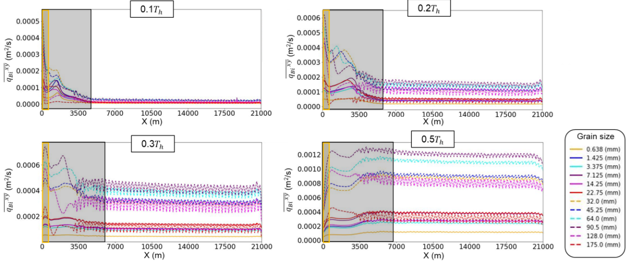
Fig. 11 Longitudinal distribution of the magnitude of cross-sectional average sediment transport flux, \overline{q_{Bl}^{xy}} ( =\sqrt{(q_{Bl}^x)^2 + (q_{Bl}^y)^2} ), for each grain size at each time ( 0.1T_h , 0.2T_h , 0.3T_h , and 0.5T_h within the final hydrograph) in Case 1-b. Yellow and grey areas indicate HBL-like reach and the affected length by bedload sheets, respectively.
