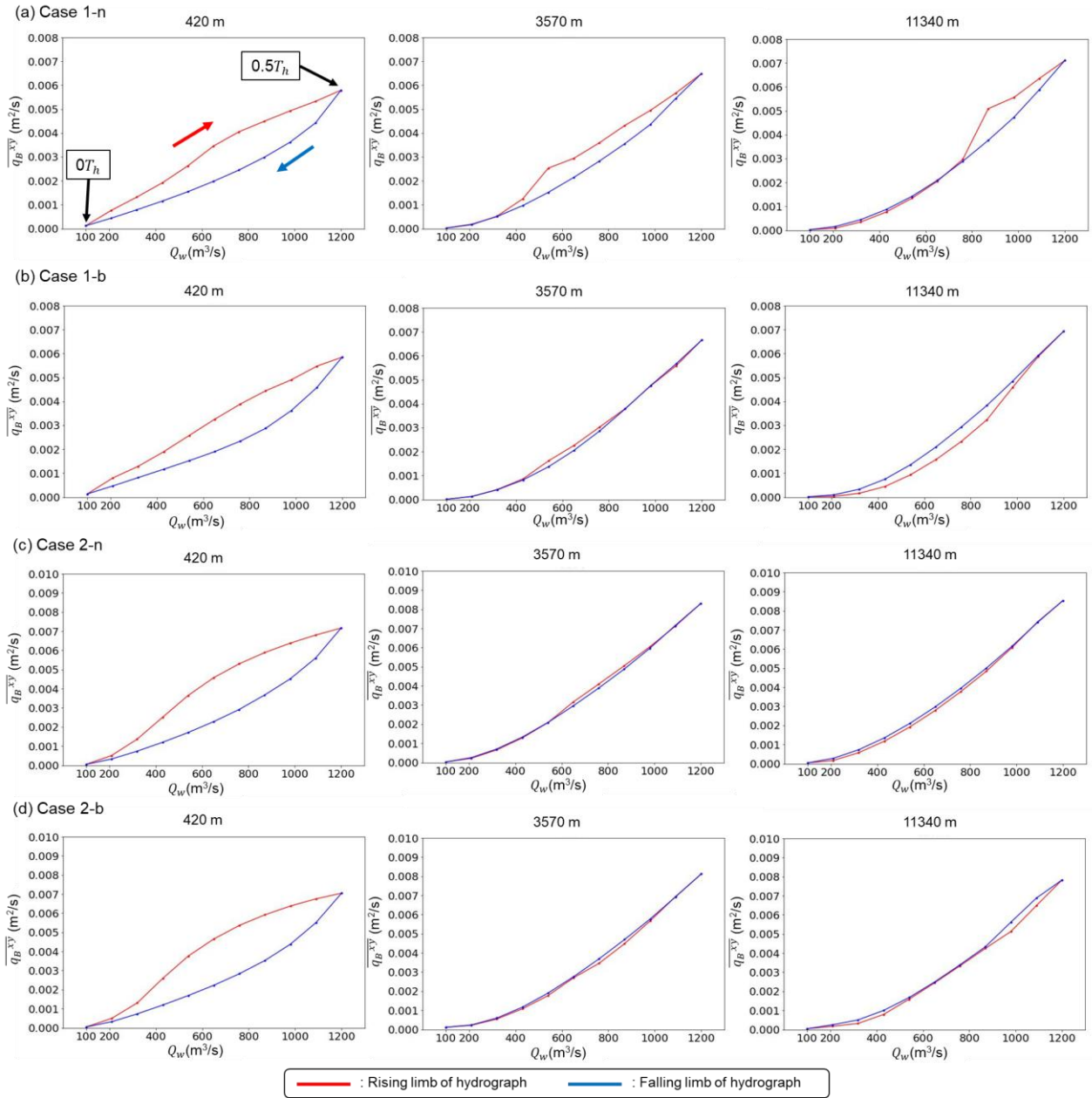
Fig. 13 Temporal variation of flow discharge, Q_w and the magnitude of cross-sectional average sediment transport flux, q_B^{xy} , within the last final hydrograph: (a) Case 1-n; (b) Case 1-b; (c) Case 2-n; and (d) Case 2-b. The red and the blue lines correspond to the rising limb and the falling limb, respectively.
