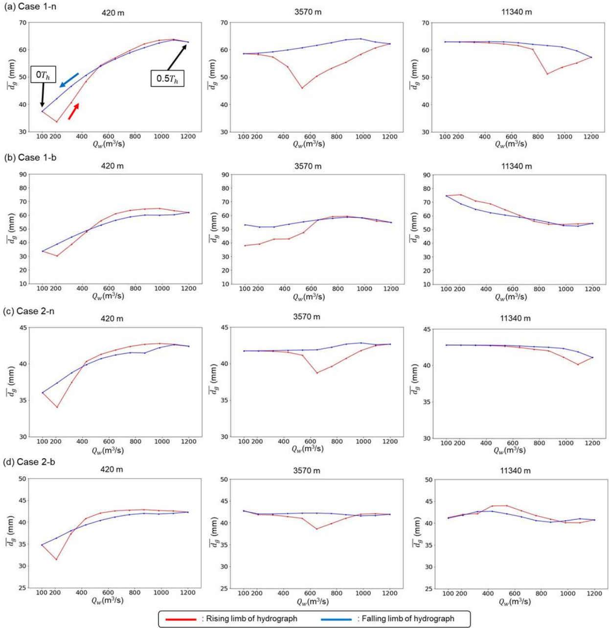
Fig. 15 Temporal variation of flow discharge, Q_w , and the cross-sectional average geometric mean diameter, \bar{d}_g , within the last final hydrograph: (a) Case 1-n; (b) Case 1-b; (c) Case 2-n; and (d) Case 2-b. The red and the blue lines correspond to the rising limb and the falling limb, respectively.
