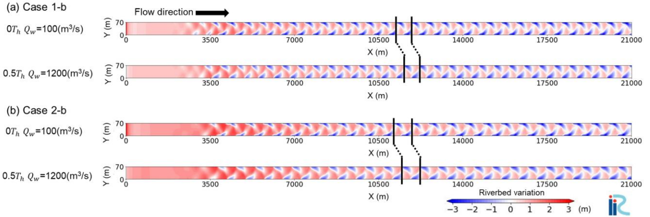
Fig. 6 The two-dimensional riverbed variation from the initial riverbed elevation at 0T_h (upper panel) and 0.5T_h (lower panel) within the final hydrograph : (a) case 1-b; (b) case 2-b. The black lines across the channel show the migration distance of a single alternate-bars.
