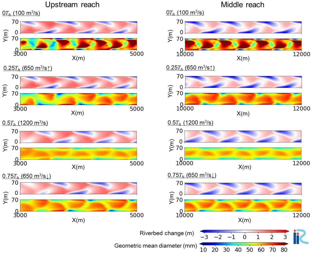
Fig. 8 Two dimensional distributions of riverbed change (upper panel) and surface geometric mean diameter (lower panel) at each time ( 0T_h , 0.25T_h , 0.5T_h , 0.75T_h within the final hydrograph ) in Case 1-b.
