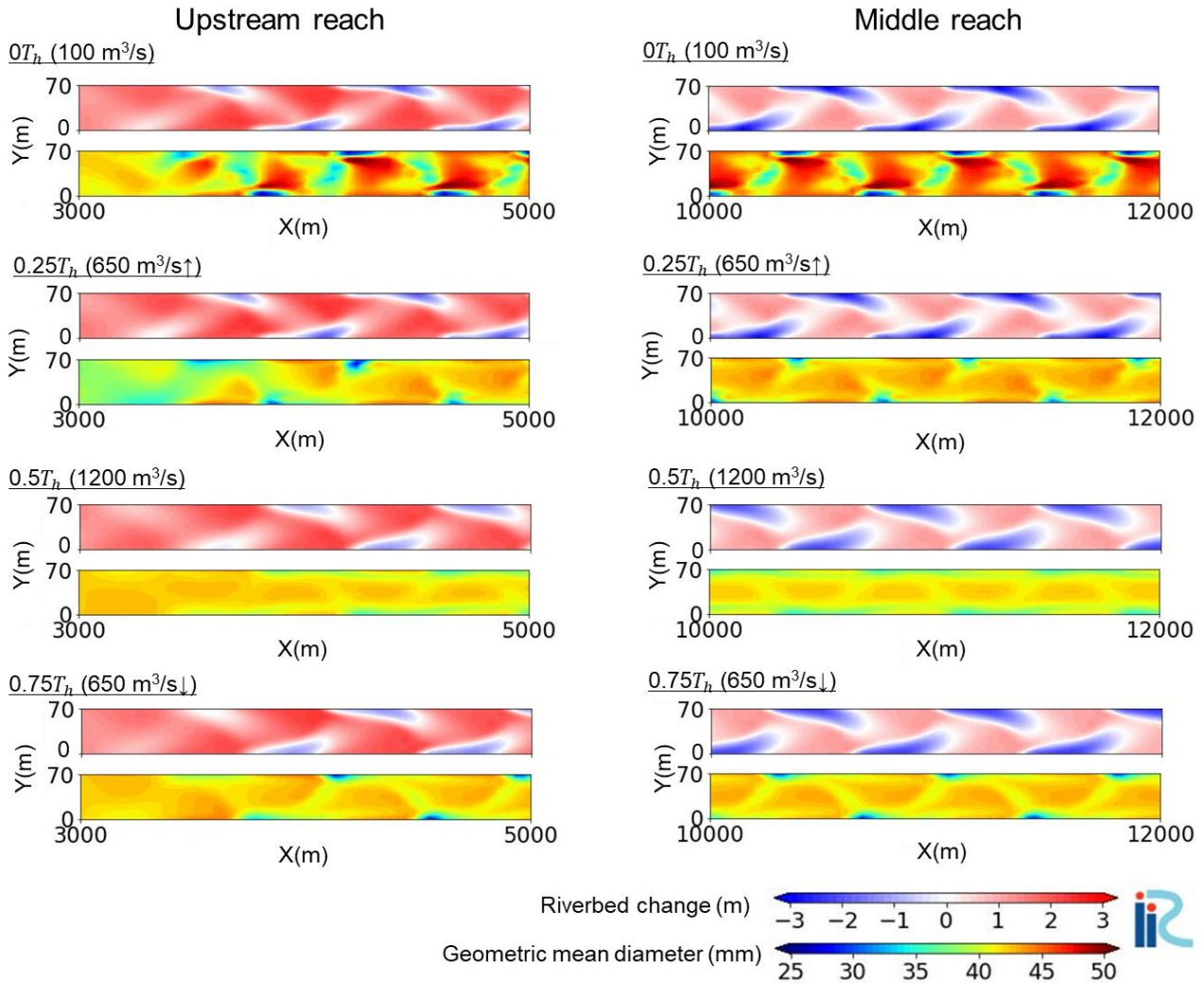
Fig. 9 Two dimensional distributions of riverbed change (upper panel) and surface geometric mean diameter (lower panel) at each time ( 0T_h , 0.25T_h , 0.5T_h , 0.75T_h within the final hydrograph ) in Case 2-b.
