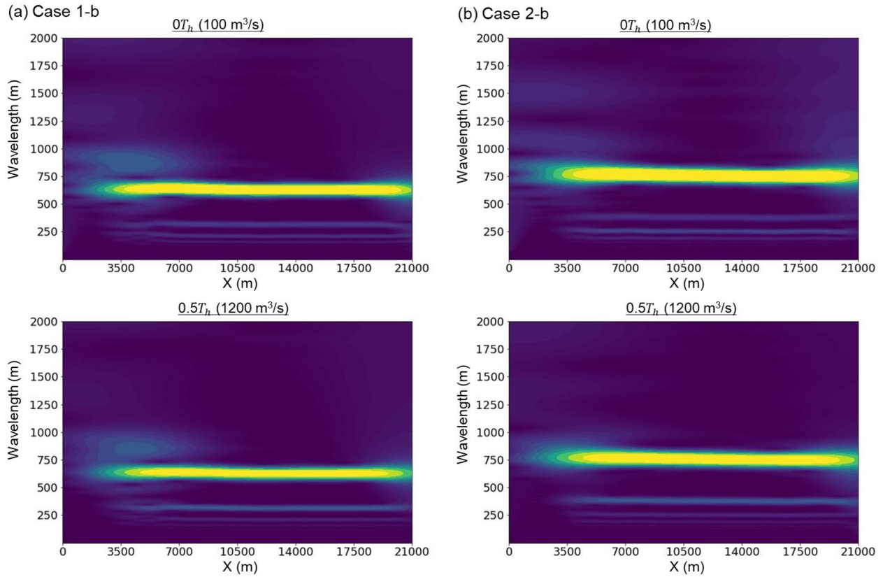
Fig. 10 Wavelet analysis of the dominant wavelength along the right bank ( Y=0 m) at 0T_h and 0.5T_h within the last final hydrograph: (a) Case 1-b, (b) Case 2-b.
