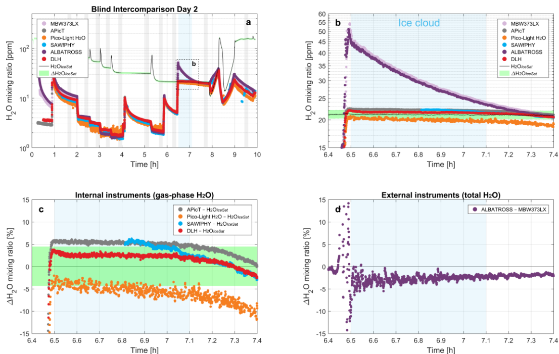
Figure 9. In-cloud measurements analysis. Panel (a): time series of \text{H}_2\text{O} mixing ratio measured by all instruments during BD2 (same as Fig. 4b), along with the ice saturated \text{H}_2\text{O} mixing ratio ( \text{H}_2\text{O}_{\text{IceSat}} ) calculated from p_{\text{AIDA}} and T_{\text{AIDA}} (black line) and its uncertainty (green shading). Panel (b): zoom into the ice cloud occurrence interval. Panel (c) relative differences (in percent) in gas-phase \text{H}_2\text{O} between all in situ instruments (APiCT, SP-APiCT, Pico-Light \text{H}_2\text{O} , SAWfPHY, DLH) and \text{H}_2\text{O}_{\text{IceSat}} . Panel (d): relative difference in total \text{H}_2\text{O} between the external instruments ALBATROSS and MBW373LX. In all panels, the blue shaded area highlights the interval of ice cloud occurrence (relative time 6.5–7.1 h).
