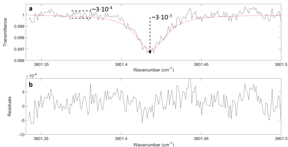
Figure A3. Pico-Light H_2O unitary spectrum (10 ms integration time) of the “stratospheric line” at 3801.41863 \text{ cm}^{-1} during BD3 at extremely dry conditions ( p_{AIDA} = 71.5 hPa, T_{AIDA} = 190.5 K, 0.81 ppm H_2O ) (panel a), and corresponding fit residuals (b).
