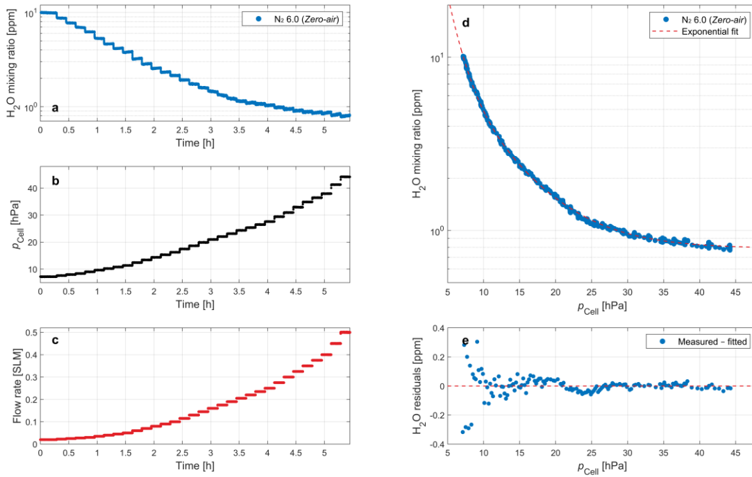
Figure A2. Overview of the nighttime ALBATROSS zero-air ( \text{N}_2 6.0) measurements performed between BD2 and BD3. Panels (a–c): time series of the measured \text{H}_2\text{O} mixing ratio, cell pressure ( p_{\text{Cell}} ) and flow rate, respectively. Panel (d): \text{H}_2\text{O} mixing ratio in the zero-air as function of p_{\text{Cell}} (blue markers) and exponential fit (red line), and the associated fit residuals (panel e).
