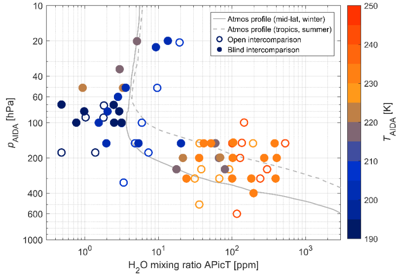
Figure 2. Scatter plot of pressure ( p_{AIDA} ) vs. H_2O mixing ratio (according to APicT measurements) and temperature ( T_{AIDA} , color-coded) measured during all static intervals (i.e., setpoint) of the intercomparison, overlaid with two atmospheric profiles of UTLS H_2O . The profiles correspond to tropical summer conditions (dashed grey line: Brunamonti et al., 2018) and mid-latitude winter conditions (solid grey line: Graf et al., 2021) and were smoothed by a \pm 1 km moving average. Open intercomparison and blind intercomparison setpoints are indicated by open and filled circles, respectively.
