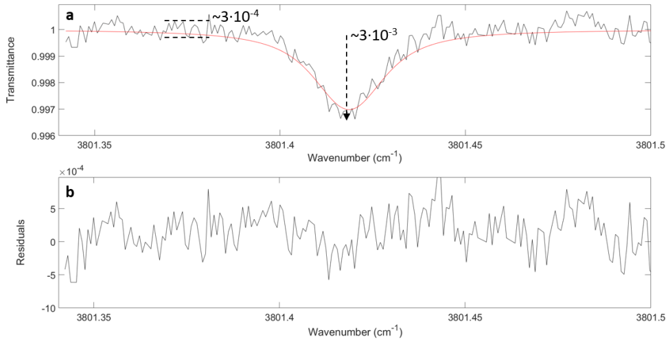
Figure A3. Pico-Light H_2O unitary spectrum (10 ms integration time) of the “stratospheric line” at 3801.41863 \text{ cm}^{-1} during BD3 at extremely dry conditions ( p_{AIDA} = 71.5 hPa, T_{AIDA} = 190.5 K, 0.81 ppm H_2O ) (panel a), and corresponding fit residuals (b).
