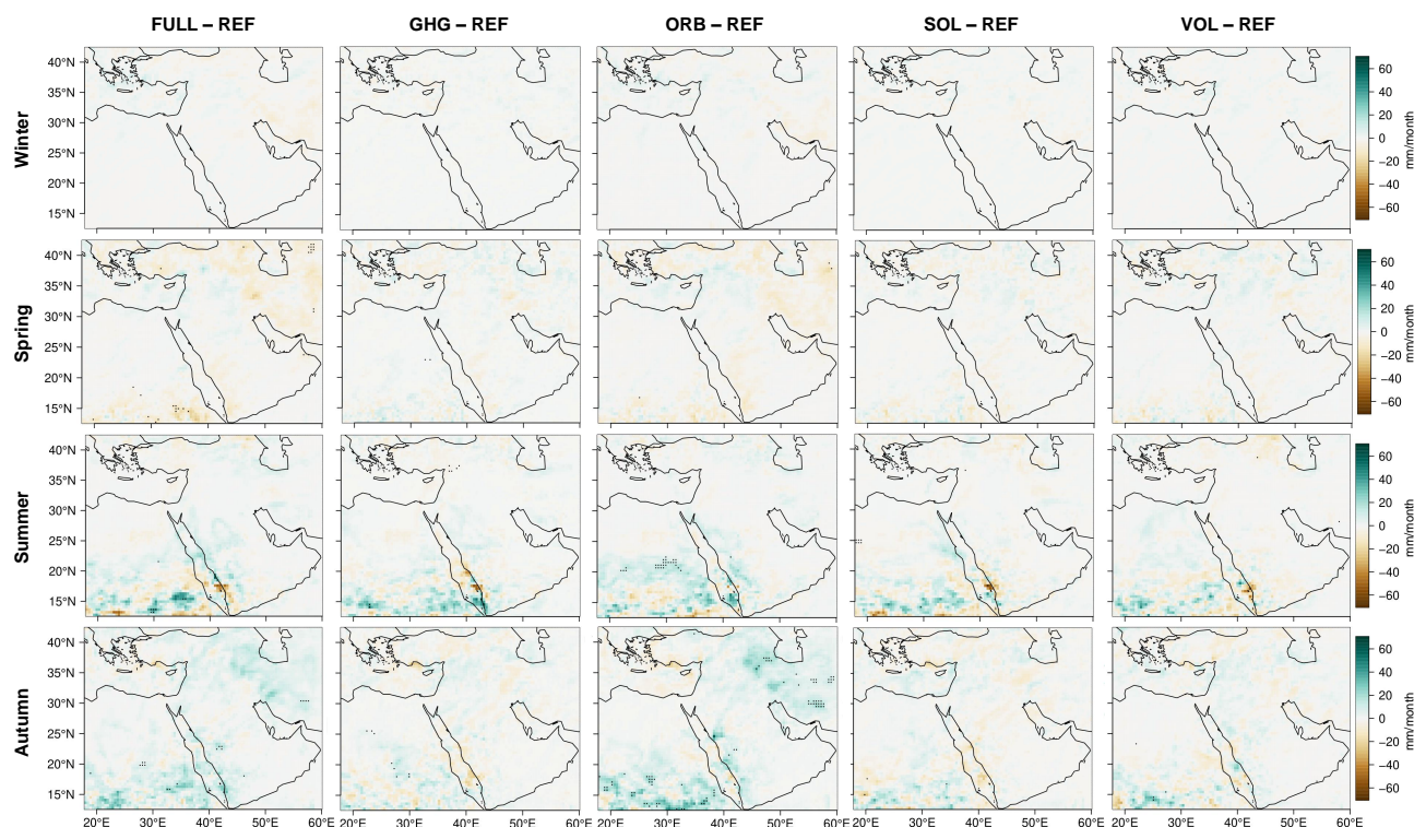
Figure 12. Seasonal mean of monthly precipitation sums for the decade 1255-1264 for the different simulations compared to REF. Significant differences are marked with a dot (Student's t-test, \alpha=0.05 ). From left to right - FULL, GHG, ORB, SOL, VOL and from top to bottom - winter, spring, summer, autumn.
