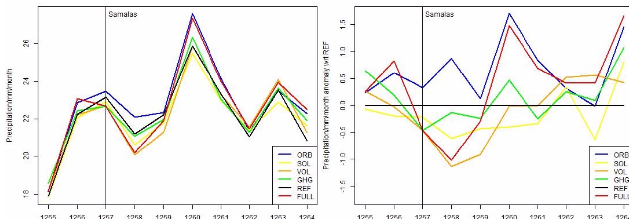
Figure 11. Annual mean total monthly precipitation averaged over the EMME domain (left) for the simulations with the different forcings and the same values represented as anomaly (right) with respect to the reference CCLM from 1255 to 1264.
