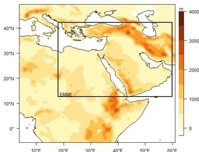
Figure 2. Simulation domain with topography and the EMME region in the black rectangle.
