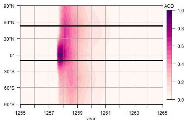
Figure 1. AOD from 1255 to 1265 for the different latitudinal bands. The latitudes used for the simulations are between the bars. Own representation of Toohey and Sigl (2017).
