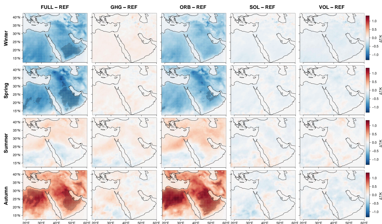
Figure 7. Mean seasonal temperature for the decade 1255-1264 for the different experiments compared to REF. Significant differences are marked with a dot (Student's t-test, \alpha=0.05 ). From left to right - FULL, GHG, ORB, SOL, VOL and top to bottom - winter, spring, summer, autumn.
