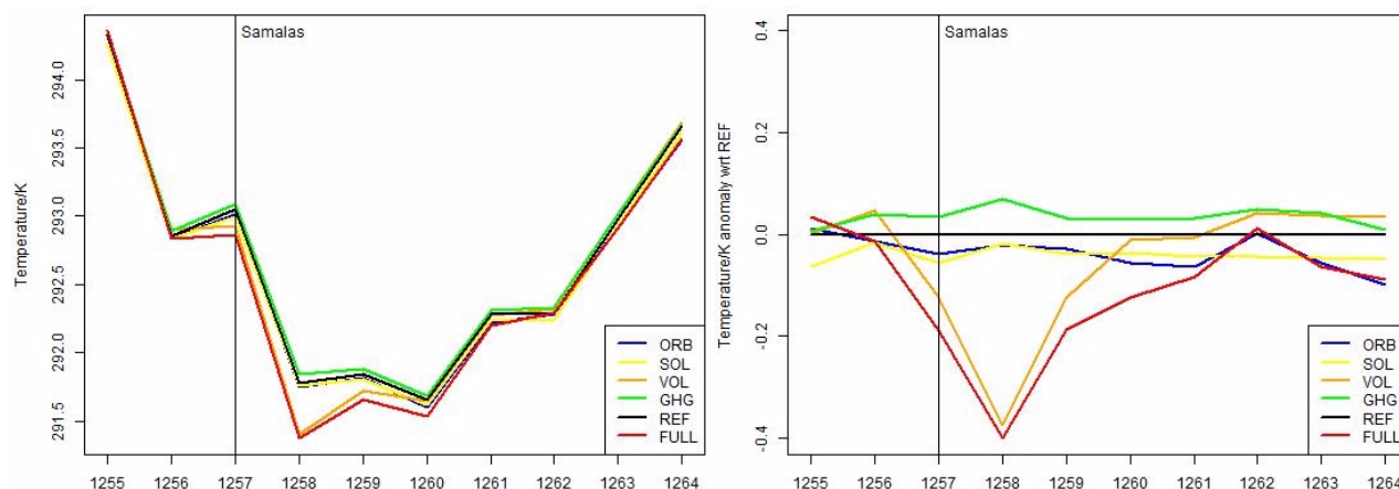
Figure 6. Annual mean 2m temperature averaged over the EMME domain (left) for the simulations with the different forcings and the same values represented as anomaly (right) with respect to the reference CCLM from 1255 to 1264.
