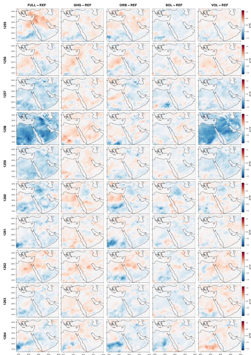
Figure B1. 2m temperature yearly distribution of differences between the differently forced CCLM simulations and the reference simulation without explicit forcing. Significant differences are marked with a dot. From left to right - FULL, GHG, ORB, SOL, VOL and from top to bottom - 1255 to 1264.
