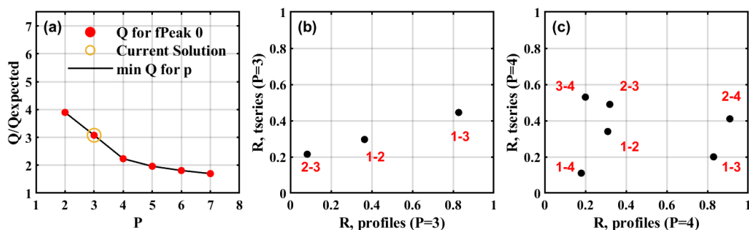
Figure R2. Key diagnostic plots of the PMF results. (a) Q/Q_{\text{expected}} as a function of number of factors ( P ); and cross-correlation coefficients ( R ) of the time series and spectral profiles among the PMF factors: (b) P = 3 and (c) P = 4 .
