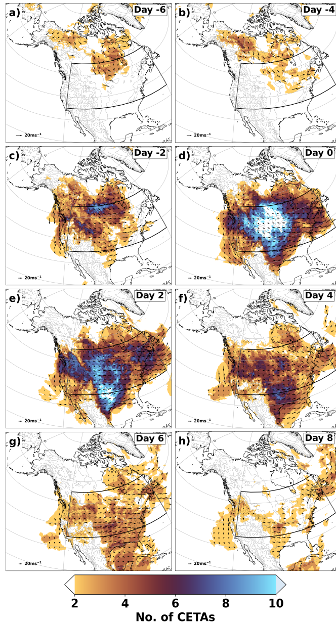
Figure 13. Same as Fig.11, but for southern North America region with a-h) showing day -6 to 8. Day-0 consists of 22 In total, 22 CS events were identified.
