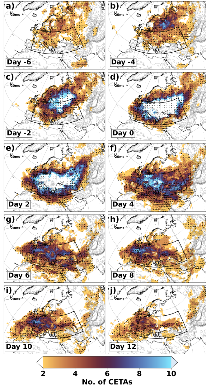
Figure 12. Same as Fig.11, but for southern Europe with a-j) showing day -6 to 12. Day 0 consists of 32 In total, 32 CS events were identified.
