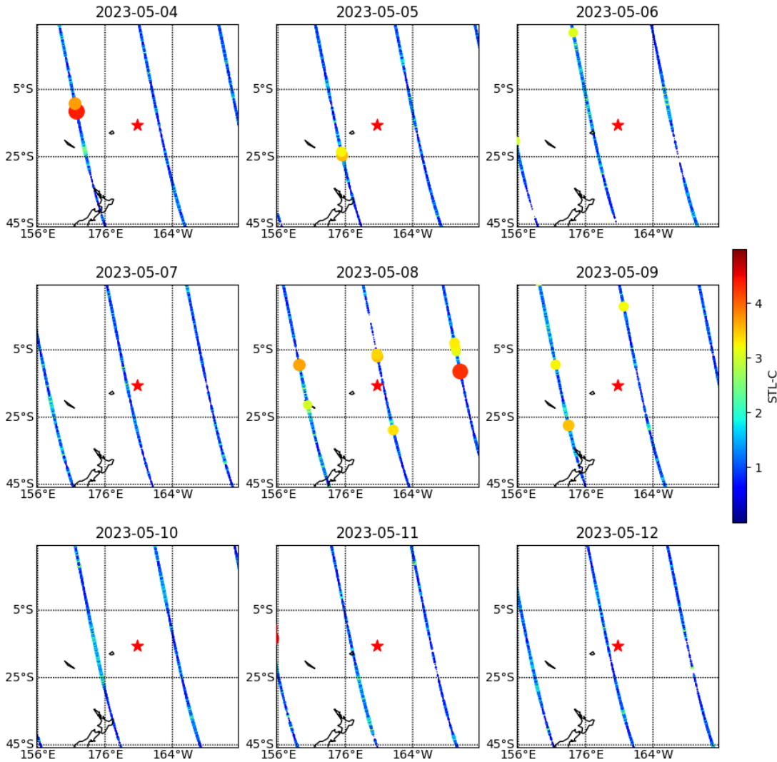
Figure 8: Daily variations of anomalous STL-C values surrounding the Mw7.6 Tonga earthquake epicenter (red star) from May 4 to May 12, 2023. The colored dots represent these anomalous STL-C values along the satellite ground track; both the size and color of the dots are scaled to their magnitude. The colorbar indicates this magnitude (Unit: unitless).
