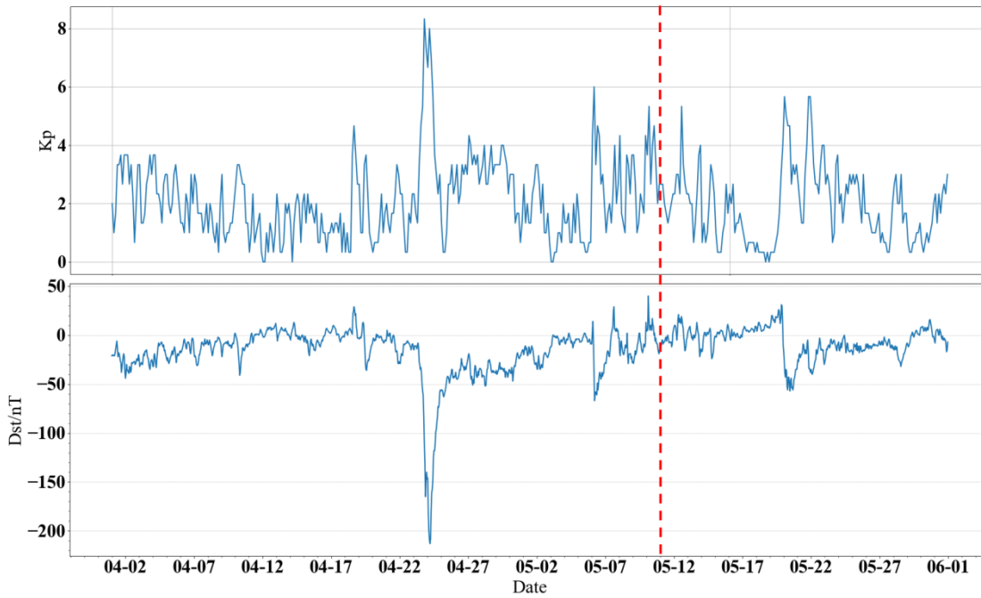
245 Figure 6: Variations in Kp and Dst Indices from April 1 to May 31, 2023 (Red Dashed Line Indicates the Time of Earthquake Occurrence).
