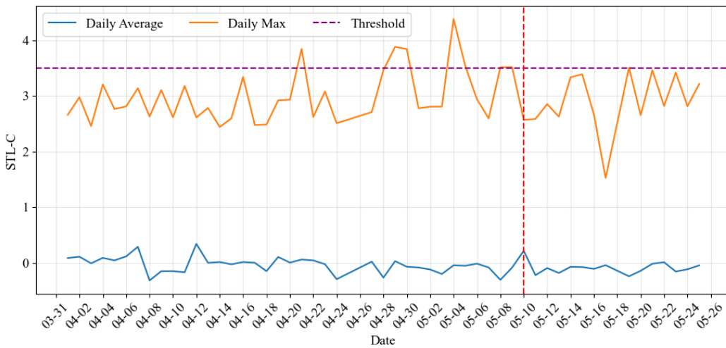
285 Figure 9: Variation Characteristics of STL-C Maximum and Average Values from April 1 to May 26, 2023. (Red Dashed Line Indicates the Time of Earthquake Occurrence)
