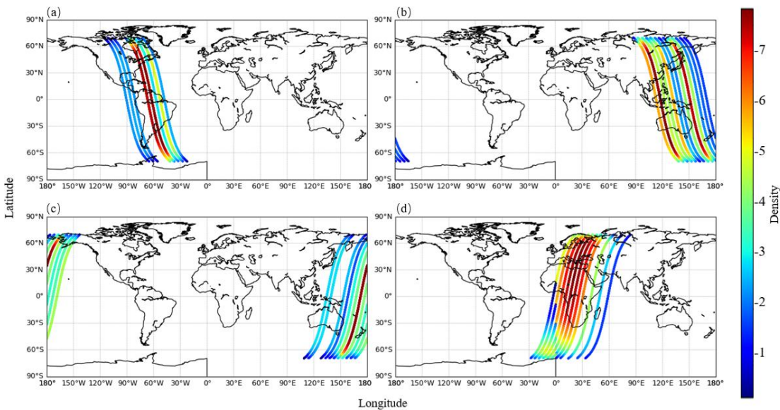
215 Figure 4: Spatial density distribution of the trend component peaks observed during May 2023. The colorbar indicates the density of peak occurrences (Unit: Counts). The subplots show the distributions for: (a) the first peak of the ascending orbits; (b) the second peak of the ascending orbits; (c) the first peak of the descending orbits; and (d) the second peak of the descending orbits.
