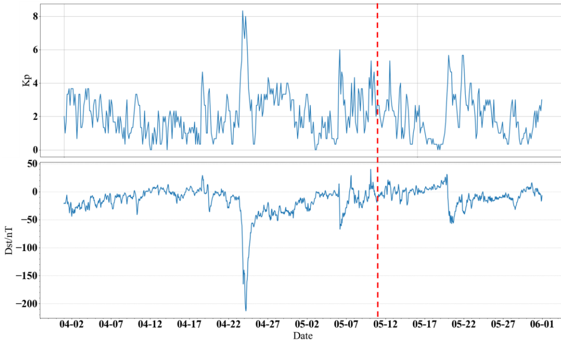
235 Figure 6: Variations in Kp and Dst Indices from April 1 to May 31, 2023 (Red Dashed Line Indicates the Time of Earthquake Occurrence)
