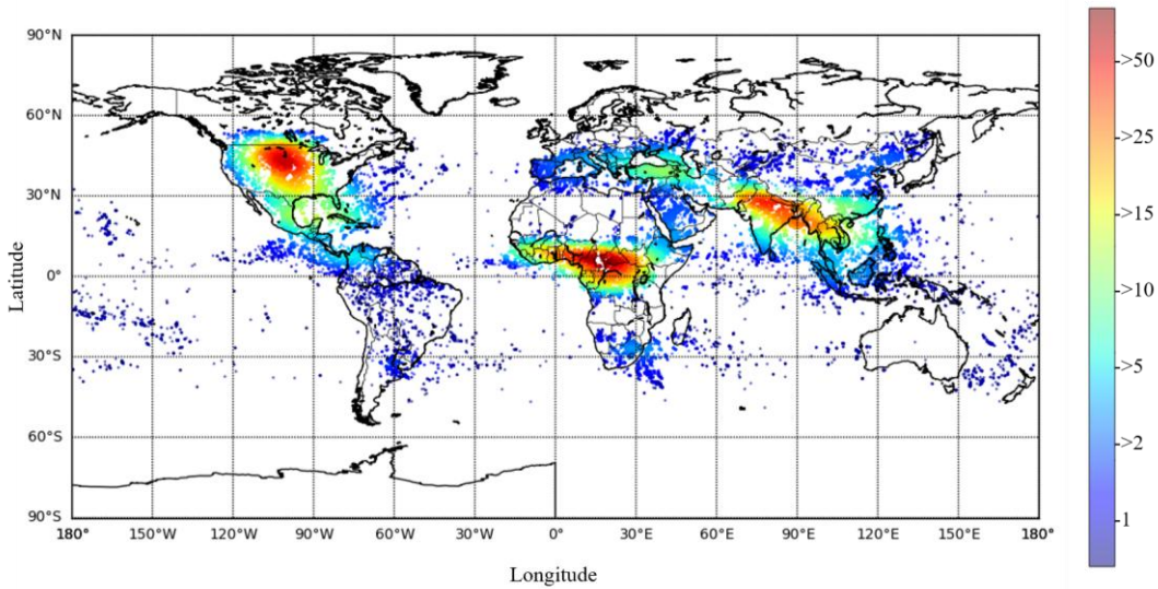
Figure 5: Global Lightning Distribution in May 2023
