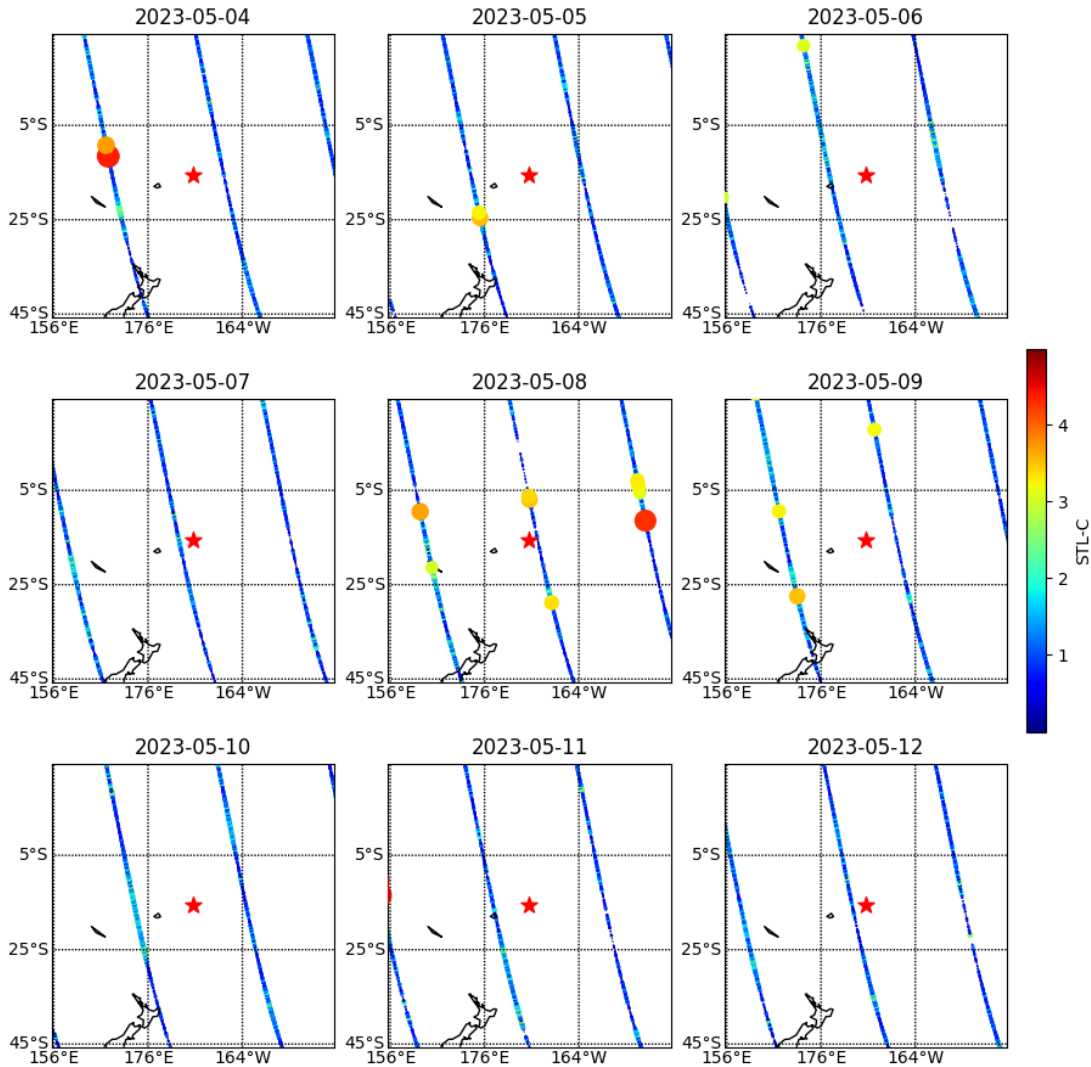
Figure 8: STL-C Variation Characteristics within the Seismic Region Before and After the Mw7.6 Tonga Islands Earthquake on May 11, 2023 (Red Star Indicates Epicenter Location)
