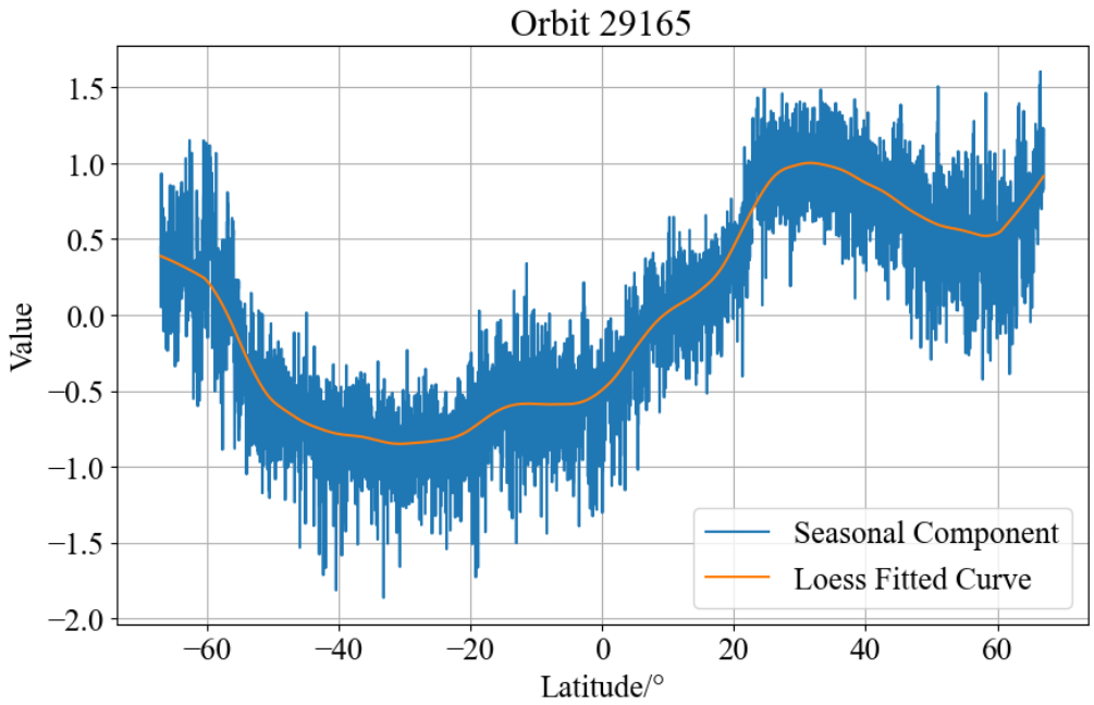
Figure 2: Seasonal Component Time Series for Orbit 29165 (Yellow Line Indicates Loess Fitting Results)
