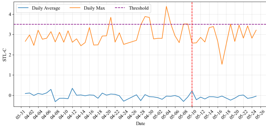
Figure 9: Variation Characteristics of STL-C Maximum and Average Values from April 1 to May 26, 2023
