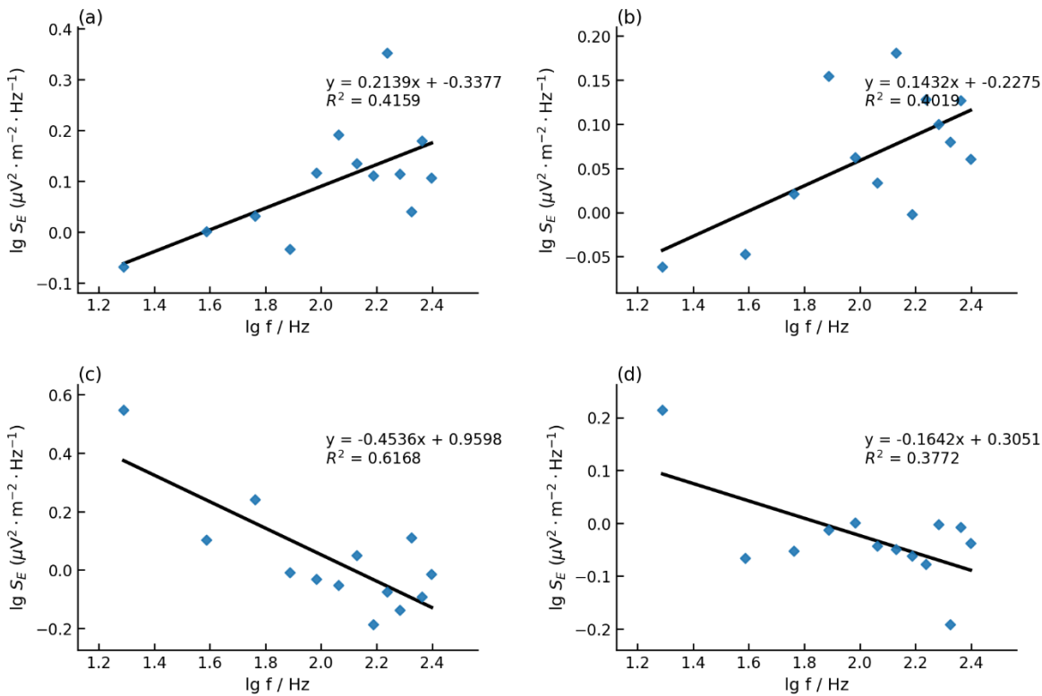
Figure 7: Linear fitting at four randomly selected observation points within one orbital cycle.(Each panel displays the logarithm of the electric field spectrum (blue diamonds) as a function of the logarithm of the frequency. The black line indicates the regression fit, with the corresponding equation and coefficient of determination ( R^2 ) shown in the top right corner of each panel.)
