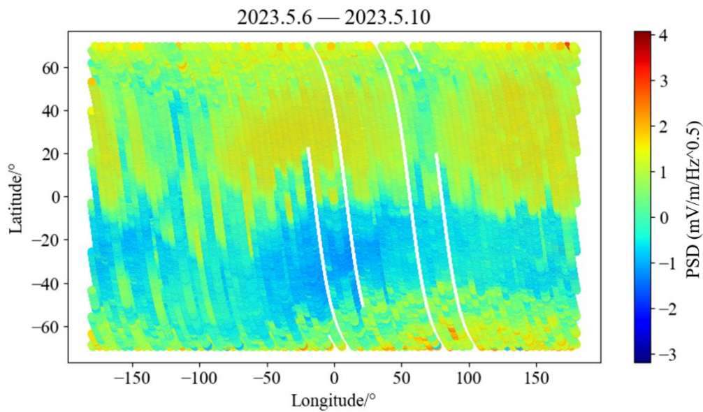
230 Figure 3: Spatial distribution map of the Original PSD Orbit-Projection-Map data observed by CSES-01 from May 6 to May 10, 2023.
