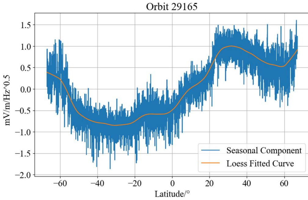
Figure 2: Seasonal Component Time Series Latitudinal profile of the seasonal component for Orbit 29165 (Yellow Line Indicates, (The orange line shows the Loess Fitting Results) fit to the seasonal data).
