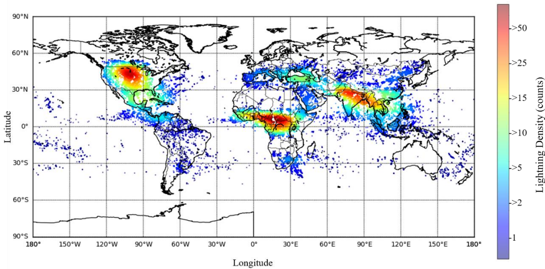
Figure 5: Global distribution of lightning activity in May 2023, based on data from the Lightning Distribution in May 2023 Imaging Sensor (LIS) .
