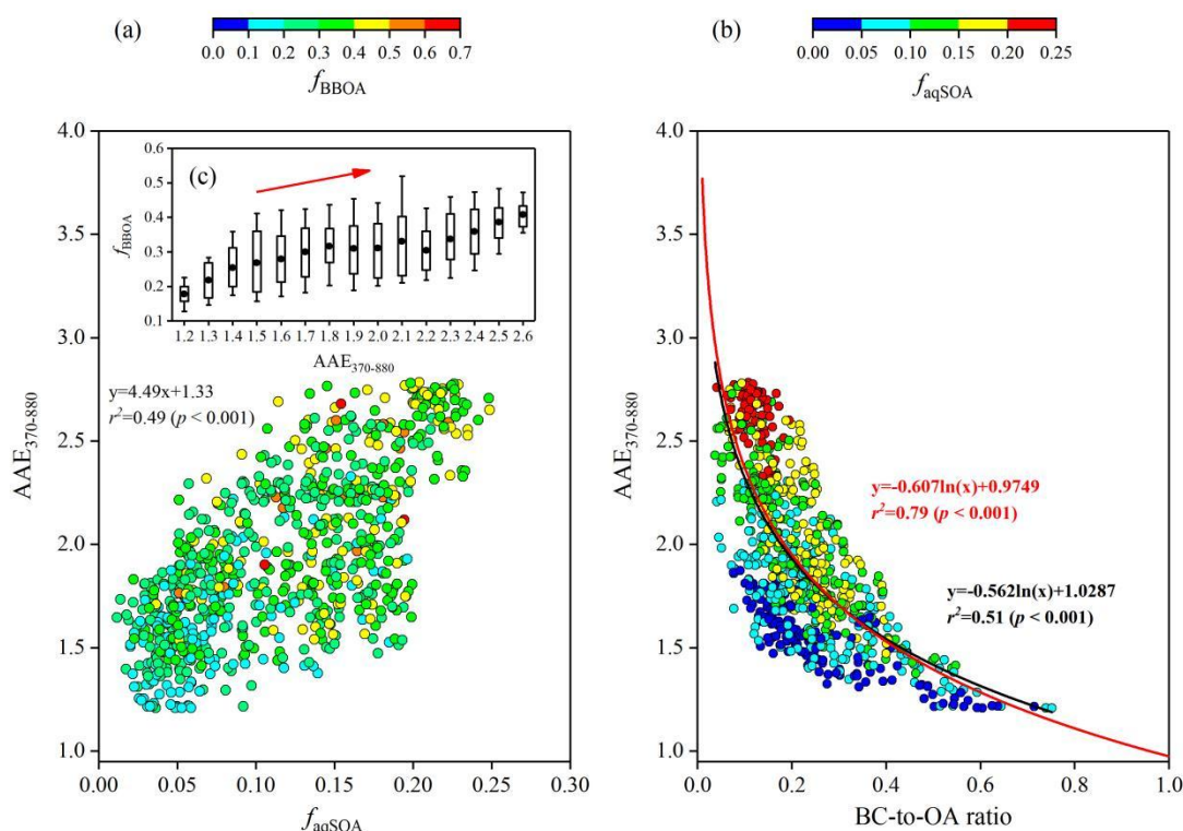
Figure 9. Relationship between (a) \text{AAE}_{370-880} and the mass fraction of aqSOA ( f_{\text{aqSOA}} = \text{aqSOA}/\text{OA} ) colored by the mass fraction of BBOA ( f_{\text{BBOA}} = \text{BBOA}/\text{OA} ), and (b) BC-to-OA ratios colored by f_{\text{aqSOA}} . (c) Variations of f_{\text{BBOA}} as a function of \text{AAE}_{370-880} . The red curve in (b) was the best fit curve to data taken from Lu et al. (2015) and described the Abs of fresh and aged BBOA.
