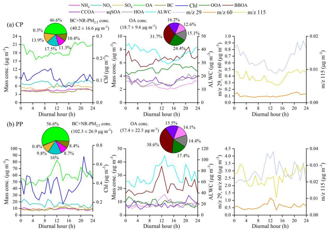
Figure 2. Diurnal variations of PM 2.5 species, BC, OA factors, m/z 29, m/z 60, and m/z 115 mass
