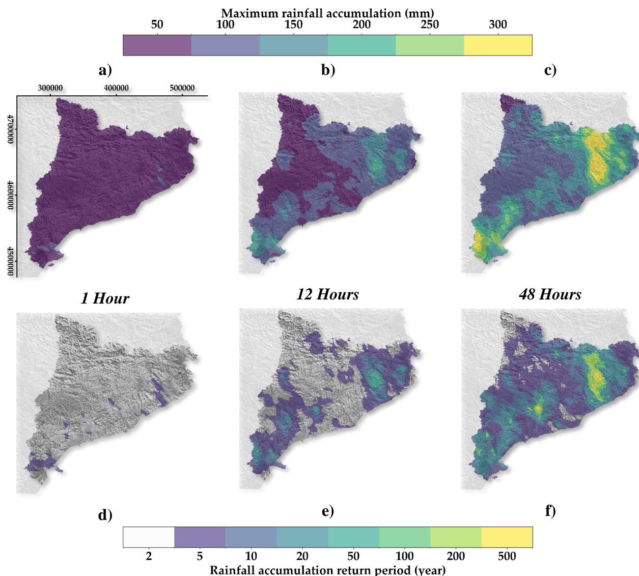
Figure 7. Geographical distribution of maximum rainfall accumulation (top) and return periods (bottom) for a duration of 1 hour (left), 12 hours (middle) and 48 hours (right) related to the meteorological hazard analysed.
