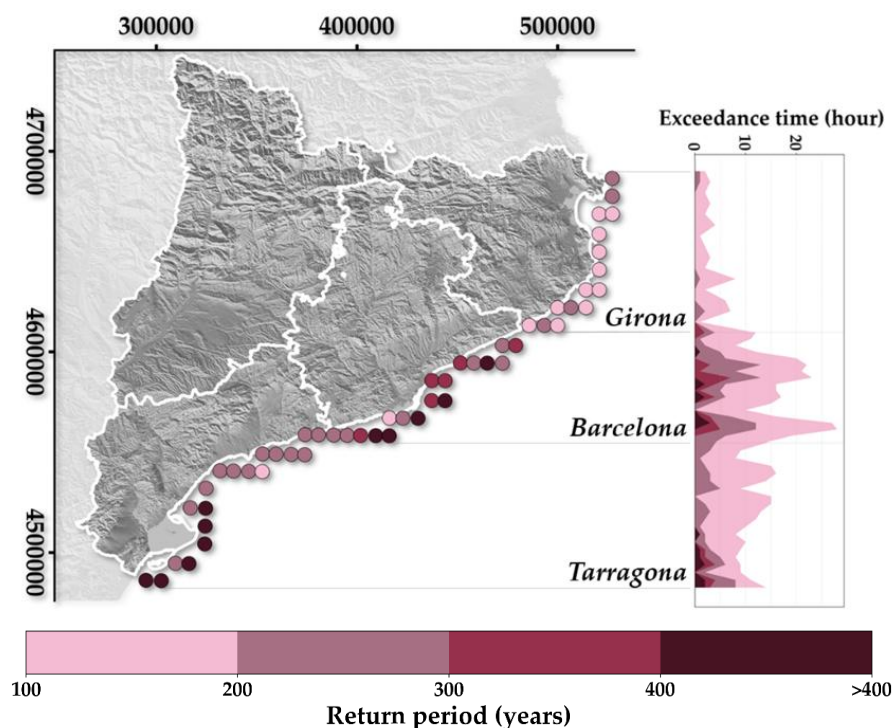
Figure 9. Geographical distribution of the significant wave height return periods related to the coastal hazard analysed and the hours of exceedance for the SIMAR grid nodes along the three coastal provinces.
