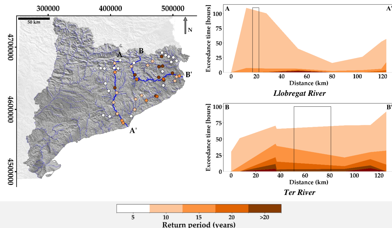
Figure 8. Geographical Distribution of the water discharge return periods related to the fluvial hazard analysed and the hours of exceedance for the Llobregat (A-A') and Ter (B-B') Rivers. Vertical lines in the longitudinal profiles mark the locations of major water reservoirs along each river.
