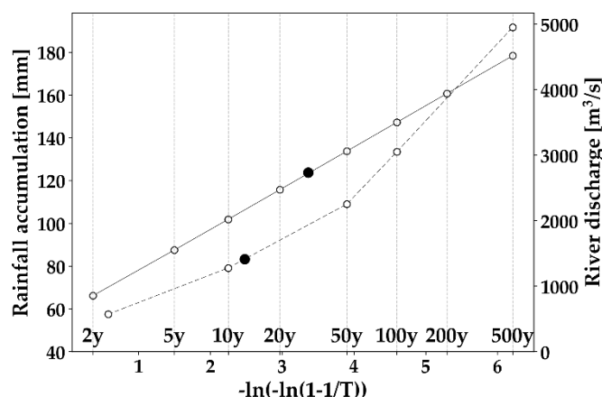
Figure 3. Example of return period estimates for meteorological (continuous line) and fluvial hazards (dashed line). The filled dots correspond to the Gloria storm event. 48-hour rainfall accumulation was selected for the meteorological hazard, and the observed discharge water level at the Llobregat river for the fluvial hazard.
