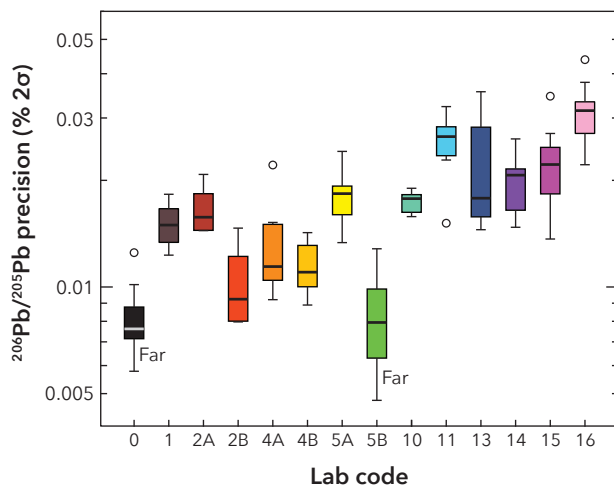
Figure 3. Precision of the uncorrected 206 Pb/ 205 Pb ratio by lab code. Labs 0 and 5B used Faraday detectors to analyse Pb isotopes, all others used ion counters.
