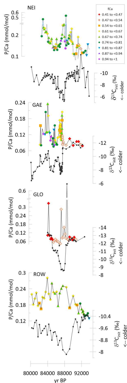
Figure 4. Time series of \delta^{13}\text{C}_{\text{init}} and P/Ca for stalagmites GAE, NEI, GLO, and ROW spanning the 92 to 80 ka time interval. The P/Ca symbols are color coded according to fCa as illustrated in the legend.
