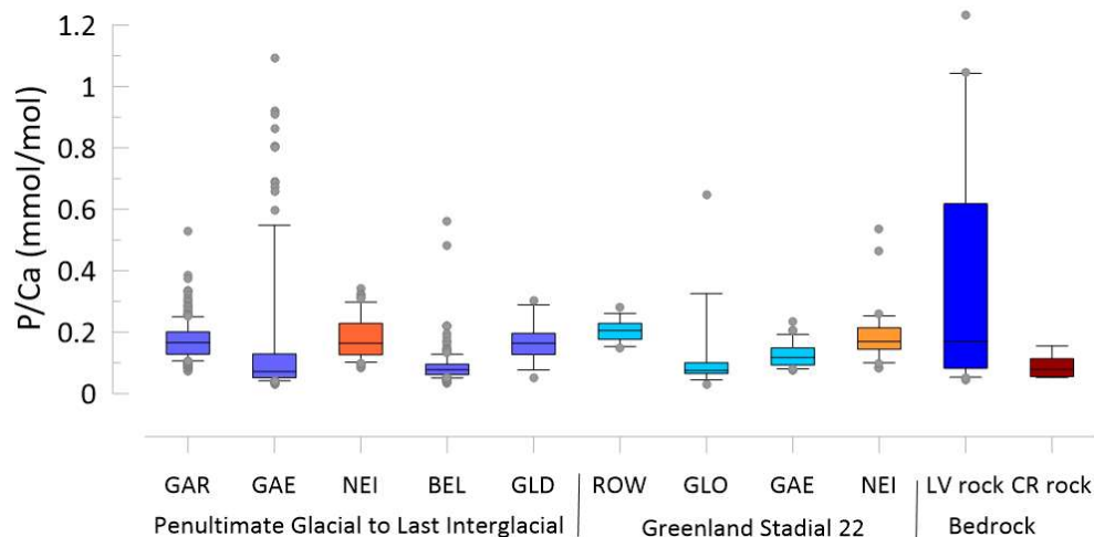
220 Figure 2. Comparison of the range of P/Ca in stalagmites within the 145 to 118 ka time frame and the 92 to 80 ka time frame and in the bedrock from La Vallina (LV) and Cueva Rosa (CR). Line indicates the median, box indicate the 80 th and 20 th percentiles and whiskers indicate the 95 th and 5 th percentiles.
