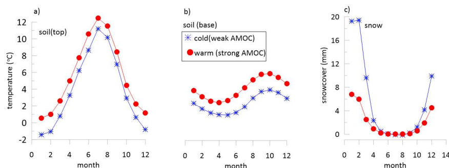
Figure 9. Comparison of monthly simulated soil temperatures and snow cover under simulations of weak AMOC typical of stadial periods and simulations of strong AMOC typical of interstadial periods. Results from simulations of (Romé, 2024; Romé et al., 2022).
