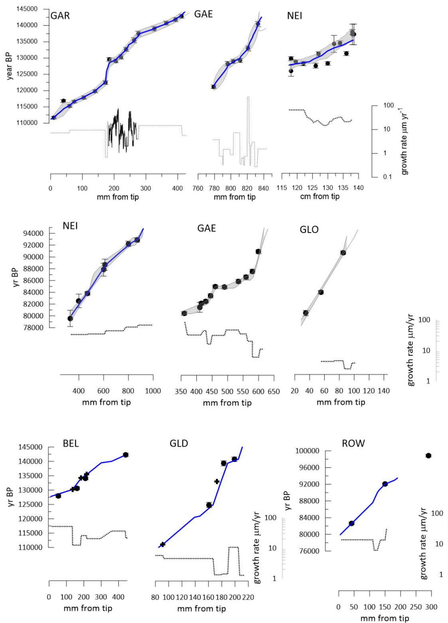
Figure S1. Illustration of age models. Blue lines indicate the employed age model. Gray shading illustrates the 95% confidence intervals for age models generated in BChron in top row, from (Stoll et al., 2022)) and in STALAGE in middle row, from (Stoll et al., 2015). Lower row illustrates age models from (Stoll et al., 2023). Growth rate estimated from the age models is shown in solid line for layer counted segments and dashed line for age models based on U/Th ages and tiepoints. Published U/Th dates are shown as circles with error on age assignments. For the lower row, tiepoints to isotope records in GAR (crosses) are also illustrated.
