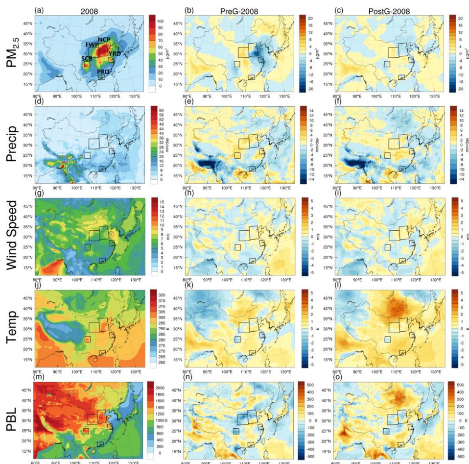
Figure 4. The PM_{2.5} (a–c, \mu g/m^3 ), precipitation (d–f, mm/day), wind speed (g–i, m/s), temperature (j–l, K), and Planetary Boundary Layer (PBL) height (m–o, m) during the EASM period in 2008 (left), and their mean changes due to meteorological variations in PreG (2009–2013, center) and PostG (2014–2018, right) phase relative to 2008, PreG-2008 and PostG-2008 represent the average annual differences between experiments SIM_{Base} and SIM_{MET=2008} ( SIM_{Base} - SIM_{MET=2008} ) for the periods 2009–2013 and 2014–2018, respectively.
