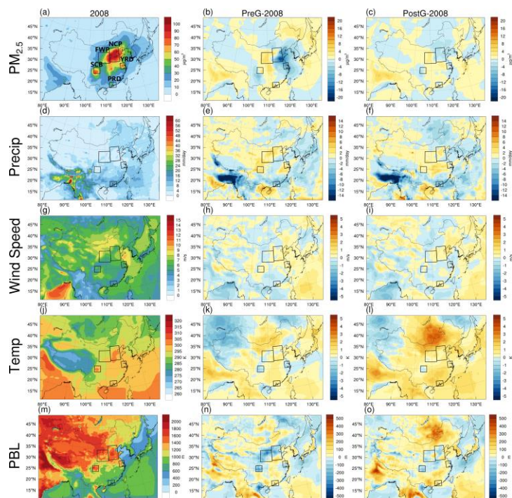
Figure 4. The \text{PM}_{2.5} (a–c, \mu\text{g}/\text{m}^3 ), precipitation (d–f, mm/day), wind speed (g–i, m/s), temperature (j–l, K), and Planetary Boundary Layer (PBL) height (m–o, m) during the EASM period in 2008 (left), and their mean changes due to meteorological variations in PreG (2009–2013, center) and PostG (2014–2018, right) phase relative to 2008 ( \text{SIM}_{\text{Base}} - \text{SIM}_{\text{MET}=2008} ). PreG-2008 and PostG-2008 represent the average annual differences between experiments \text{SIM}_{\text{Base}} and \text{SIM}_{\text{MET}=2008} ( \text{SIM}_{\text{Base}} - \text{SIM}_{\text{MET}=2008} ) for the periods 2009–2013 and 2014–2018, respectively.
