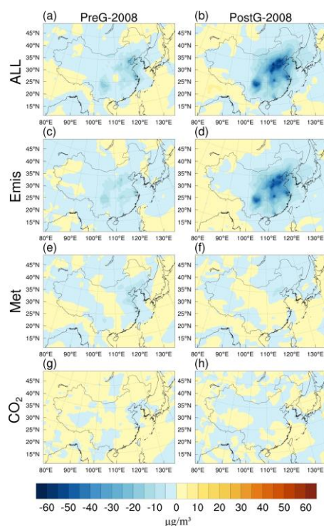
Figure 6. The total changes in \text{PM}_{2.5} concentrations (All, \text{SIM}_{\text{Base}} - \text{SIM}_{2008} ), and the changes in \text{PM}_{2.5} attributed to variations of anthropogenic pollutant emissions (Emis, All-Met- \text{CO}_2 ), meteorological conditions (Met, \text{SIM}_{\text{Base}} - \text{SIM}_{\text{MET}=2008} ), and \text{CO}_2 emissions ( \text{CO}_2 , \text{SIM}_{\text{Base}} - \text{SIM}_{\text{CO}_2=2008} ) during the EASM period in PreG (2009–2013, left) and PostG (2014–2018, right) phase relative to 2008.
