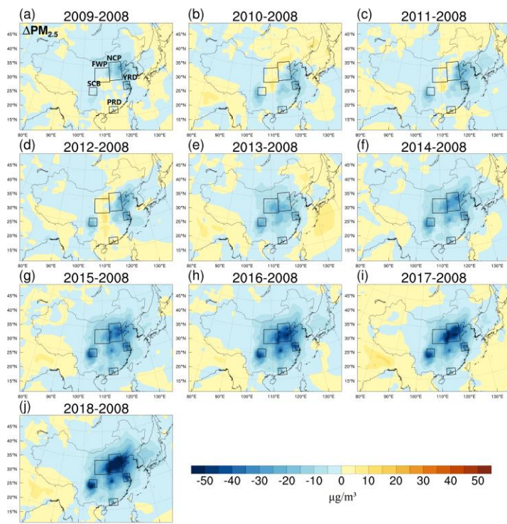
Figure 3. Changes in near-surface \text{PM}_{2.5} concentrations ( \mu\text{g}/\text{m}^3 ) during the EASM period from 2009 (a) to 2018 (j) relative to 2008 in East Asia ( \text{SIM}_{\text{Base}} - \text{SIM}_{2008} ).
