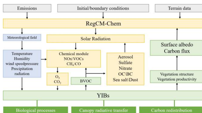
Figure 1. Framework of the RegCM-Chem-YIBs Model.
