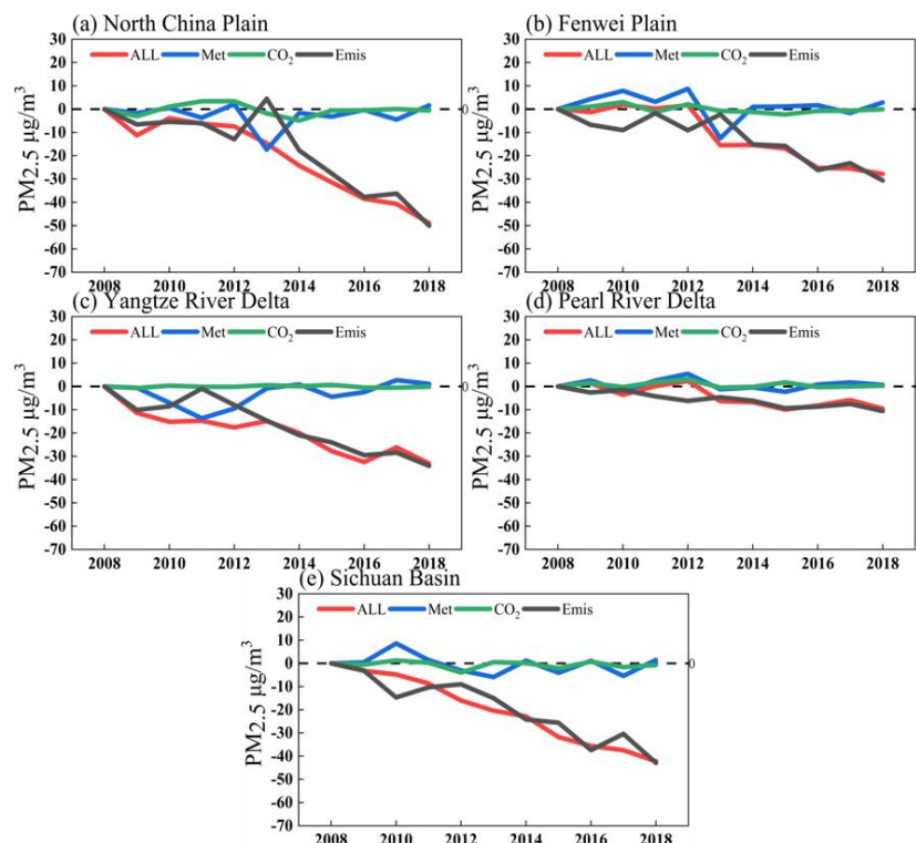
Figure 8. Changes in total \text{PM}_{2.5} concentrations from 2008 to 2018 (ALL, red line) and the contributions of anthropogenic pollutant emissions (Emis, black line), meteorological conditions (Met, blue line), and \text{CO}_2 emission changes ( \text{CO}_2 , green line) to \text{PM}_{2.5} concentrations (Units: \mu\text{g}/\text{m}^3 ).
