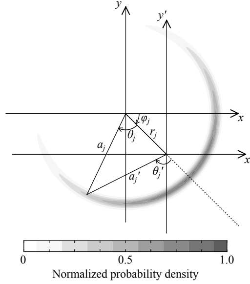
Figure 2. Schematics of variables used in the statistical model and probability density function for individual wave components. x_j + iy_j is (total) complex-valued amplitude; (i.e., its magnitude represents wave amplitude and its angle represents wave phase as the coefficients of complex Fourier series) , x'_j + iy'_j is that with zero mean; and angles are positive clockwise because harmonic analysis conventionally uses phase lags . Shading shows the probability density function of wrapped normal distribution, with narrow Gaussian amplitude spread to make shading discernible. Note that a_j is assumed to be constant, but a'_j varies because of phase distribution. Note also that (a_j, \theta_j) and (a'_j, \theta'_j) are realizations of (A_j, \Theta_j) and (A'_j, \Theta'_j) in Eqs. (1) and (3), respectively. For illustration purposes, \varphi_j = \pi/4 and \sigma_j = 0.3\pi are used.
