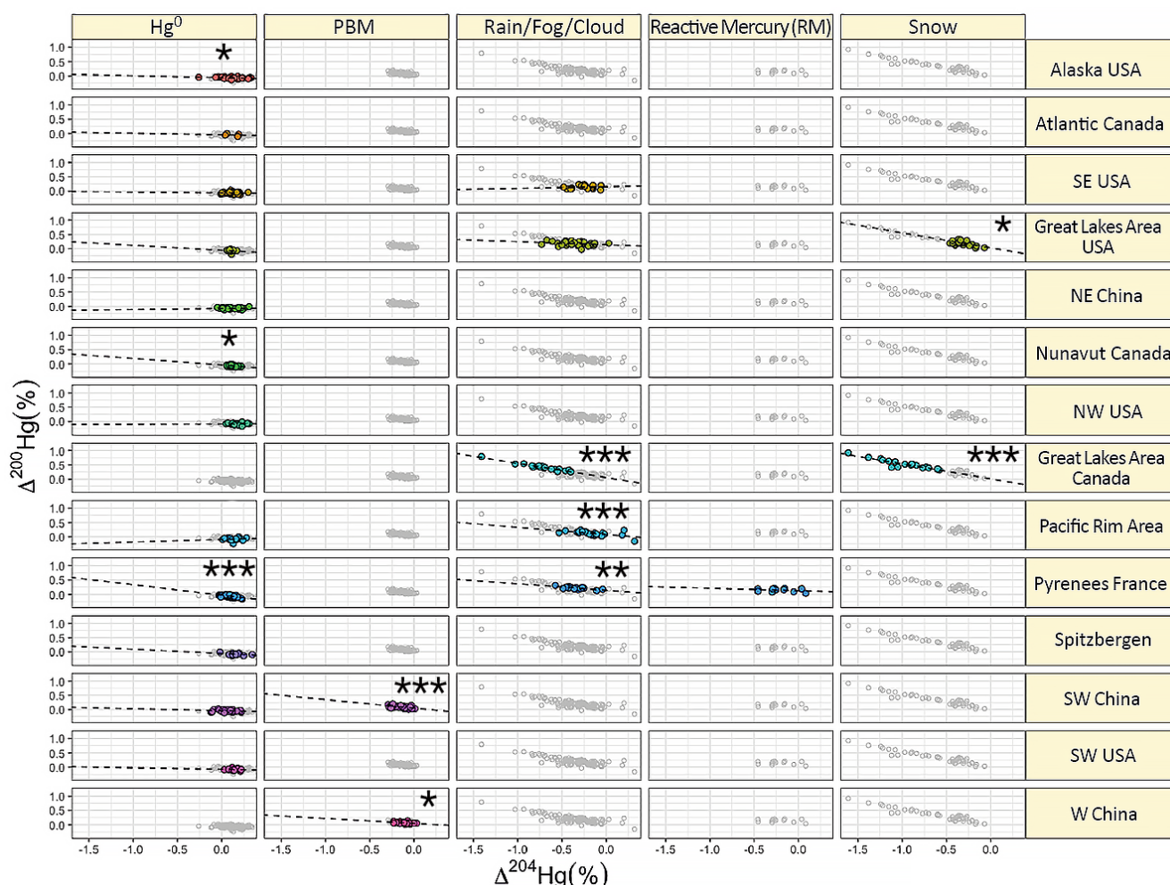
1800 Figure 14. Global observations of even-MIF ( \Delta^{200}\text{Hg} vs. \Delta^{204}\text{Hg} ) by, from left, \text{Hg}^0 , PBM, rain/fog/cloud, reactive mercury (RM), and snow.
