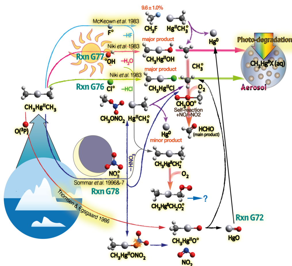
Figure 10. Schematics of the atmospheric fate of DMHg.
