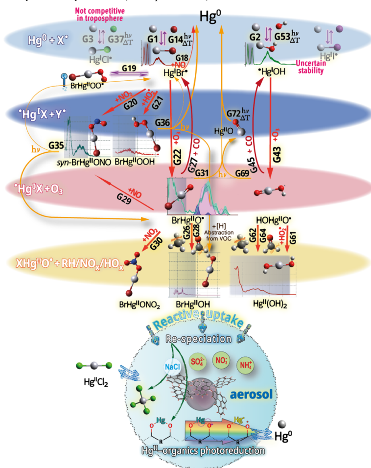
Figure 7. Outline of tropospheric gas-phase Hg chemistry. The reactions of the type \text{Hg} + \text{XO}^\bullet ( \text{X} = \text{O}_2, \text{Br} and \text{NO}_2 ) directly leading to mercuric species are, for the (varying) reasons given in the text, impossible processes in the homogeneous gas phase. In the troposphere, gas-phase oxidation of \text{Hg}^0 in termolecular reactions is initiated by a few radicals in which Br atoms and, with some uncertainty, OH radicals have the
