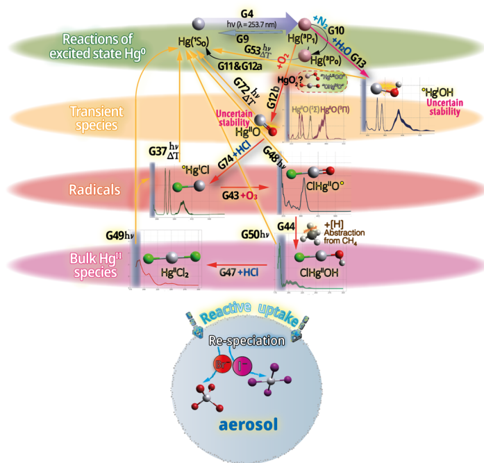
Figure 9. At approximately 35 km, the stratosphere begins to contain actinic radiation, which can electronically excite Hg (at 253.7 nm), but below it is absorbed by O 3 in the Hartley bands (with a maximum at 254 nm). Electronically excited Hg 0 reacts primarily with O 2 , with one of the exit channels leading to the formation of HgO via the intermediate OHg IV O. Before HgO can fully decompose into elements, it reacts further via secondary HCl-driven fast chemistry to HgCl 2 , the major constituent of Hg in the mid-upper stratosphere. A 2:1 steady state between HgCl 2 and Hg 0 occurs because the former photo dissociates more slowly than photosensitized Hg oxidizes, both at significant rates (Saiz-Lopez et al. 2022). The reactive uptake in aerosols, followed by Hg II complexation with the heavier halides, reflects the observed situation in the lower stratosphere (Murphy et al. 1998).
