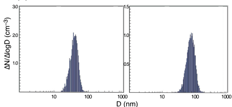
Figure 6. Particle growth of the reaction products from the halogen atom ( \text{X} = \text{Cl}, \text{Br} ) induced oxidation of \text{Hg}^0 vapor studied after the same degree of \text{Hg}^0 conversion ( \sim 75\% , 5–8 ppb) but at different reaction times a and b ( \sim 45 min, \text{Hg}^0 + \text{Br} and \sim 4 h, \text{Hg}^0 + \text{Cl} , respectively). Adopted from Sun et al. (2016).
