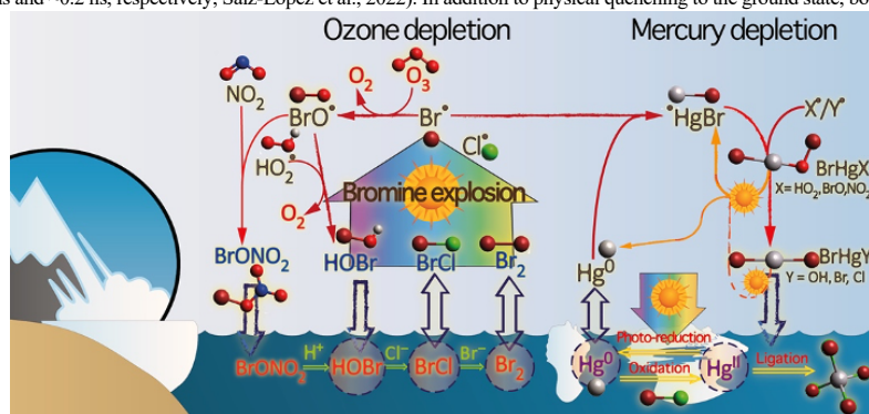
345 Figure 2. The chemistry behind bromine explosion events and related surface layer ozone and mercury depletion events.
