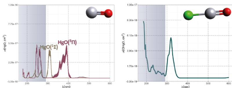
Figure 5. Computed absorption spectra of (a) HgO (lowlying 3 Π and 1 Σ states) and (b) ClHgO radical (Saiz-Lopez et al., 2018; Saiz-Lopez et al., 2022). Wavelengths accessible in the troposphere are to the right of the colored area.
