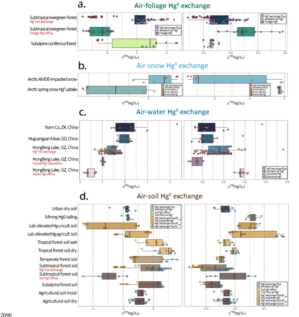
Figure 18. Statistical summary of observations from isotopic studies of Hg^0 exchange between the atmosphere and various groups of surface reservoirs on Earth. In the air-foliage group, data were taken from Yuan et al. (2019b) and Chen et al. (2023). For the air-snow group, data were taken from Sherman et al. (2010) and Douglas and Blum (2019). For the air-water group, data were taken from Zhang et al. (2023a; 2021a). For the air-soil group, data were taken from Zhang et al. (2020), Zhu et al. (2022), Yuan et al. (2021; 2023b) and Chen et al. (2023).
