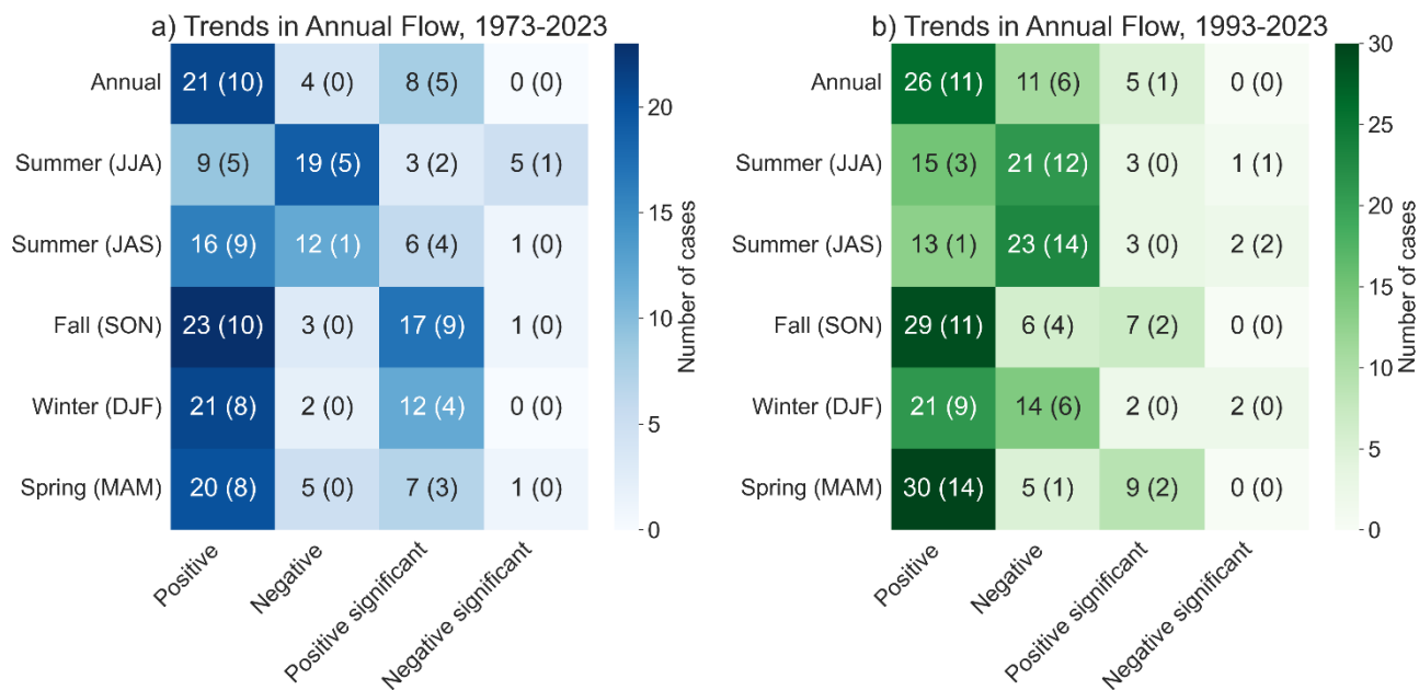
455 Figure 8: Heatmaps showing a summary of the results from analysis of annual and seasonal trends in streamflow for the periods 1973-2023 (a) and 1993-2023 (b). The numbers in parentheses indicate the count of catchments with more than 5% glaciation. Note that for the period 1973-2023, the 17 significant positive SON trends include two from the same glacial river (Jökulsá á Fjöllum river).
