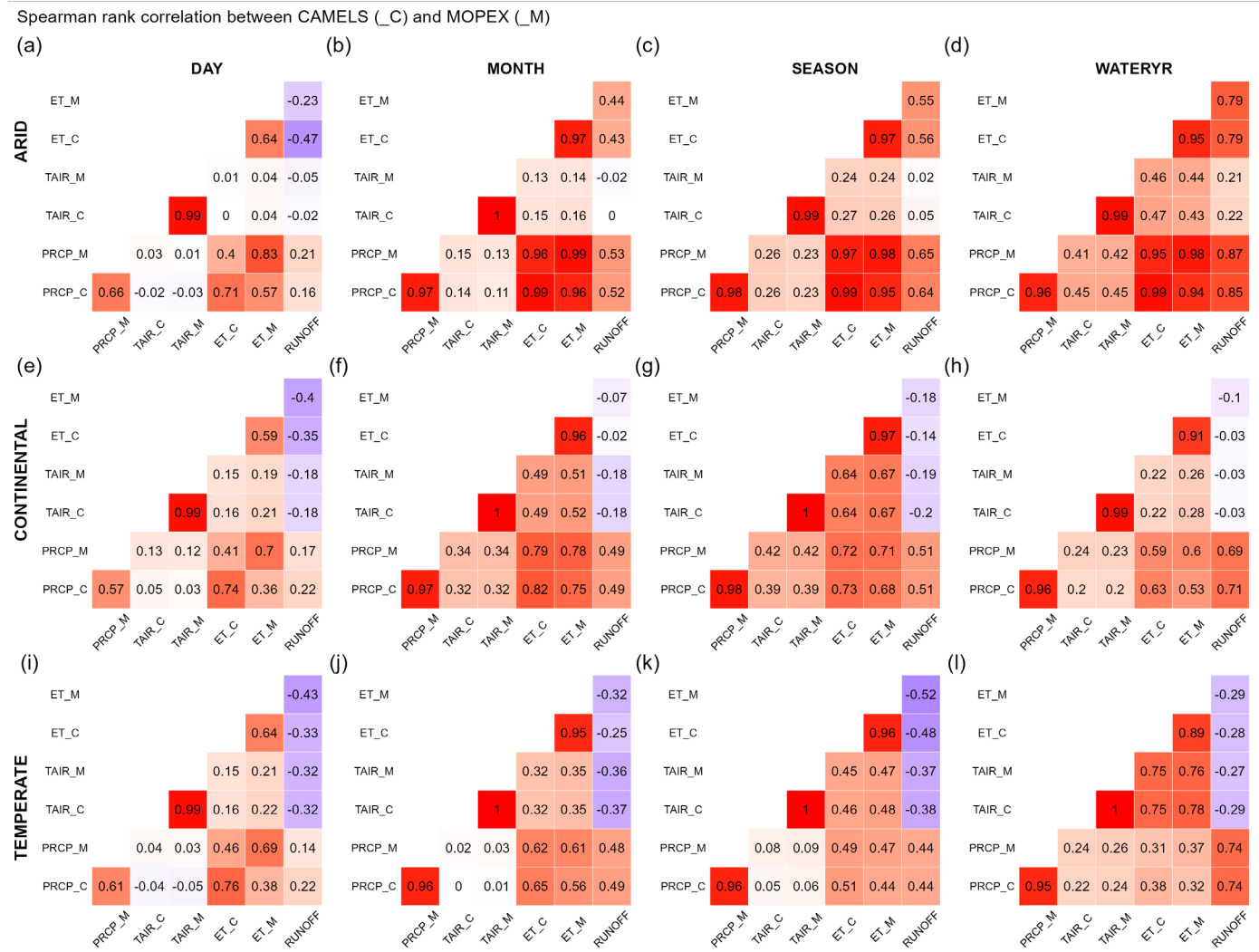
Figure 22. Spearman rank correlation values between CAMELS ( \_C ) and MOPEX ( \_M ) datasets for precipitation (PRCP) in millimeters, temperature (TAIR) in degrees Celsius, and water balance calculated evapotranspiration (ET) in millimeters. Runoff, in millimeters, represents both datasets. Arid correlations are between (a) daily values, (b) monthly values, (c) seasonal values, and (d) annual water year values. Continental correlations are between (e) daily values, (f) monthly values, (g) seasonal values, and (h) annual water year values. Temperate correlations are between (i) daily values, (j) monthly values, (k) seasonal values, and (l) annual water year values.
