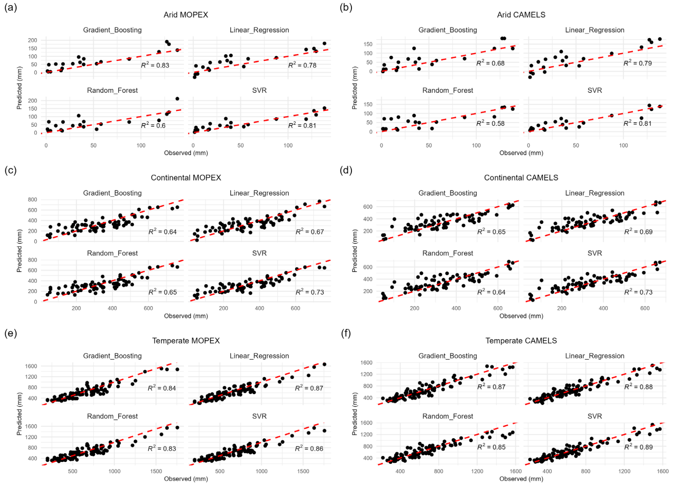
Figure 27. Observed versus predicted total annual runoff (mm) for each ML model and each climate region. The dashed red line represents the 1:1 reference line. MOPEX correlations are (a) arid, (c) continental, and (e) temperate. CAMELS correlations are (b) arid, (d) continental, and (f) temperate.
