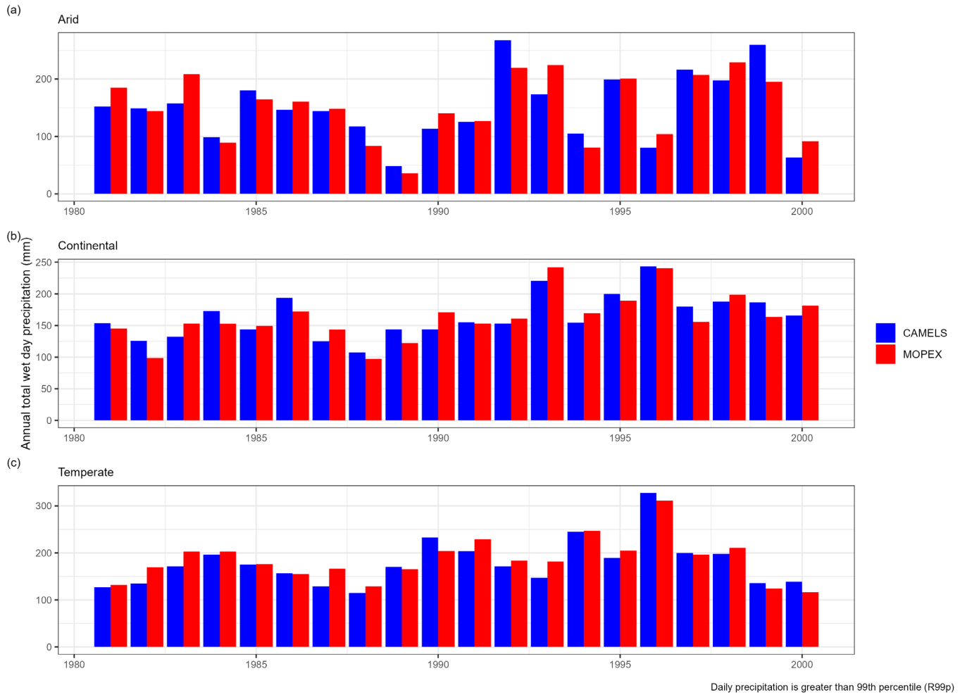
Figure 25. Annual total precipitation when daily precipitation amount on a wet day ( \geq 1\text{mm} ) is greater than the 99th percentile for a) arid, b) continental, and c) temperate regions. Colors (blue and red) represent the dataset.
