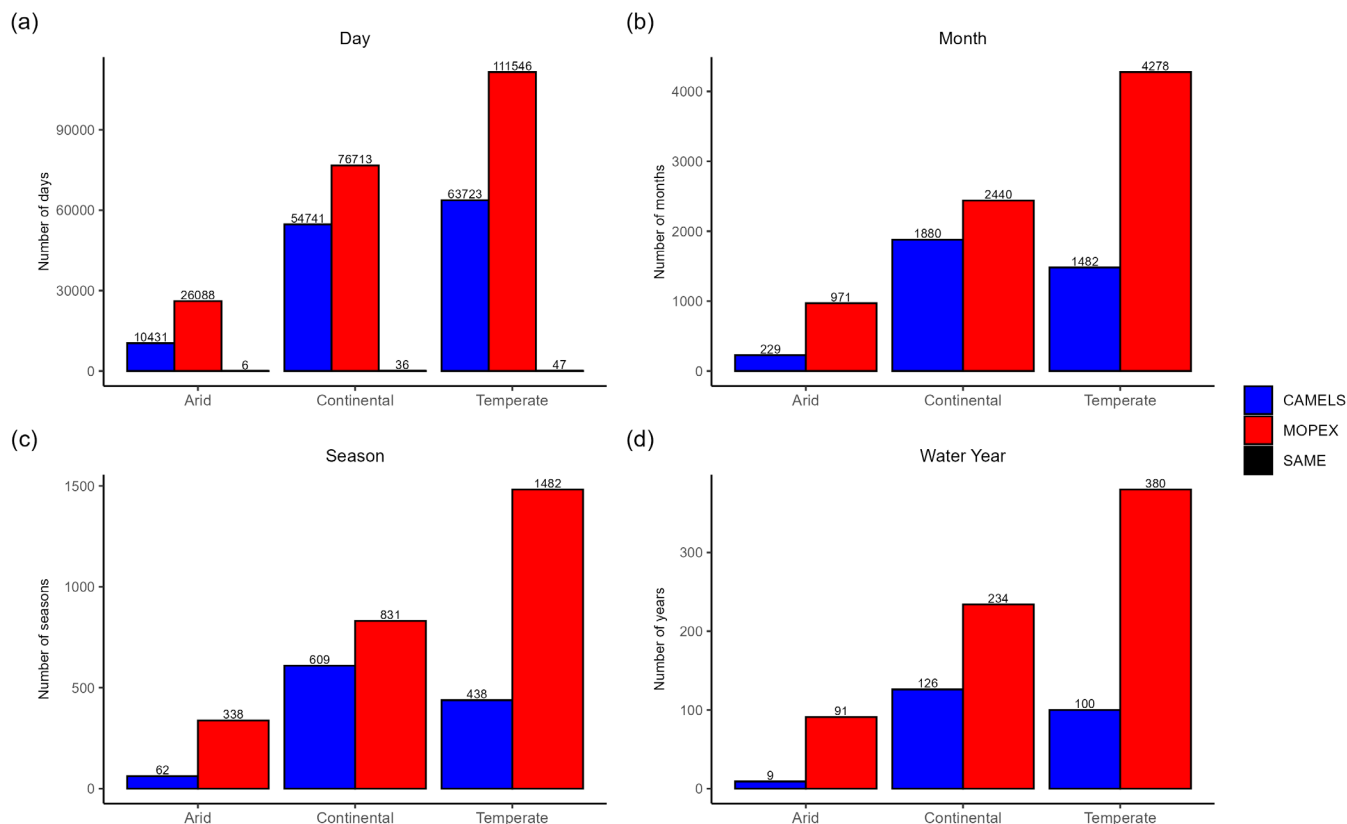
Figure 14. Sign tally results from non-parametric binomial sign for (a) daily, (b) monthly, (c) seasonal, and (d) annual temperature values. Counts on the y-axis reflect the number of basins (gauges) within each climate region times the number of temporal periods. All results are based on CAMELS minus MOPEX values. Positive values (CAMELS) indicate that CAMELS > MOPEX (blue bars), negative (MOPEX) values indicate MOPEX > CAMELS (red bars), and zero (SAME) indicate that CAMELS = MOPEX (black bars).
