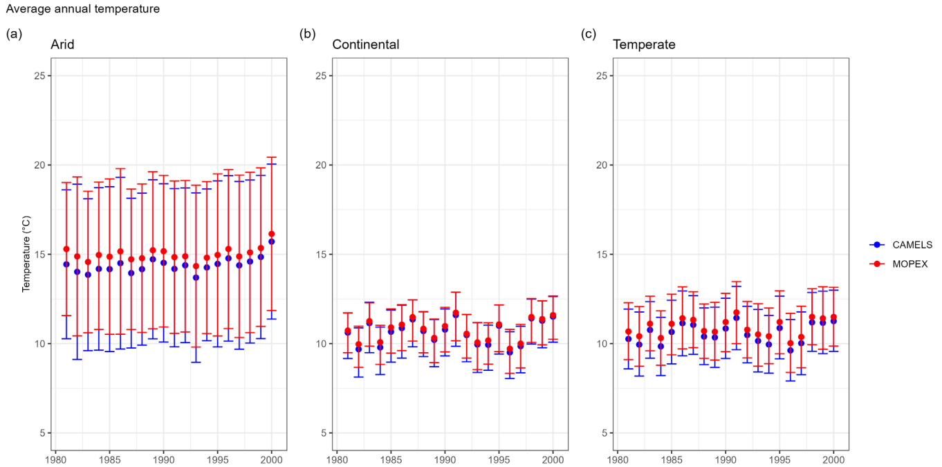
Figure 12. Average annual temperature for CAMELS (blue) and MOPEX (red) by (a) arid, (b) continental, and (c) temperate climate region in degrees Celsius. The mean value is determined using all basins within the climate region and each corresponding water year for 1981-2000. Error bars represent two-sided 95 % confidence intervals, derived from bootstrapping with replacement for 10,000 replicates.
