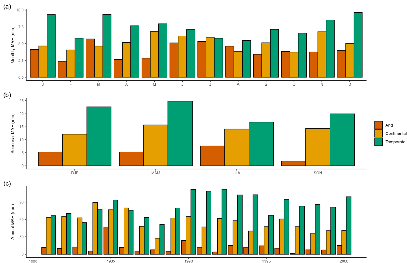
Precipitation mean absolute error
