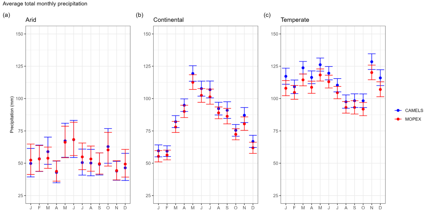
Figure 7. Average total monthly precipitation for CAMELS (blue) and MOPEX (red) by (a) arid, (b) continental, and (c) temperate climate region in millimeters. The mean value is determined using all basins within the climate region and each corresponding month for 1981-2000. Error bars represent two-sided 95 % confidence intervals, derived from bootstrapping with replacement for 10,000 replicates.
