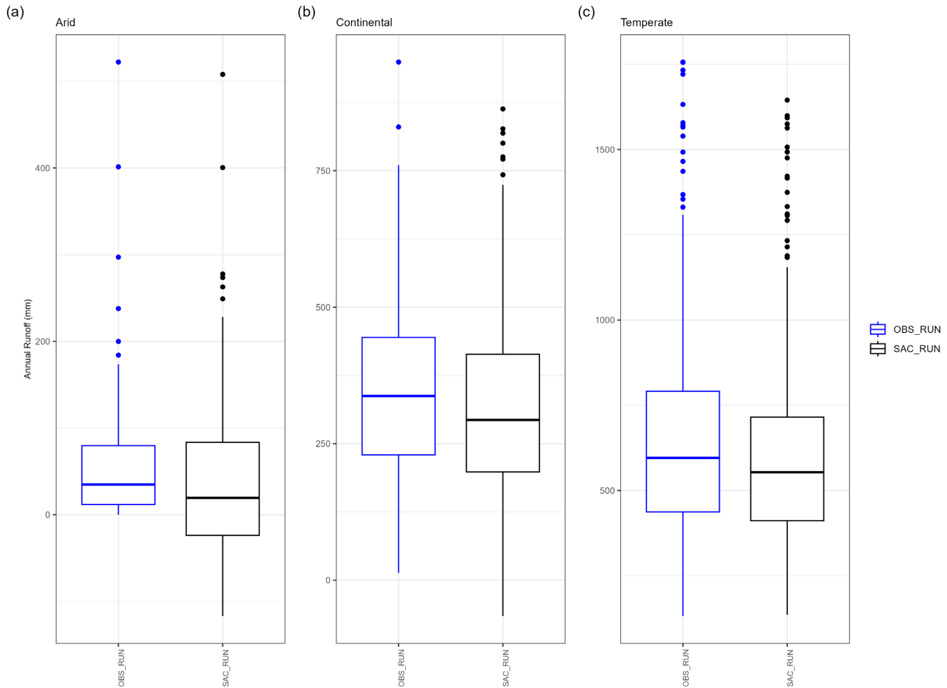
Figure 4. Total annual runoff for (a) arid, (b) continental, and (c) temperate regions. The boxplots represent the annual totals for all basins in a region, with measured observed runoff (OBS_RUN, blue) and water balance calculated runoff (PRCP minus ET) using CAMELS SAC-SMA model output ET (SAC_RUN, black).
