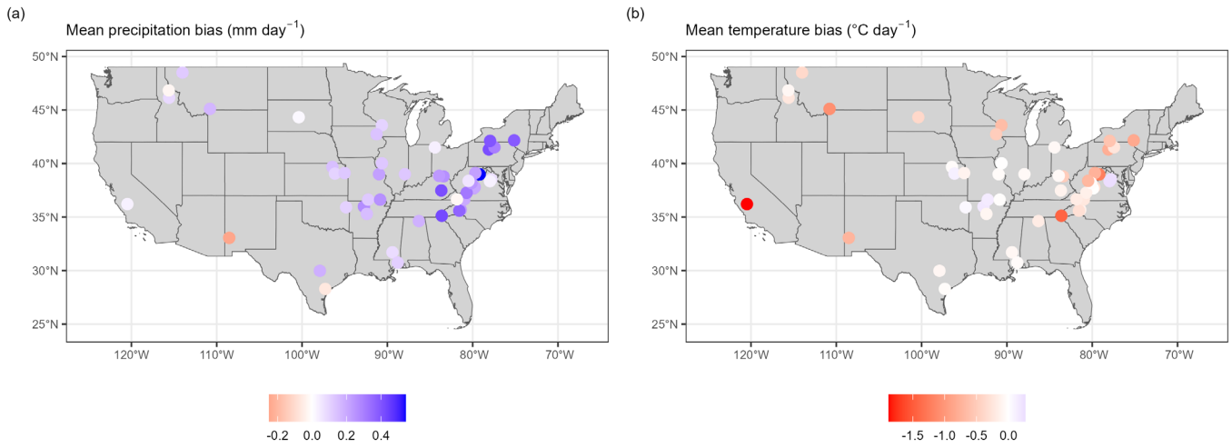
Figure 19. Overall bias for (a) mean precipitation at each gauge location based on CAMELS minus MOPEX. Color bar represents bias in millimeters per day where negative values (red) indicate a MOPEX wet bias and positive values (blue) indicate a CAMELS wet bias. Overall bias for (b) mean temperature at each gauge location based on CAMELS minus MOPEX. Color bar represents bias in degrees Celsius per day where negative values (red) indicate a MOPEX warm bias and positive values (blue) indicate a CAMELS warm bias.
