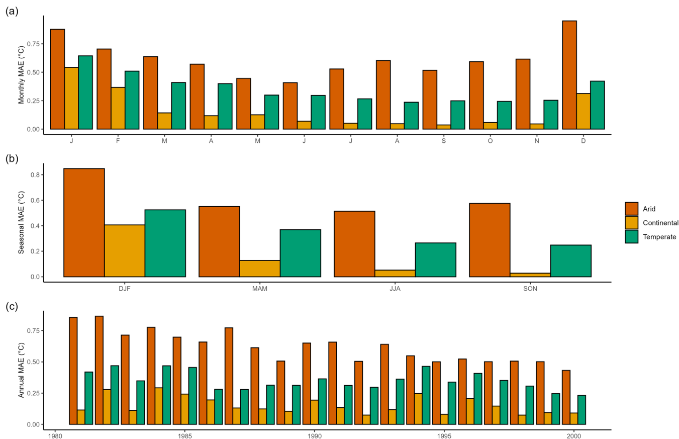
Figure 21. Mean absolute error for (a) monthly, (b) seasonal, and (c) annual temperature in degrees Celsius. MAE is based on means between all basins within a climate region (arid, continental, and temperate).
