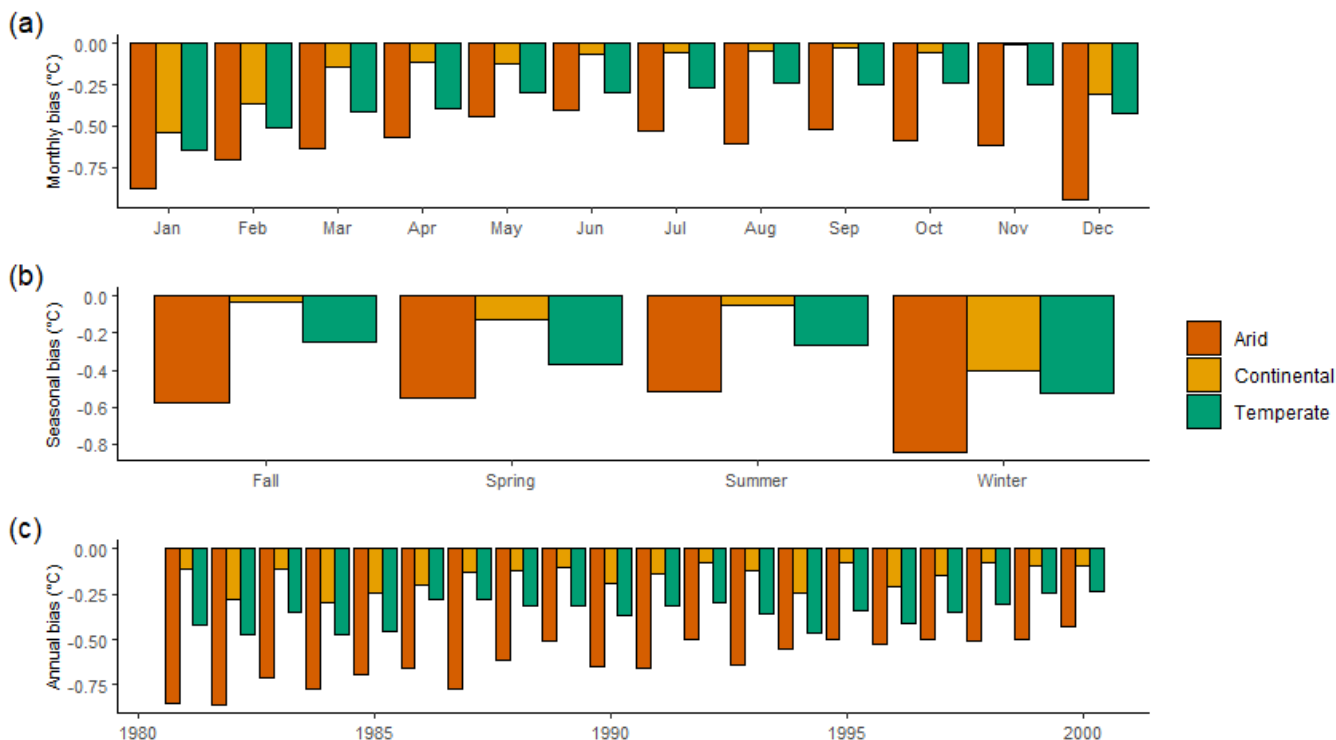
Figure 18. Magnitude of temperature bias averaged over all watersheds in a climate region (arid, continental, and temperate) based on a) monthly, b) seasonal, and c) annual totals. All differences are CAMELS minus MOPEX values. Positive bias indicates CAMELS > MOPEX while negative bias indicates MOPEX > CAMELS.
