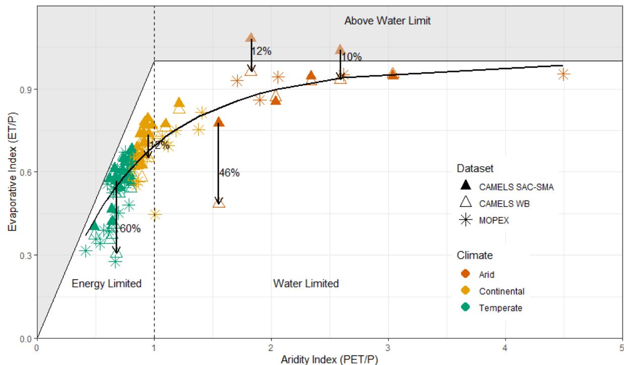
Figure 5. Budyko diagram with the aridity and evaporative indices plotted for each of the 47 catchments (1981–2000). The overall aridity index and evaporative index is plotted for each catchment for the three ET values, resulting in 141 points. The three ET values include MOPEX (asterisk), CAMELS (solid triangle) with SAC-SMA derived ET, and CAMELS WB (open triangle) with water balance calculated evapotranspiration. Evaporative index values > 1 are non-physical.
