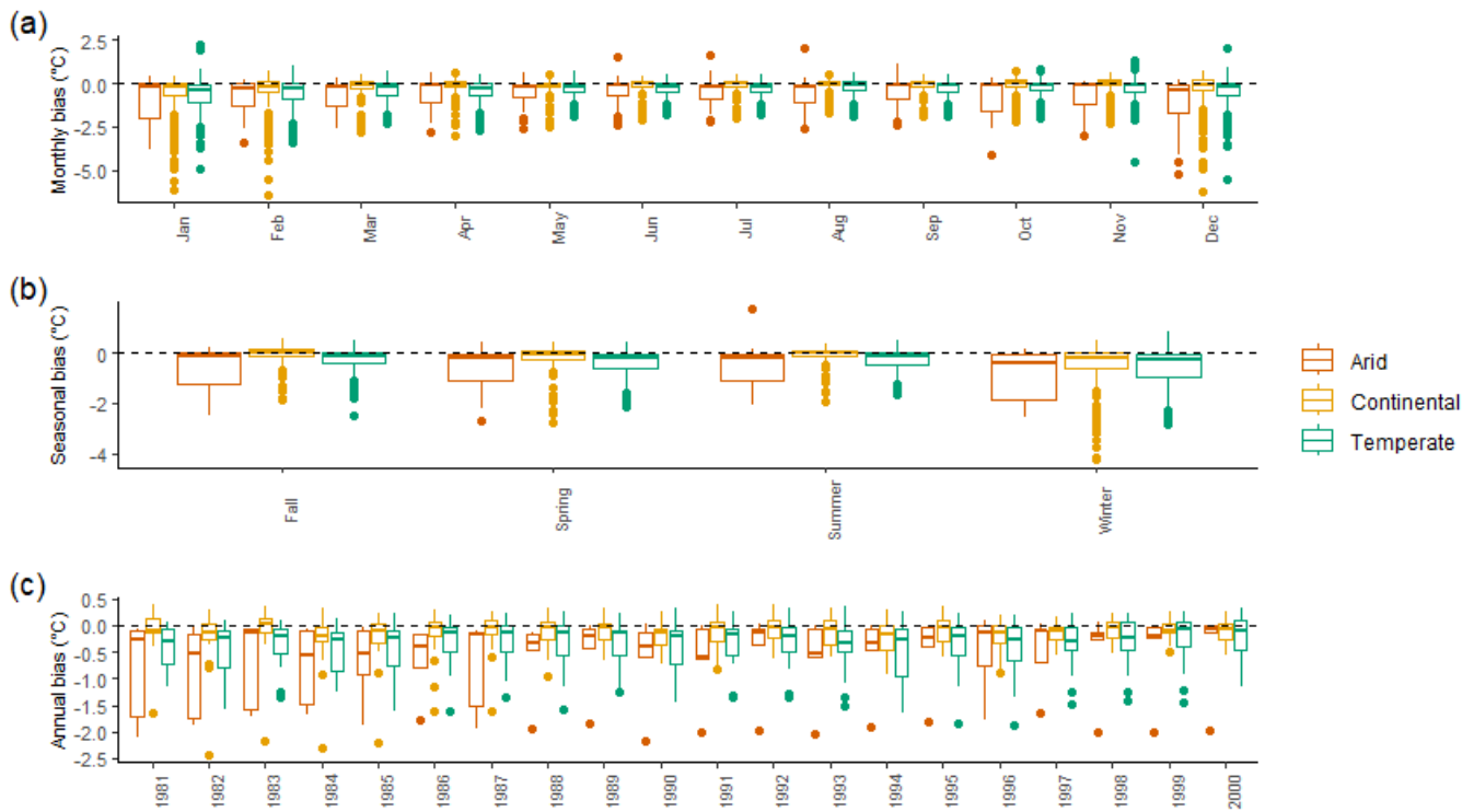
Figure 16. Monthly (a), seasonal (b), and annual (c) temperature biases. All basins are combined by climate region (arid, continental, and temperate) and box plots represent the number of observations indicated in Table 3. Temperature biases are based on mean values of CAMELS minus MOPEX. Positive values indicate CAMELS > MOPEX and negative values indicate MOPEX > CAMELS.
