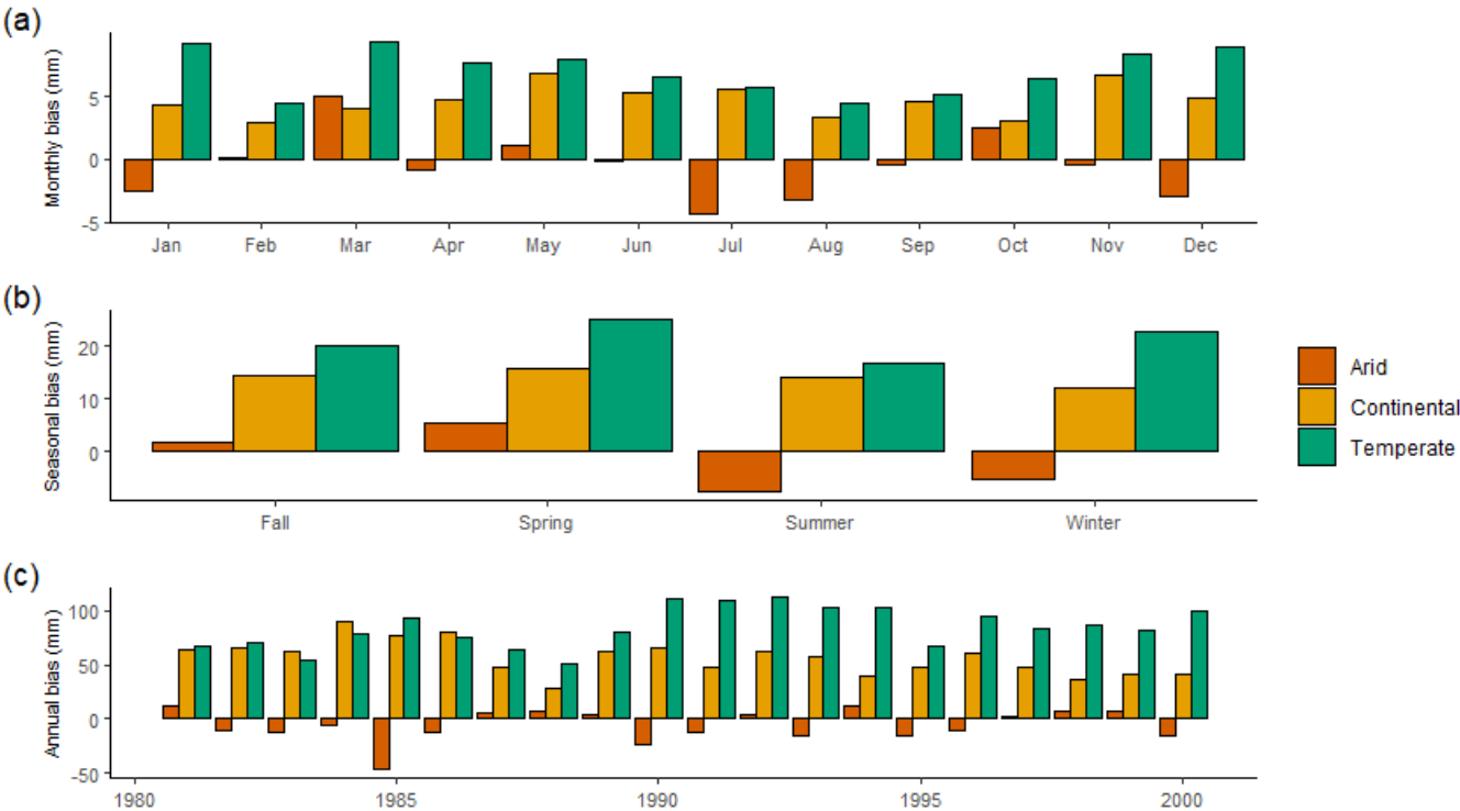
Figure 17. Magnitude of precipitation bias averaged over all watersheds in a climate region (arid, continental, and temperate) based on a) monthly, b) seasonal, and c) annual totals. All differences are CAMELS minus MOPEX values. Positive bias indicates CAMELS > MOPEX while negative bias indicates MOPEX > CAMELS.
