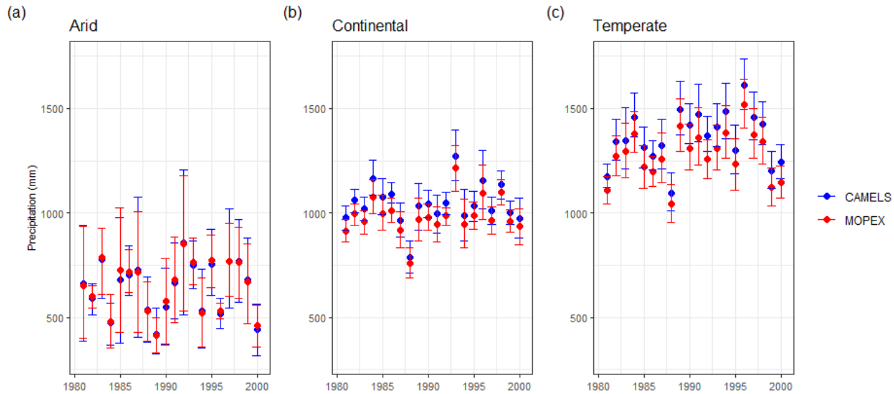
Figure 9. Average total annual precipitation for CAMELS (blue) and MOPEX (red) by a) arid, b) continental, and c) temperate climate region. The mean value is determined using all basins within the climate region and each corresponding water year for 1981-2000. Error bars represent two-sided 95 % confidence interval, derived from bootstrapping with replacement for 10,000 replicates.
