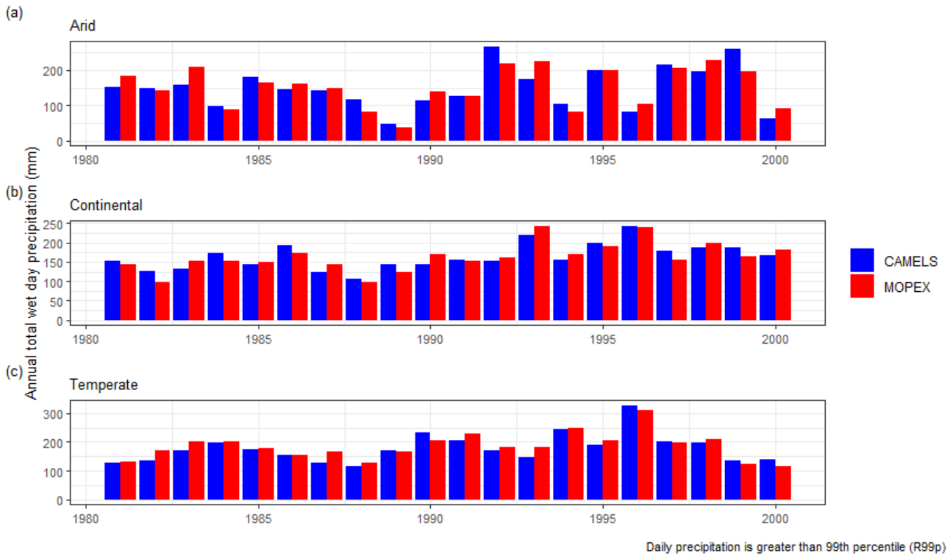
Figure 25. Annual total precipitation when daily precipitation amount on a wet day ( \geq 1\text{mm} ) is greater than the 99th percentile for a) arid, b) continental, and c) temperate regions. Colors (blue and red) represent the dataset.
