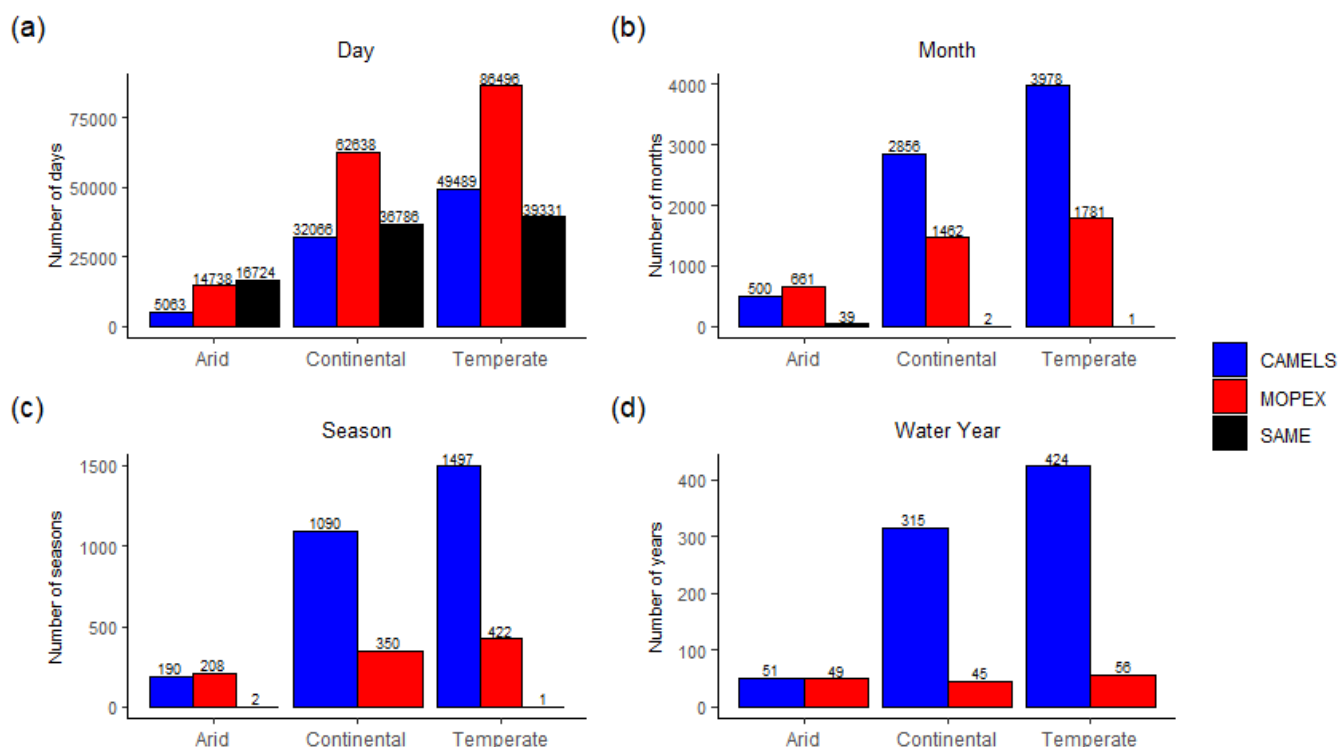
Figure 13. Sign tally results from non-parametric binomial sign test for a) daily, b) monthly, c) seasonal, and d) annual precipitation values. Counts on the y-axis reflect the number of basins (gauges) within each climate region times the number of temporal periods. All results are based on CAMELS minus MOPEX values. Positive values (CAMELS) indicate that CAMELS > MOPEX (blue bars), negative (MOPEX) values indicate MOPEX > CAMELS (red bars), and zero (SAME) indicate that CAMELS = MOPEX (black bars).
