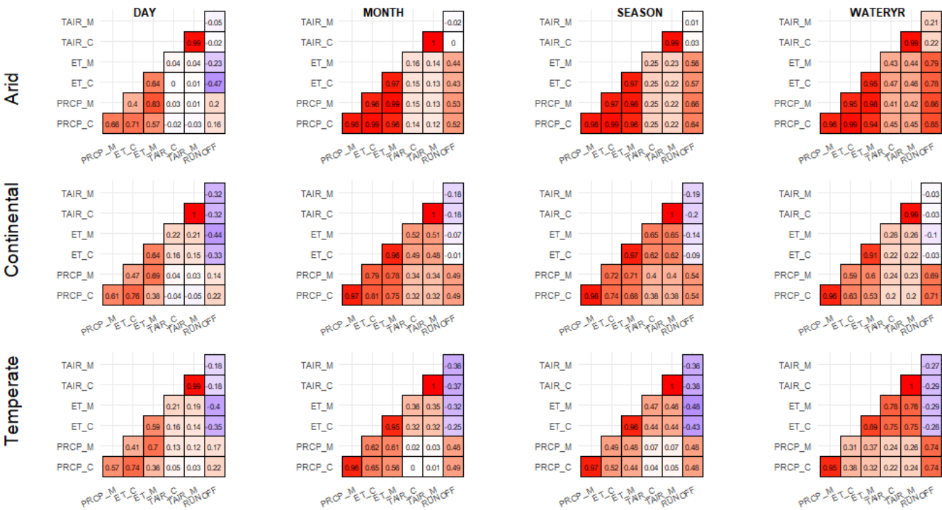
Figure 22. Spearman rank correlation values between CAMELS (_C) and MOPEX (_M) datasets for precipitation, temperature, and water balance calculated evapotranspiration. Runoff represents both datasets.
