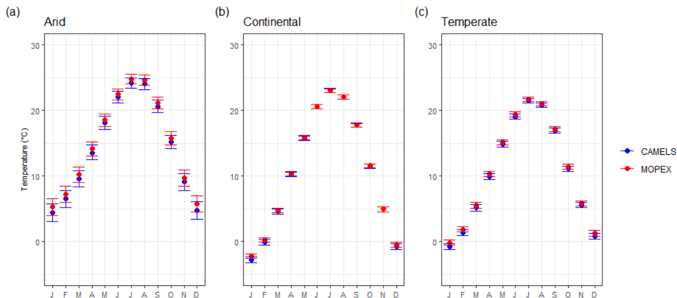
515 Figure 10. Average monthly mean temperature for CAMELS (blue) and MOPEX (red) by a) arid, b) continental, and c) temperate climate region. The mean value is determined using all basins within the climate region and each corresponding month for 1981-2000. Error bars represent two-sided 95 % confidence interval, derived from bootstrapping with replacement for 10,000 replicates.
