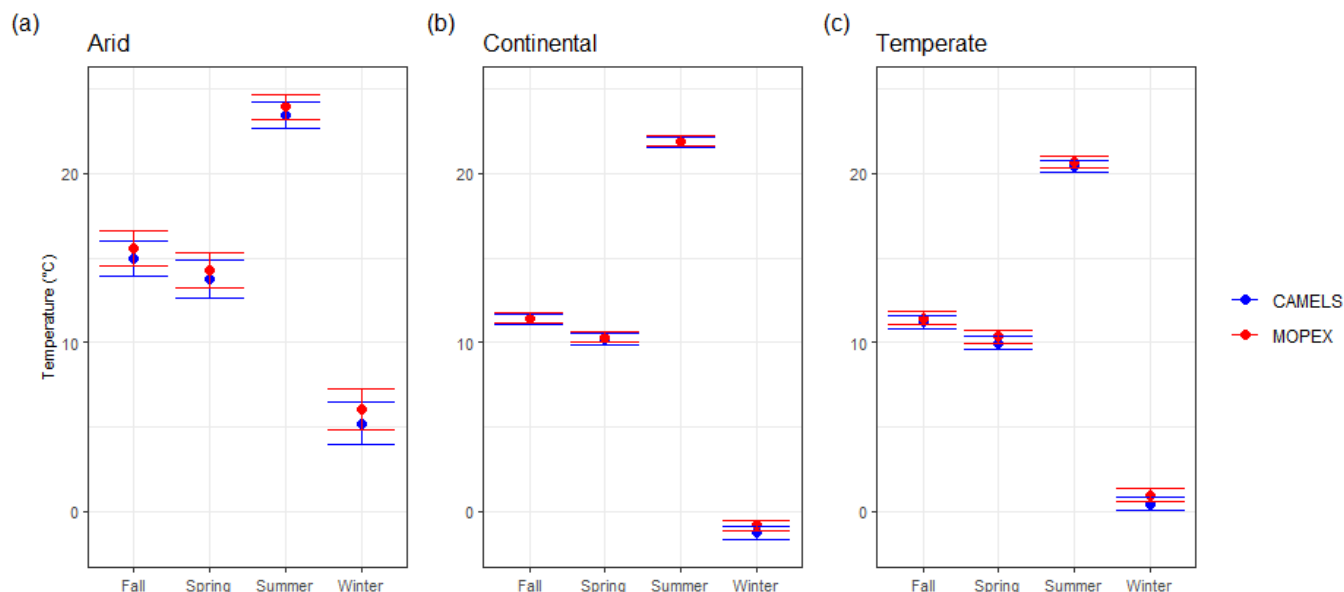
525 Figure 11. Average mean seasonal temperature for CAMELS (blue) and MOPEX (red) by a) arid, b) continental, and c) temperate climate region. The mean value is determined using all basins within the climate region and each corresponding season for 1981-2000. Error bars represent two-sided 95 % confidence interval, derived from bootstrapping with replacement for 10,000 replicates.
