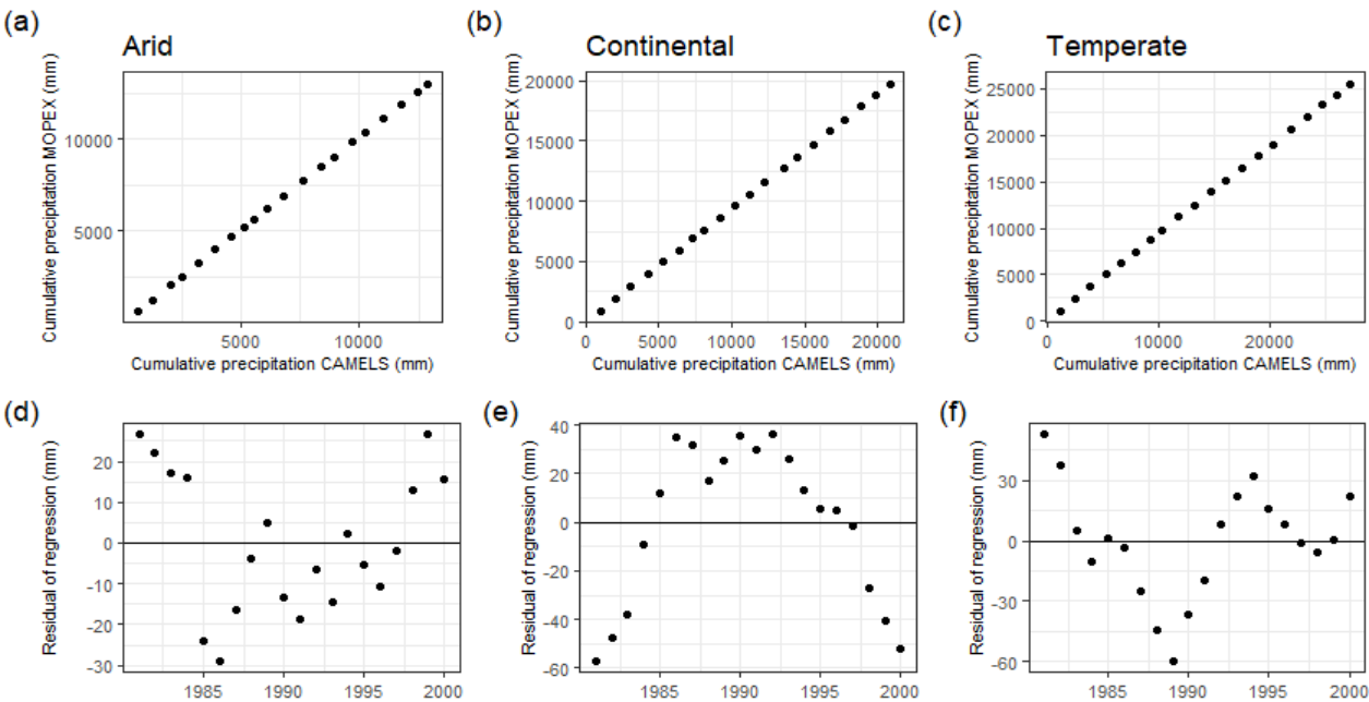
Figure 28. Cumulative annual precipitation of CAMELS versus MOPEX for each climate region a) arid, b) continental, c) temperate for all water years 1981 – 2000. Residuals of regression are shown for each double mass curve d) arid, e) continental, f) temperate.
