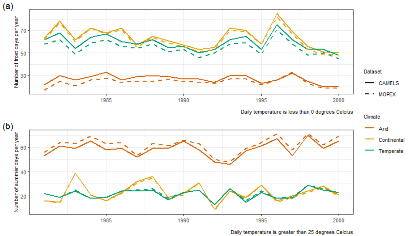
Figure 26. Temperature indices which show the a) annual count of frost days where temperature is < 0^{\circ}\text{C} and b) annual count of summer days where temperature is > 25^{\circ}\text{C} . Colors represent the climate region (arid, continental, and temperate), dashed lines represent MOPEX, and solid lines represent CAMELS.
