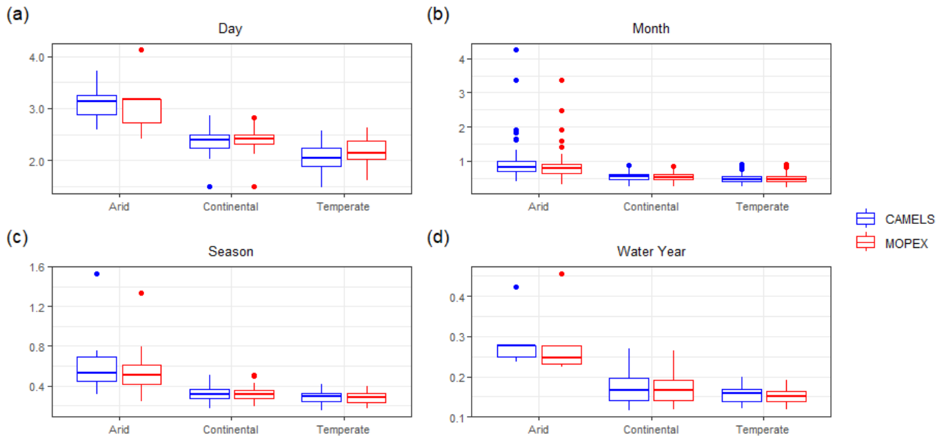
Figure 6. Coefficient of variation of precipitation for CAMELS (blue) and MOPEX (red) for each climate region, shown by temporal aggregation a) day, b) month, c) season, and d) water year. Each boxplot represents the value of all basins within the climate region based on total precipitation (mm). Note progressively declining y-axis range from (a) to (d).
