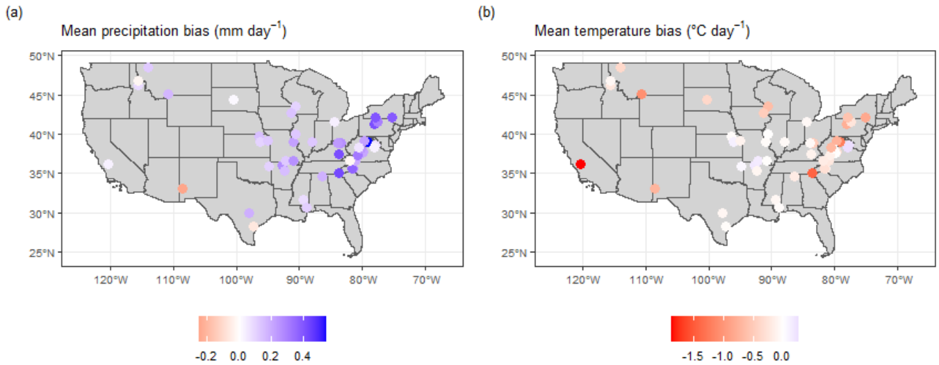
Figure 19. Overall bias for a) mean precipitation at each gauge location based on CAMELS minus MOPEX. Color bar represents bias in mm per day where negative values (red) indicate a MOPEX bias and positive values (blue) indicate a CAMELS wet bias. Overall bias for b) mean temperature at each gauge location based on CAMELS minus MOPEX. Color bar represents bias in degrees Celsius per day where negative values (red) indicate a MOPEX bias and positive values (blue) indicate a CAMELS warm bias.
