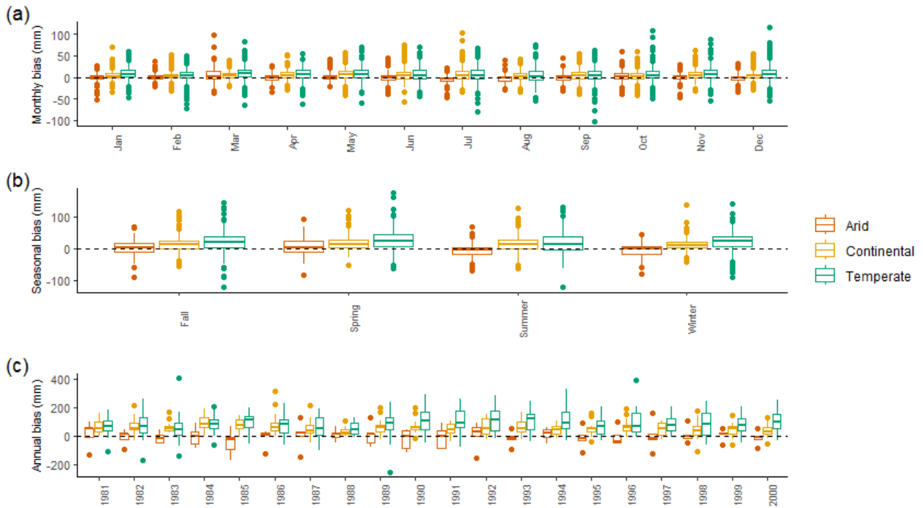
Figure 15. Monthly (a), seasonal (b), and annual (c) precipitation biases. All basins are combined by climate region (arid, continental, and temperate) and box plots represent the number of observations indicated in Table 3. Precipitation biases are based on total values of CAMELS minus MOPEX. Positive values indicate CAMELS > MOPEX and negative values indicate MOPEX > CAMELS.
