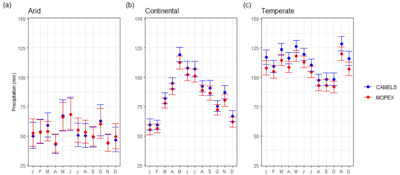
Figure 7. Average total monthly precipitation for CAMELS (blue) and MOPEX (red) by a) arid, b) continental, and c) temperate climate region. The mean value is determined using all basins within the climate region and each corresponding month for 1981-2000. Error bars represent two-sided 95 % confidence interval, derived from bootstrapping with replacement for 10,000 replicates.
