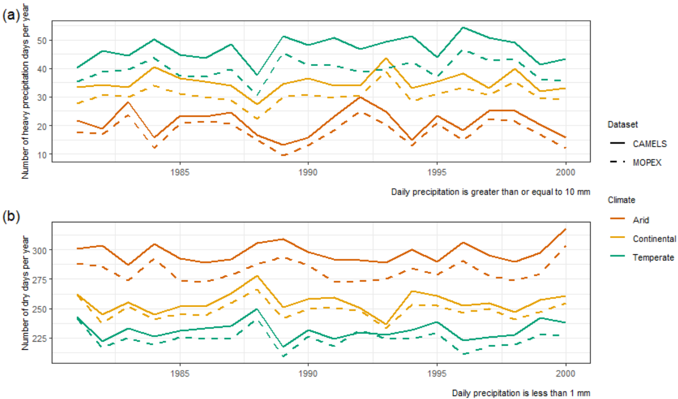
810 Figure 24. Precipitation indices which show the a) annual count of heavy precipitation days where precipitation is \geq 10 mm and b) annual 815 count of dry days where precipitation amount is < 1 mm. Colors represent the climate region (arid, continental, and temperate), dashed lines represent MOPEX, and solid lines represent CAMELS.
