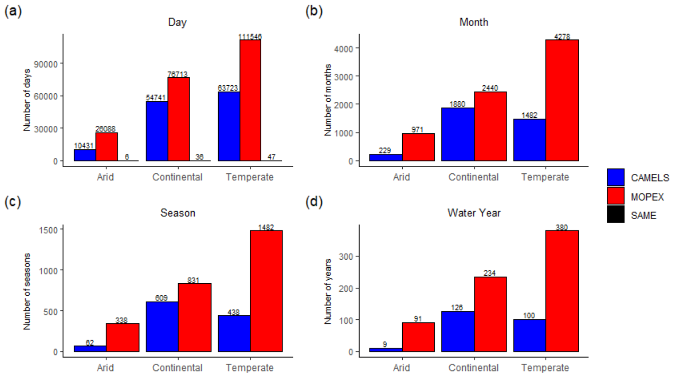
Figure 14. Sign tally results from non-parametric binomial sign for a) daily, b) monthly, c) seasonal, and d) annual temperature values. Counts on the y-axis reflect the number of basins (gauges) within each climate region times the number of temporal periods. All results are based on CAMELS minus MOPEX values. Positive values (CAMELS) indicate that CAMELS > MOPEX (blue bars), negative (MOPEX) values indicate MOPEX > CAMELS (red bars), and zero (SAME) indicate that CAMELS = MOPEX (black bars).
