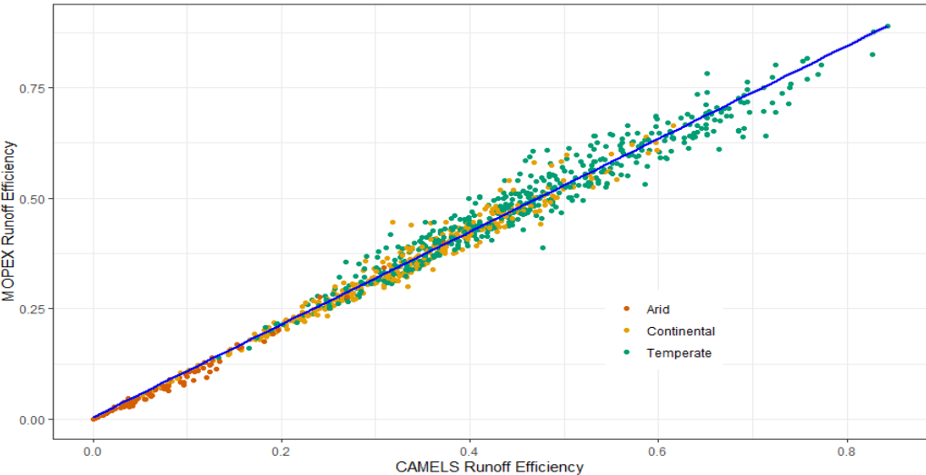
Figure 23. Annual runoff coefficient (runoff/precipitation) for each basin. Colored points represent climate region (arid, continental, and temperate). The blue line indicates the best linear fit.
