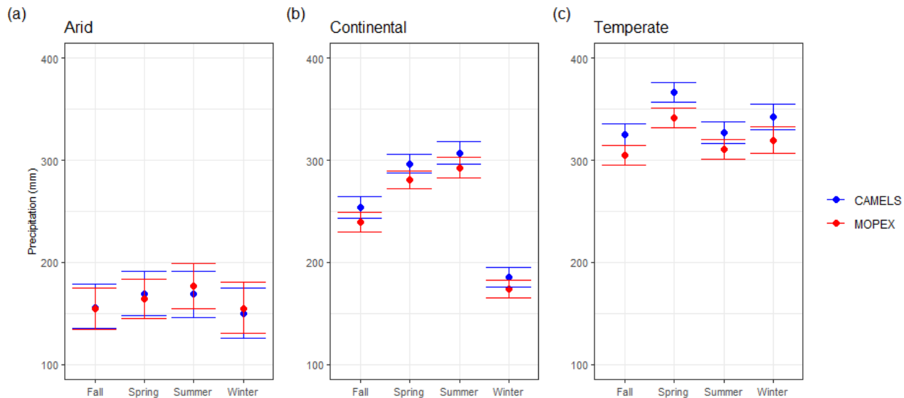
Figure 8. Average total seasonal precipitation for CAMELS (blue) and MOPEX (red) by a) arid, b) continental, and c) temperate climate region. The mean value is determined using all basins within the climate region and each corresponding season for 1981-2000. Error bars represent two-sided 95 % confidence interval, derived from bootstrapping with replacement for 10,000 replicates.
