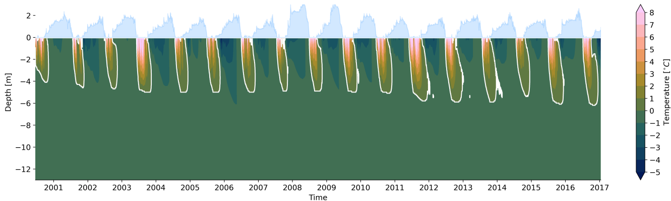
Figure 2. Time series of daily averaged modelled ground temperatures during natural undisturbed conditions at the Schilthorn site from 2000 to 2017. White contours indicate the 0 °C isotherm, i.e, the ALT. Snow depth is indicated in light blue above the 0 m depth level.
