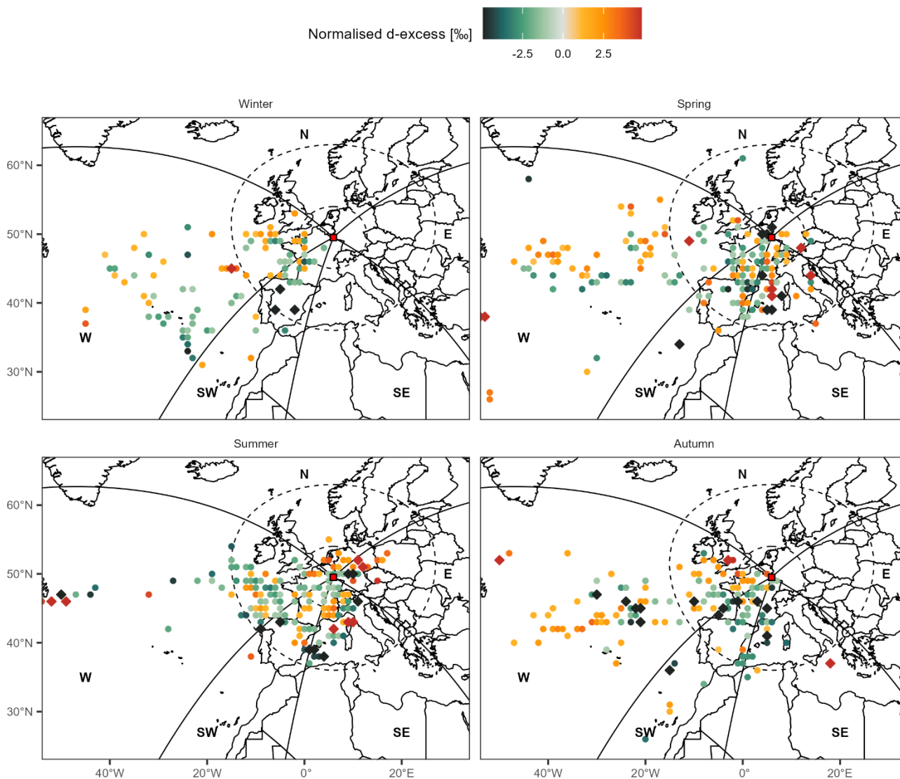
345 Figure 7: Maps of normalised precipitation d-excess values at the study site ( N = 847 ) based on the air moisture contributing areas (Fig. 3). Only moisture uptake locations contributing to more than 0.1 percent of the total seasonal uptake are shown. The colour of the points represents the mean (precipitation amount weighted) normalised precipitation d-excess (using 30-day running mean windows) of all trajectories carrying moisture from that specific location (i.e., cell of 1^\circ by 1^\circ raster). It is important to note that these are precipitation d-excess values from the sampling site marked by a red square, not the d-excess at the moisture origin. Moisture uptake locations with normalised precipitation d-excess between -1.0\% and 1.0\% are not shown, while moisture uptake locations with normalised precipitation d-excess below -5.0\% are marked with black diamonds and above 5.0\% with red diamonds. 350 The location of the sampling site is indicated with a red rectangle.
