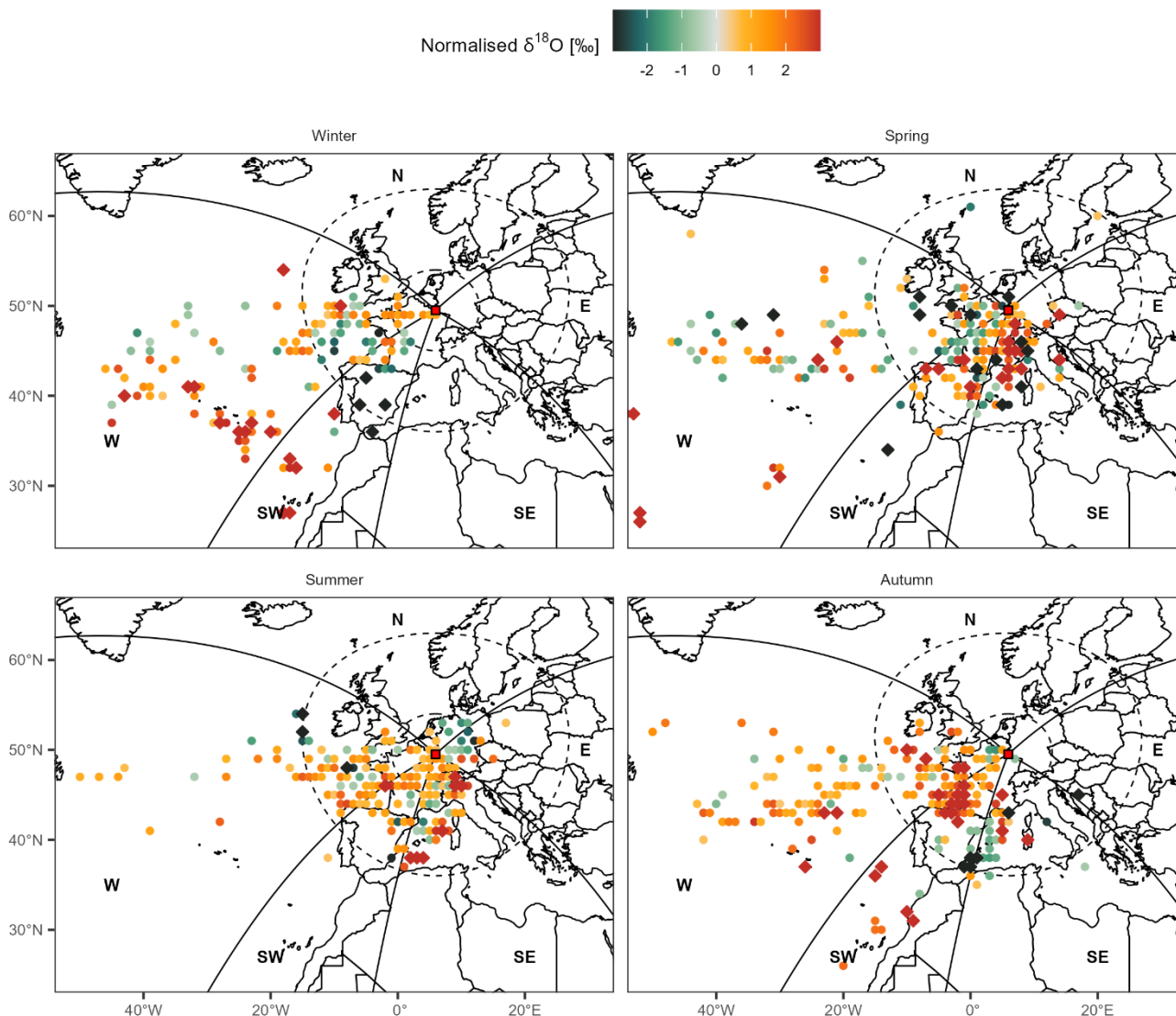
335 Figure 6: Maps of normalised precipitation \delta^{18}\text{O} values at the study site ( N = 847 ) based on the air moisture contributing areas (Fig. 3). Only moisture uptake locations contributing to more than 0.1 percent of the total seasonal uptake are shown. The colour of the points represents the mean (precipitation amount weighted) normalised precipitation \delta^{18}\text{O} (using 30-day running mean windows) of all trajectories carrying moisture from that specific location (i.e., cell of 1^\circ by 1^\circ raster). It is important to note that these are precipitation \delta^{18}\text{O} from the sampling site marked by a red square, not the \delta^{18}\text{O} at the moisture origin. Moisture uptake locations with normalised precipitation \delta^{18}\text{O} between -0.5 ‰ and 0.5 ‰ are not shown, while moisture uptake locations with normalised precipitation \delta^{18}\text{O} below -3.0 ‰ are marked with black diamonds and above 3.0 ‰ with red diamonds. 340
