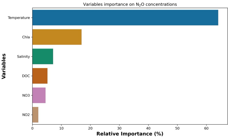
Figure 4: The relative importance of the leading environmental and biogeochemical variables driving the variability of nitrous oxide concentrations analyzed through cross-valued boosting (CVB). These are, in decreasing order, Temperature, Chlorophyll a (Chla), Salinity, Dissolved Organic Carbon (DOC), Nitrate (NO 3 ) and Nitrite (NO 2 ). The figure was developed using Python software version 3.12.3.
