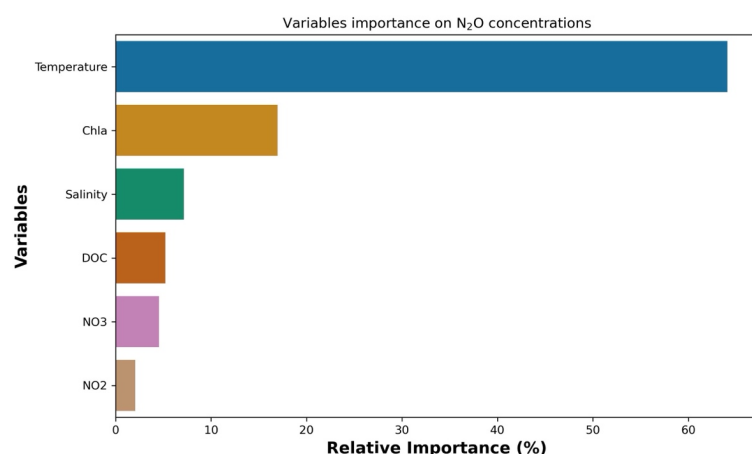
Figure 4: The relative importance of the leading environmental and biogeochemical variables driving the variability of nitrous oxide concentrations variability analyzed through cross-valued boosting (CVB). These are, in decreasing order, Temperature, Chlorophyll a (Chla), Salinity, Dissolved Organic Carbon (DOC), Nitrate (NO 3 ) and Nitrite (NO 2 ). The figure was developed using Python software version 3.12.3.
