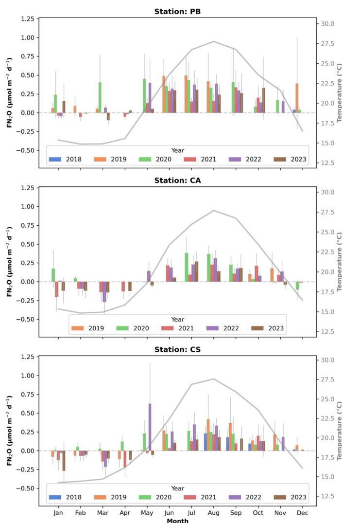
Figure 6: Box plot of monthly averaged values of air-sea Nitrous Oxide ( N_2O ) transfer ( FN_2O ) in \mu\text{mol m}^{-2} \text{d}^{-1} for all the study years (left axis) and averaged temperature ( ^{\circ}\text{C} ) values (right axis; grey line) for the PB (upper plot), CA (middle plot) and CS (lower plot) sites. Error bars represent \pm standard deviation. FN_2O significantly differs from 0, as evaluated by a t-test ( p>0.005 ). Figures were developed with the Python software version 3.12.3.
