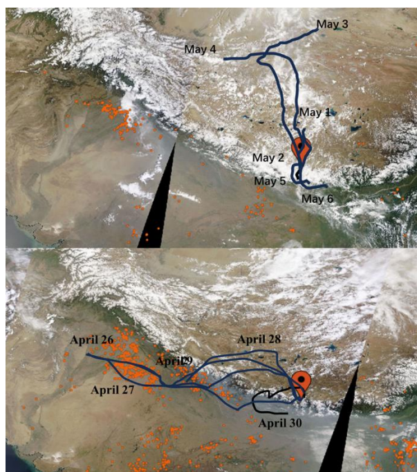
Figure 5. The modelled air-mass back trajectories during “Earth Summit Mission” scientific expedition in spring 2022 (a: from May 1 st to May 6 th ; b: April 26 th to April 30 th ). The active fire spots captured by MODIS ( https://worldview.earthdata.nasa.gov , the red dots in the figure) are also presented.
