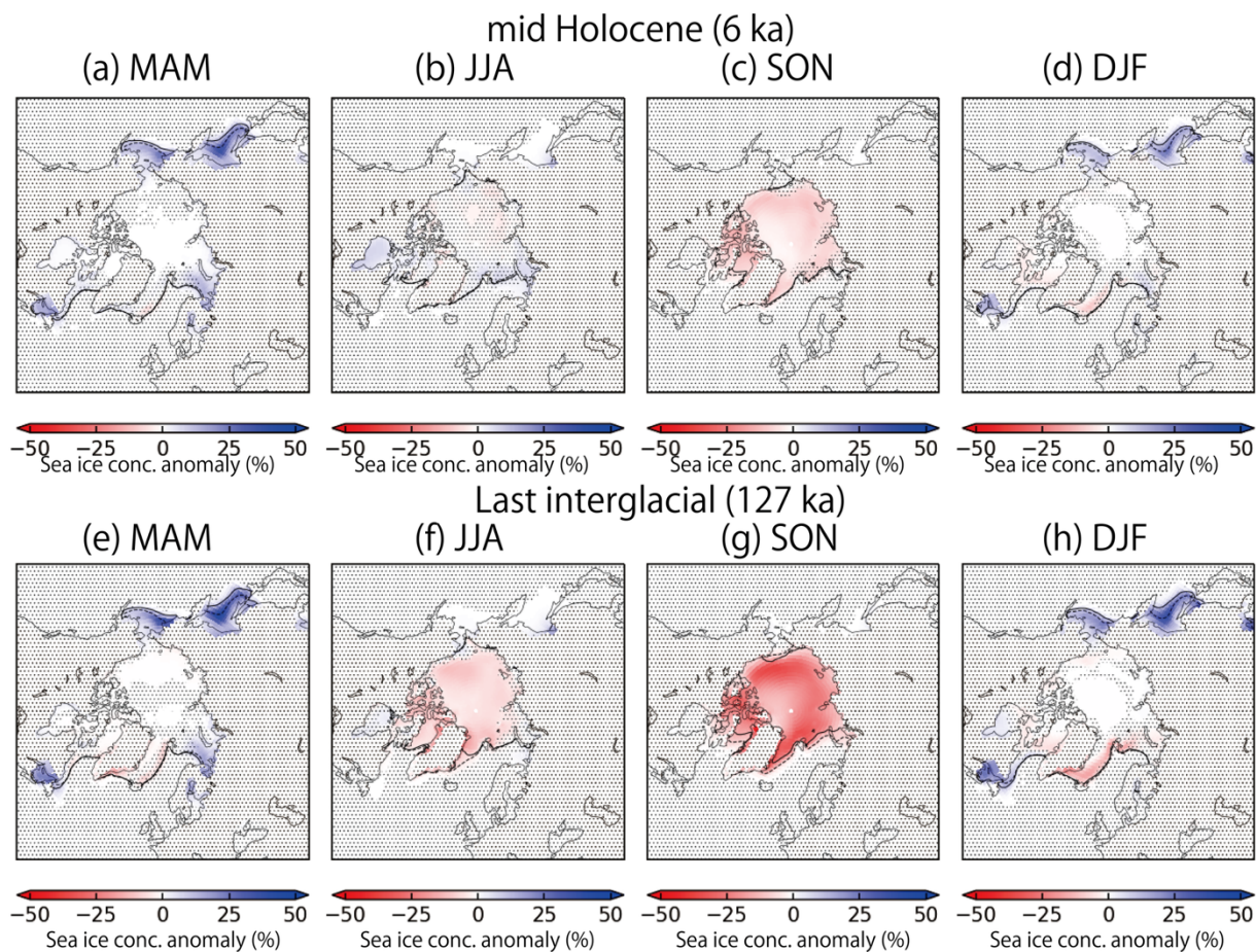
470 Figure A3: Sea ice concentration anomaly around the Arctic Ocean relative to the preindustrial condition for MAM, JJA, SON, and DJF during (a–d) the mid-Holocene (MH) ( MHcontrol-P_{lcontrol} ) and (e–h) the Last Interglacial (LIG) ( LIGcontrol-P_{lcontrol} ). The dotted area represents the region where 95% confidence interval was not achieved. The dashed line represents the boundary of the sea ice concentration of 15% for the P_{lcontrol} experiment. The solid line represents that for MHcontrol (upper panels) and LIGcontrol (lower panels) experiments, respectively.
