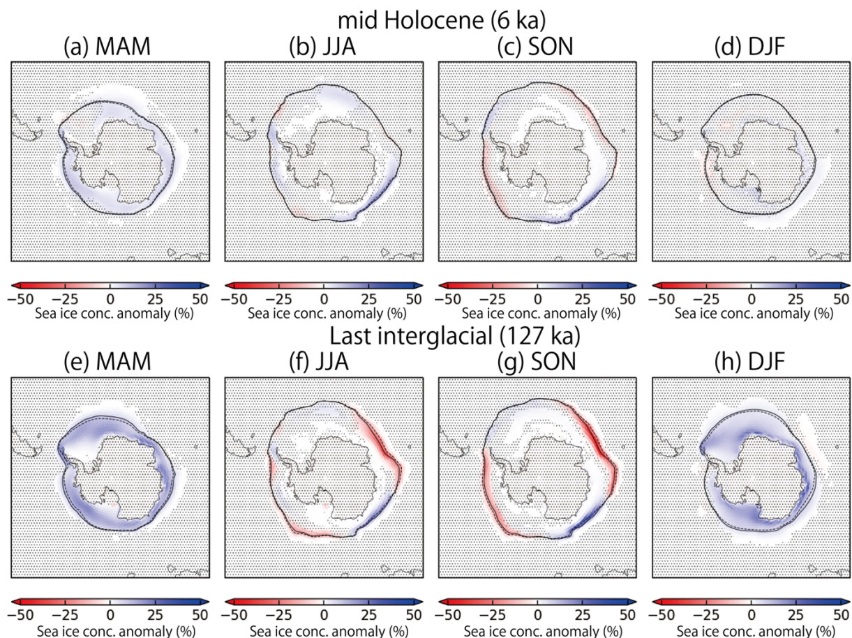
485 Figure A5: Sea ice concentration anomaly around the South Pole relative to the preindustrial condition for MAM, JJA, SON, and DJF during the mid-Holocene (MH) ( MH_{control}-PI_{control} ) (a–d) and the Last Interglacial (LIG) ( LIG_{control}-PI_{control} ) (e–h). The dotted area represents the region where 95% confidence interval was not achieved. The dashed line represents the boundary of the sea ice concentration of 15% for the PI_{control} experiment. The solid line represents that for MH_{control} (upper panels) and LIG_{control} (lower panels) experiments, respectively.
