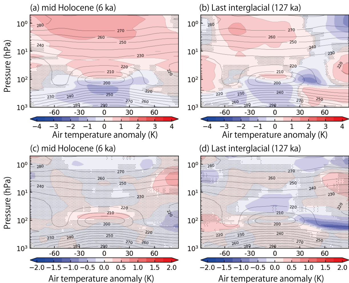
190 Figure 4: Zonal and annual mean air temperature anomaly relative to the preindustrial (PI) condition in the (a) MH ( MHcontrol – PIcontrol ) and (b) LIG ( LIGcontrol – PIcontrol ). Zonal and annual mean ozone-induced air temperature anomaly relative to the preindustrial (PI) condition in the (c) MH ( MHcontrol – PIcontrol – MHnoChem + PInoChem ) and (d) LIG ( LIGcontrol – PIcontrol – LIGnoChem + PInoChem ). The contour represents the zonal and annual mean ozone concentration in the MH and LIG, respectively. The dotted area represents the region where 95% confidence interval was not achieved.
