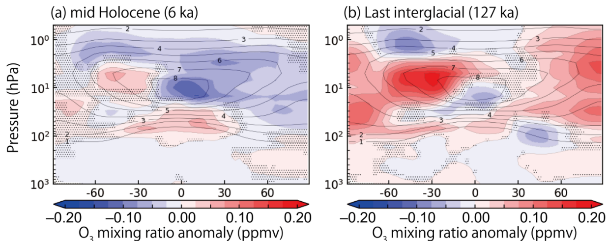
Figure 2: Zonal and annual mean ozone anomaly relative to the preindustrial (PI) condition in the (a) MH ( MH_{control}-PI_{control} ) and (b) LIG ( LIG_{control}-PI_{control} ). The contour represents the zonal and annual mean ozone concentration in the MH and LIG, respectively. The dotted area represents the region where 95% confidence interval was not achieved.
