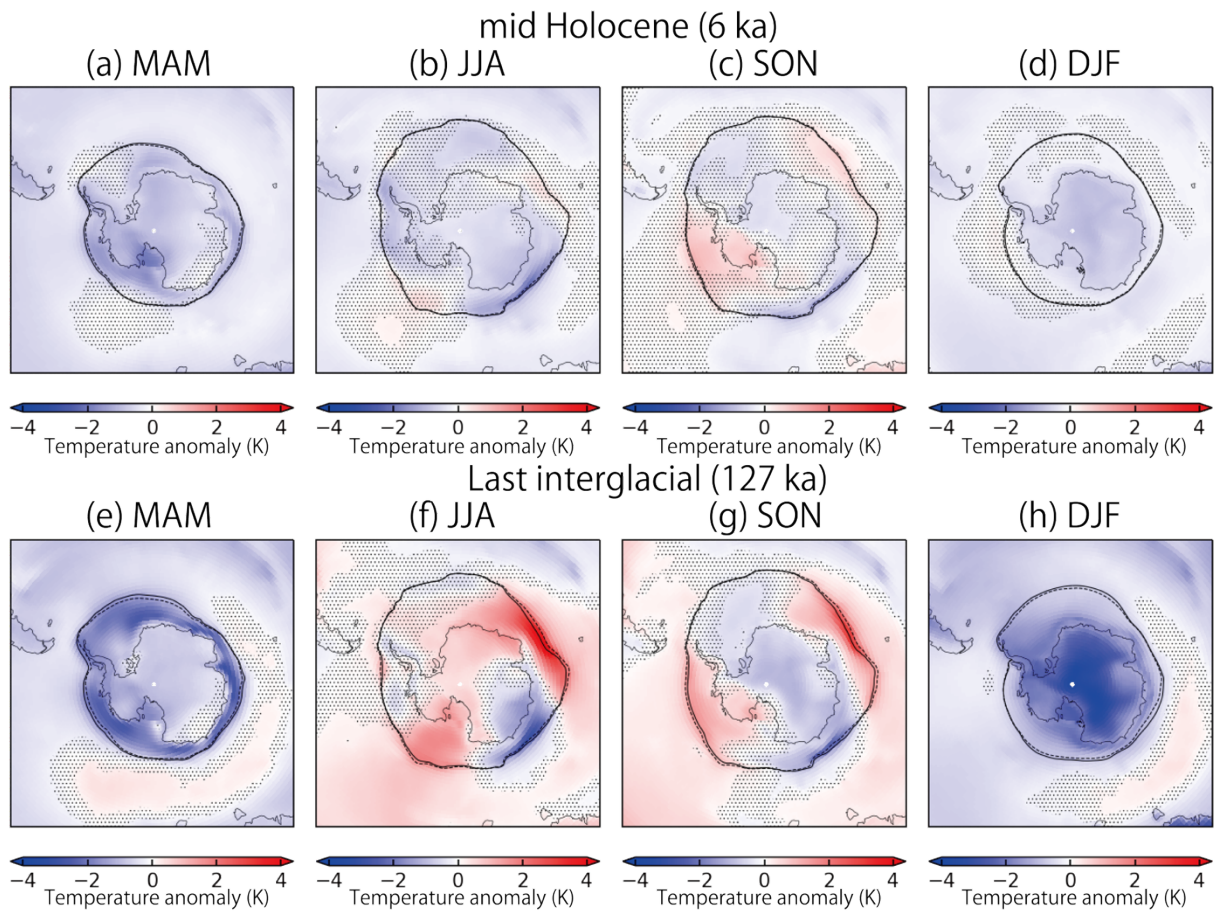
Figure 10: Surface air temperature anomaly around the South Pole relative to the preindustrial condition for MAM, JJA, SON, and DJF during the mid-Holocene (MH) ( MHcontrol - Pcontrol ) (a–d) and the Last Interglacial (LIG) ( LIGcontrol - Pcontrol ) (e–h). The dotted area represents the region where 95% confidence interval was not achieved. The dashed line represents the boundary of the sea ice concentration of 15% for the Pcontrol experiment. The solid line represents that for MHcontrol (upper panels) and LIGcontrol (lower panels) experiments, respectively.
