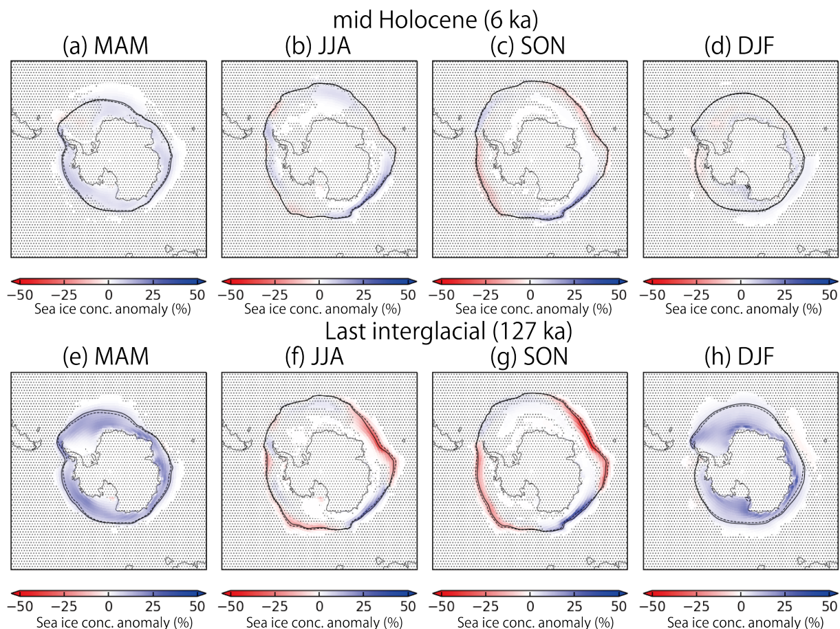
Figure A5: Sea ice concentration anomaly around the South Pole relative to the preindustrial condition for MAM, JJA, SON, and DJF during the mid-Holocene (MH) ( MHcontrol-P_{Icontrol} ) (a–d) and the Last Interglacial (LIG) ( LIGcontrol-P_{Icontrol} ) (e–h). The dotted area represents the region where 95% confidence interval was not achieved. The dashed line represents the boundary of the sea ice concentration of 15% for the P_{Icontrol} experiment. The solid line represents that for MHcontrol (upper panels) and LIGcontrol (lower panels) experiments, respectively.
