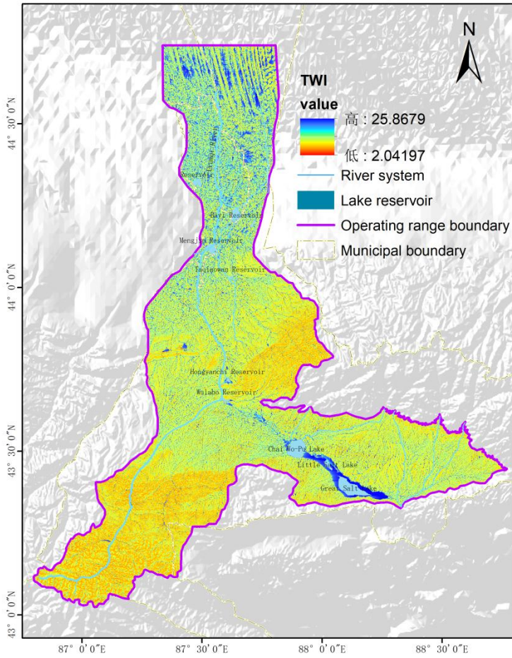
Figure S5: Distribution of TWI in Urumqi River and Chai Wo-pu Basin
