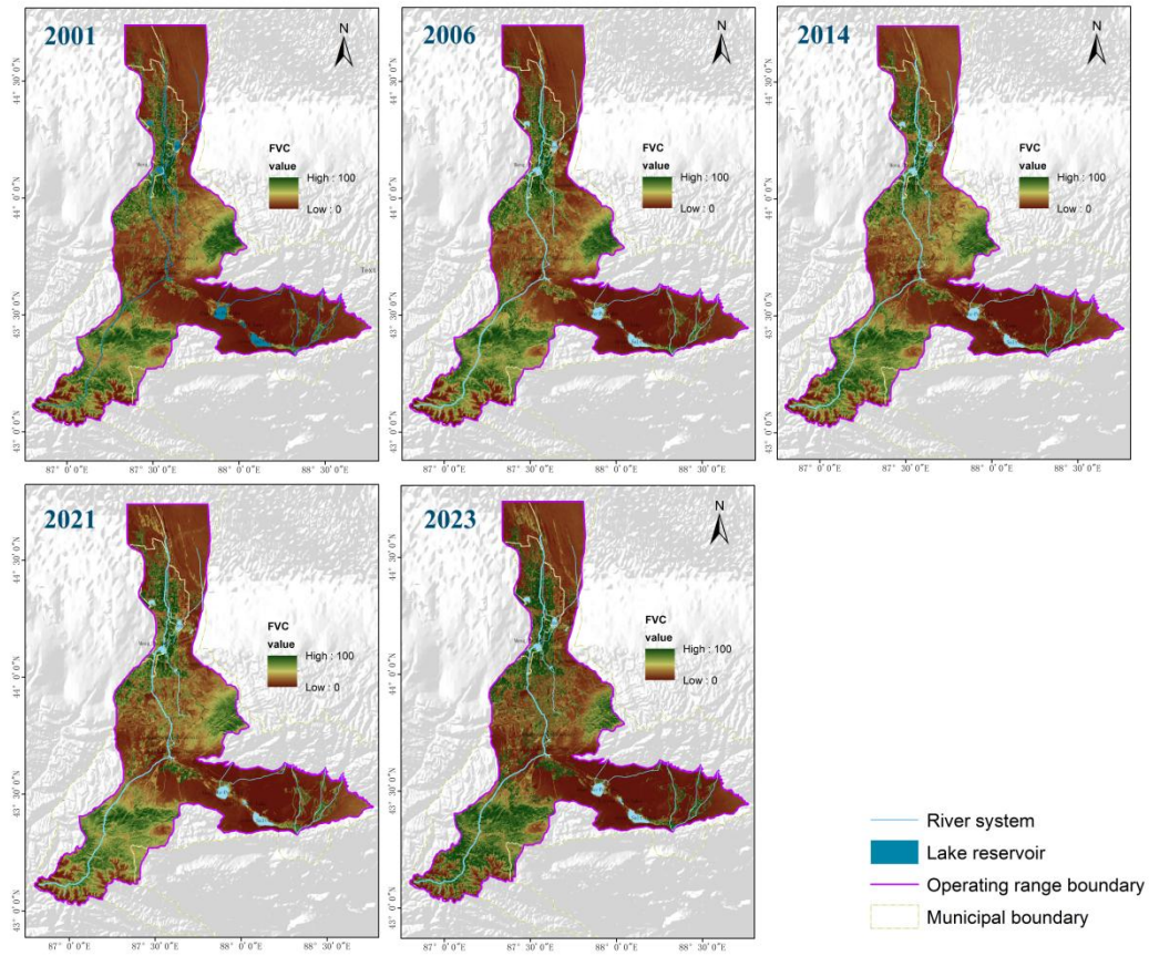
Figure S3: Distribution of FVC in Urumqi River and Chai Wo-pu Basin
