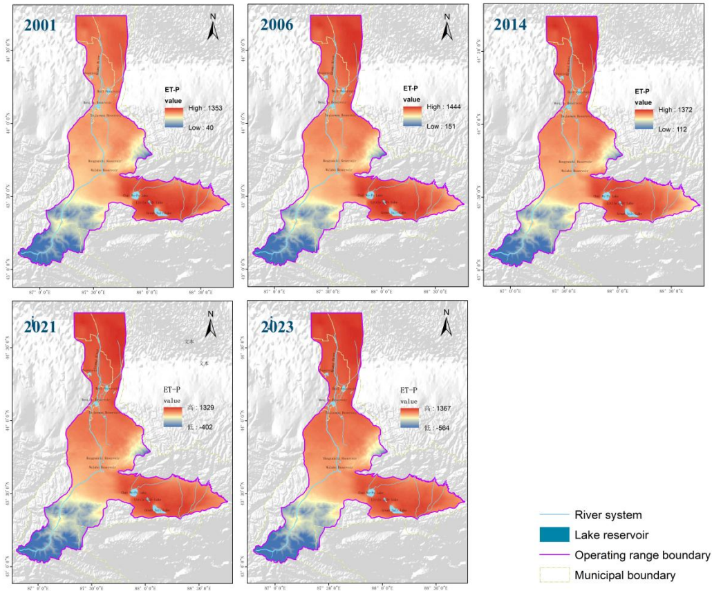
Figure S4: Distribution of E-P in Urumqi River and Chai Wo-pu Basin
