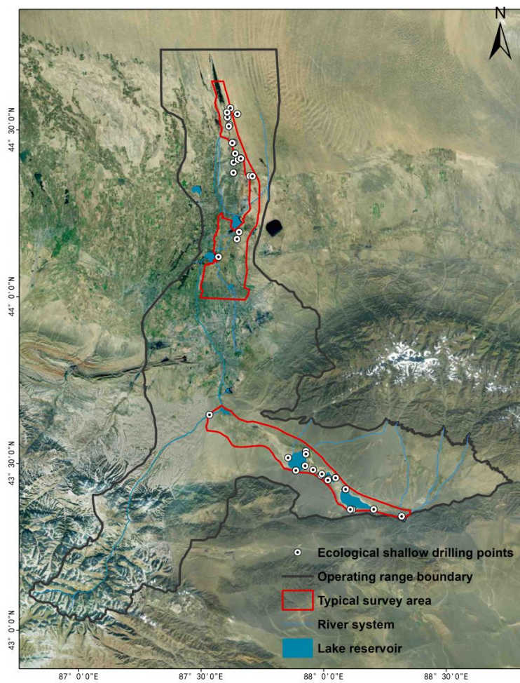
Figure S1: Ecological shallow drilling points
