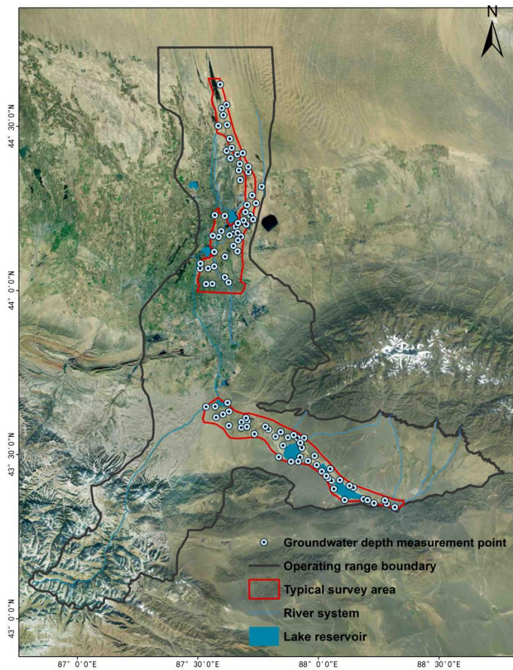
Figure S2: Groundwater depth measurement location distribution
