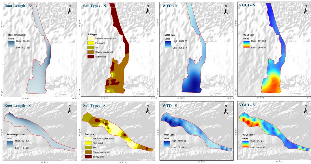
Figure S6: Distribution of Vegetation Groundwater Uptake Index in the GDEs Typical Areas of the Urumqi River and Chai Wo-pu Basin
