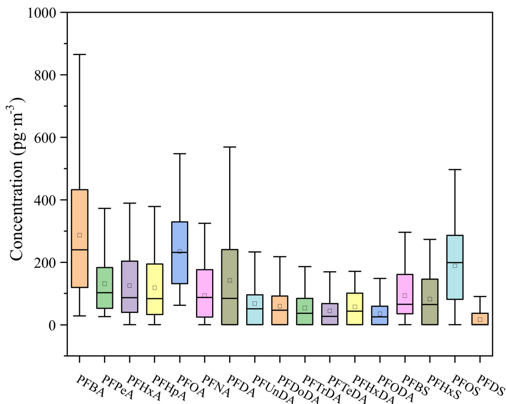
Fig. 1. Box diagram of 17 PFAA concentrations in PM 2.5 across four seasons
