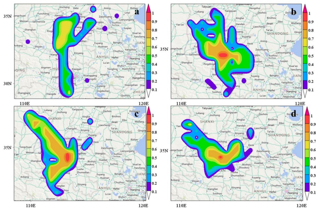
Fig. 4. Map of potential source analysis of PM 2.5 -bound PFAAs in Zhengzhou City in four seasons (a, b, c and d are spring, summer, fall and winter respectively, created by MeteoinfoMap 3.5.11 (Wang, 2014; Wang, 2019)). © Microsoft. The software is open.
